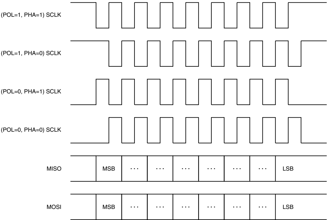
Figure 20-3. ECSPI SCLK, MISO, and MOSI Relationship
