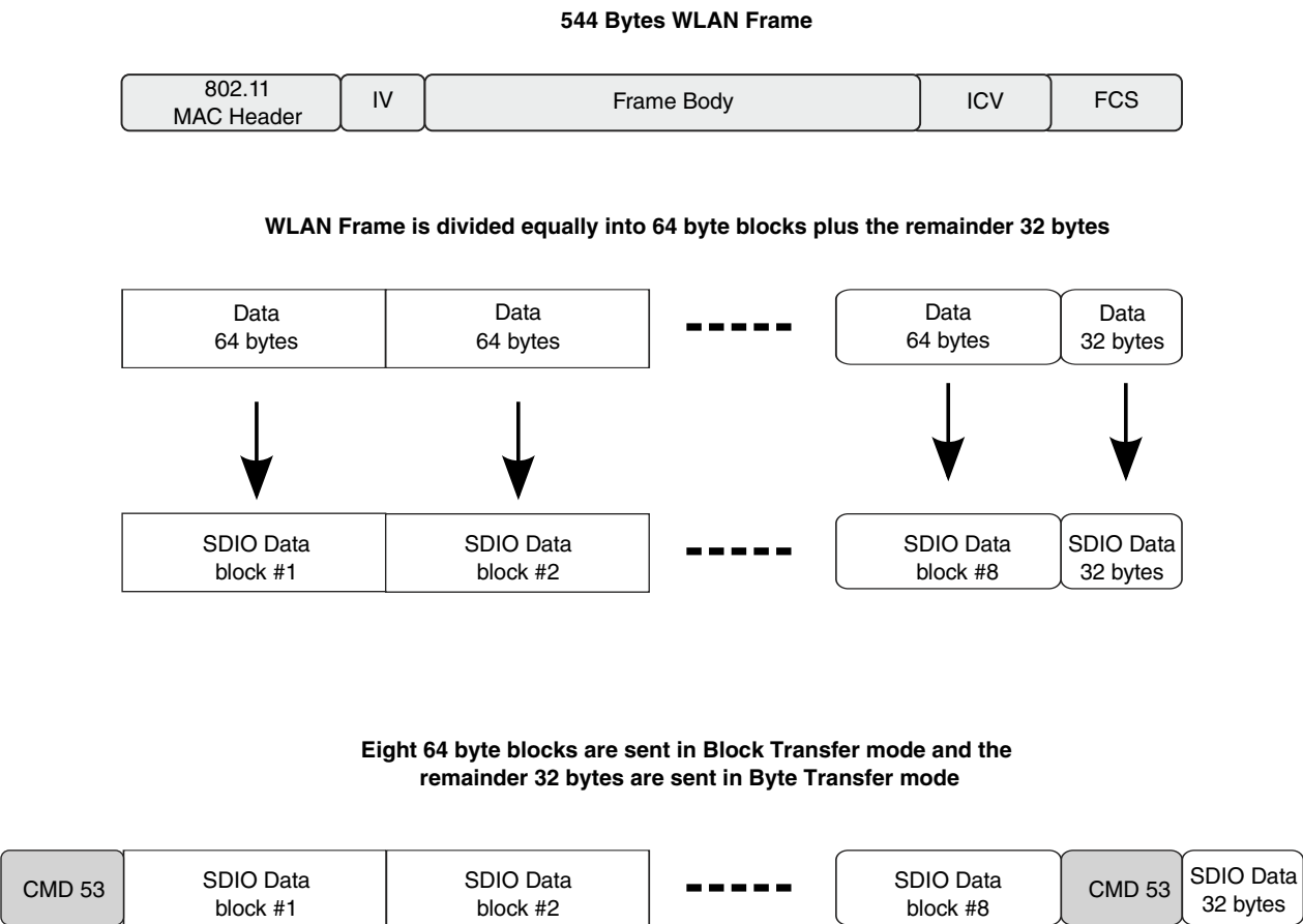
Figure 58-6. Example for Dividing Large Data Transfers
