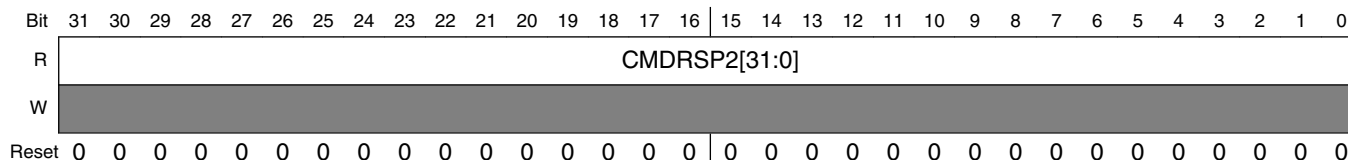
uSDHCx_CMD_RSP2 field descriptions
