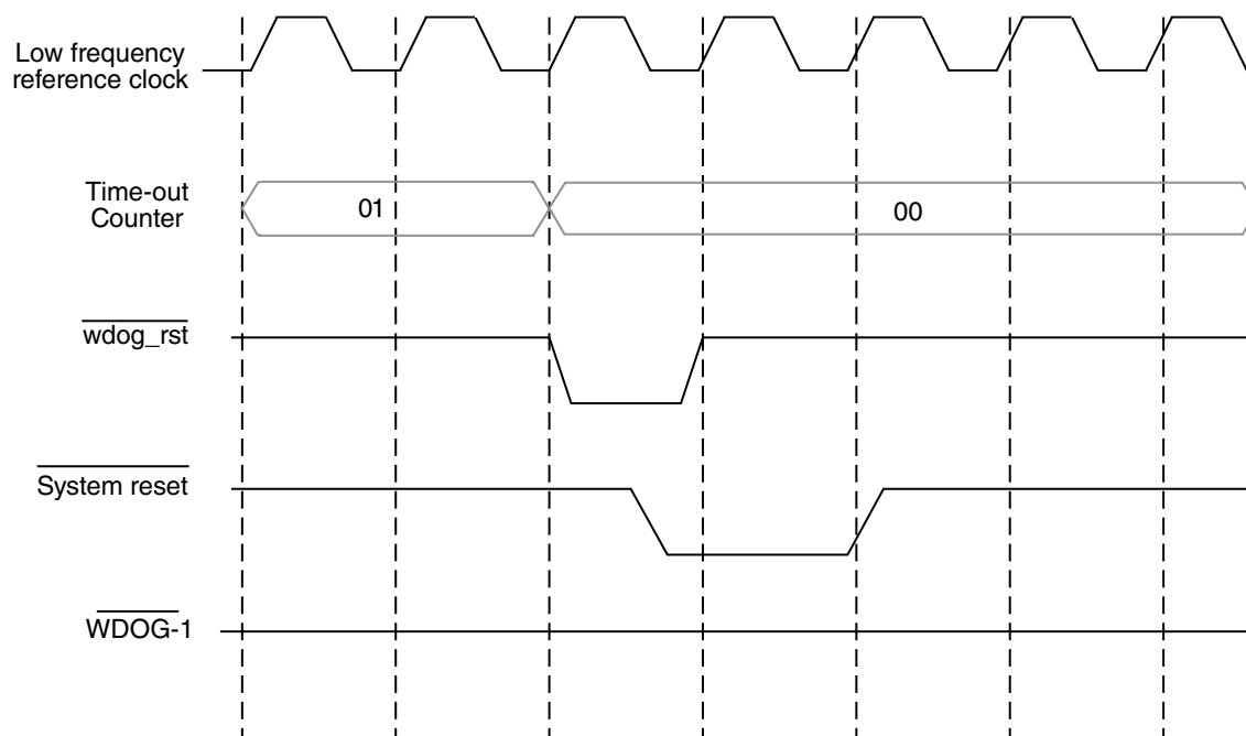
Figure 59-4. WDOG timeout condition/WDT bit is not set
