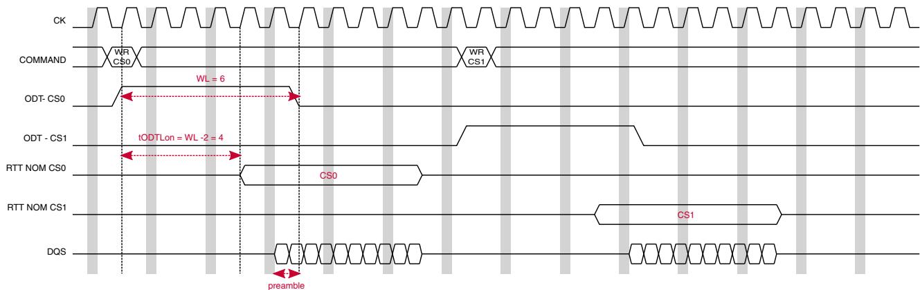
Figure 35-7. ODT - Timing Diagram DDR3 WL=6, BL=8
