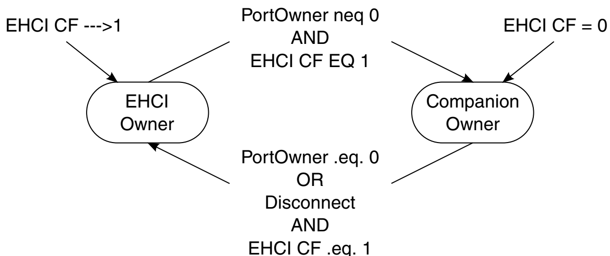
Figure 56-5. Port Owner Handoff State Machine
