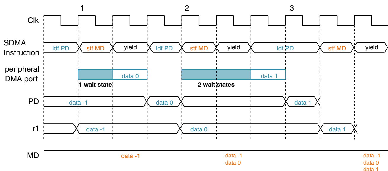
Figure 46-21. Peripheral to External Memory Example (1)
