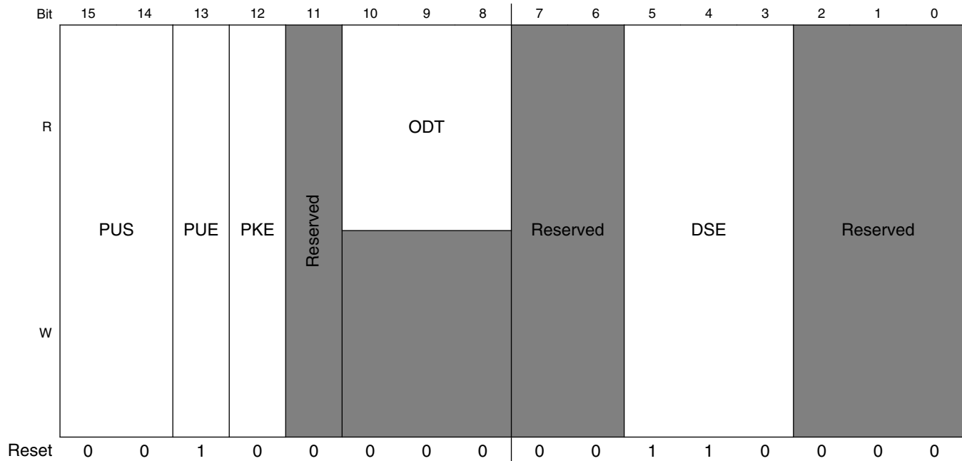
IOMUXC_SW_PAD_CTL_PAD_DRAM_SDQS1_P field descriptions
