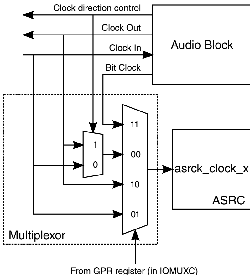
Figure 9-3. Muxing scheme template for ASRC input clocks
