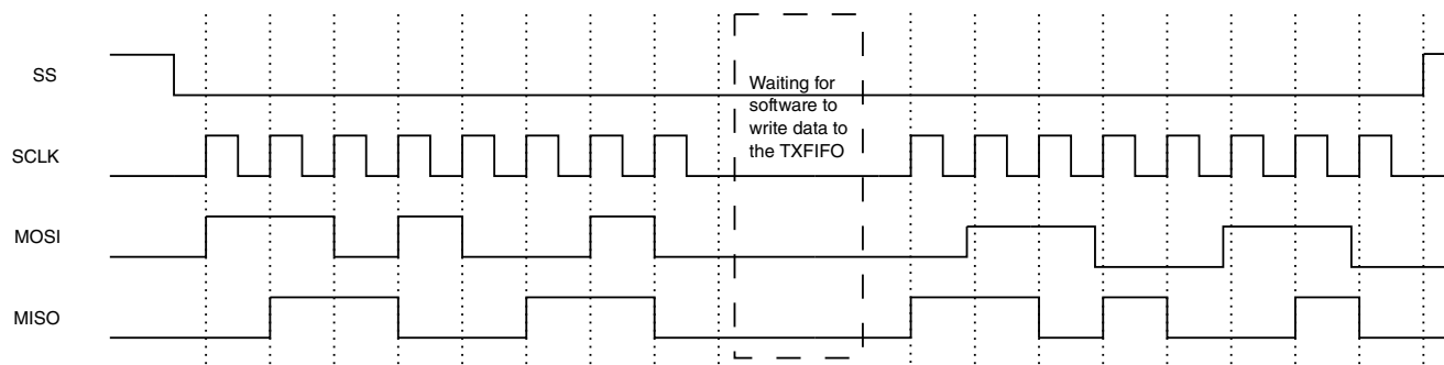
Figure 20-8. SPI Burst While SS_CTL[3:0] is Clear
