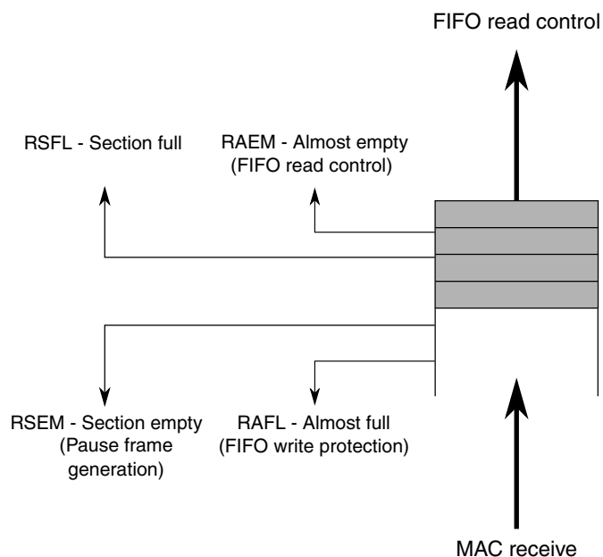
Figure 22-11. Receive FIFO overview
