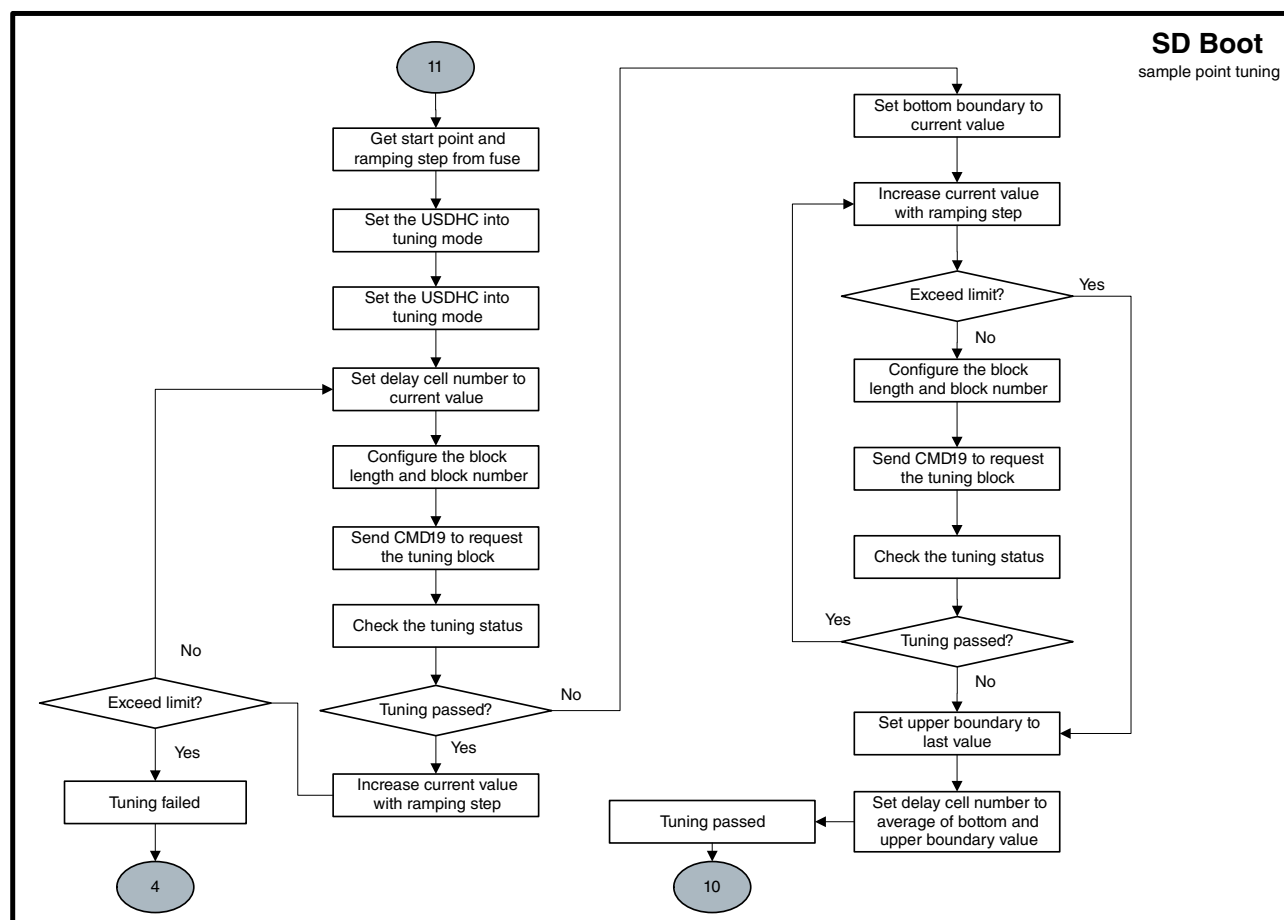
Figure 8-17. Expansion device boot flow (6 of 6) i.MX 6ULL Applications Processor Reference Manual, Rev. 1, 11/2017
