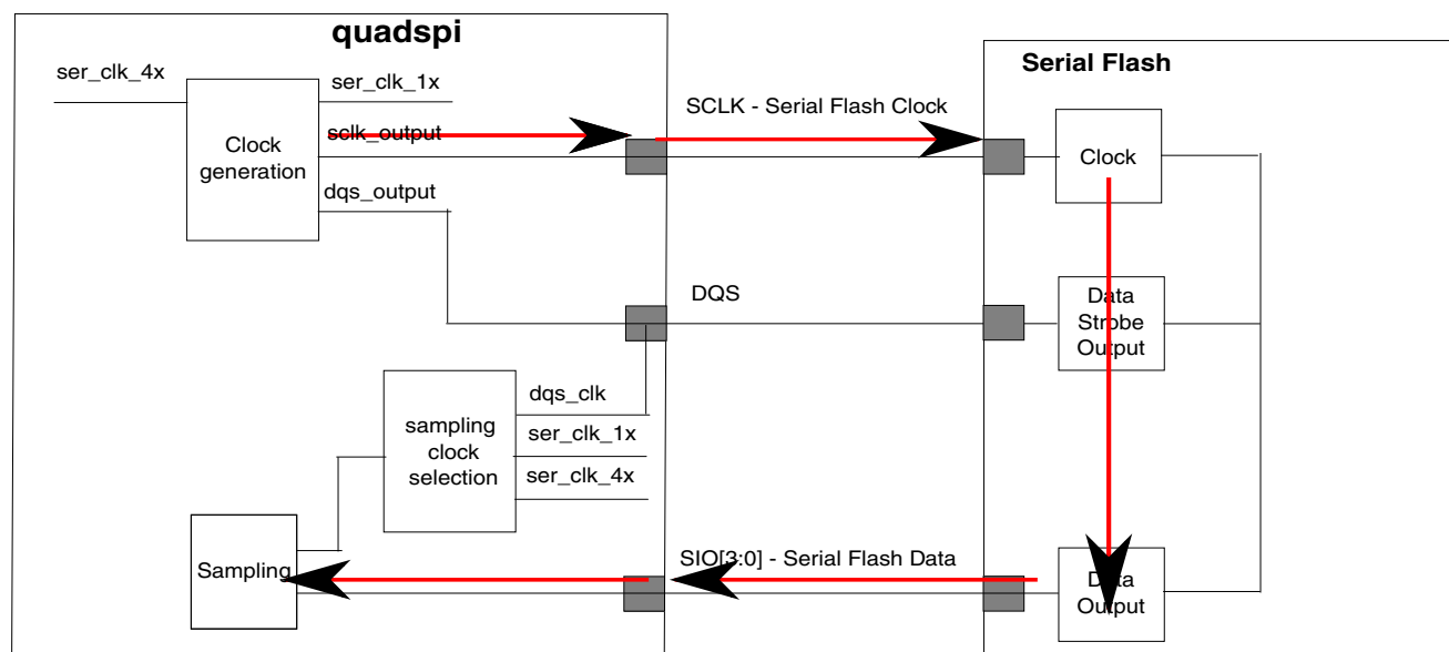
Figure 42-12. Serial flash data and clock path
