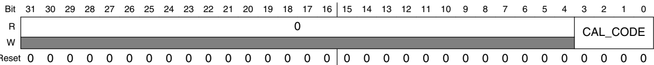
ADCx_CAL field descriptions
