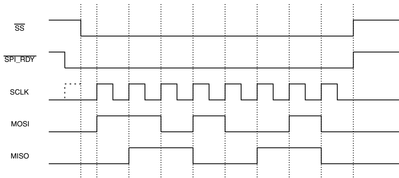
Figure 20-6. Relationship Between a SPI Burst and SPI_RDY: Low-Level Triggered
