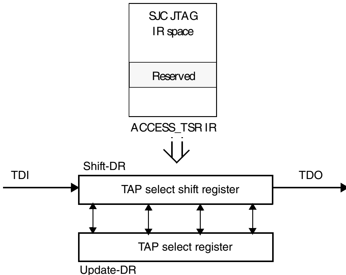
Figure 47-10. Using Reserved IR to Access the TAP Select Register (SJC_TSR)
