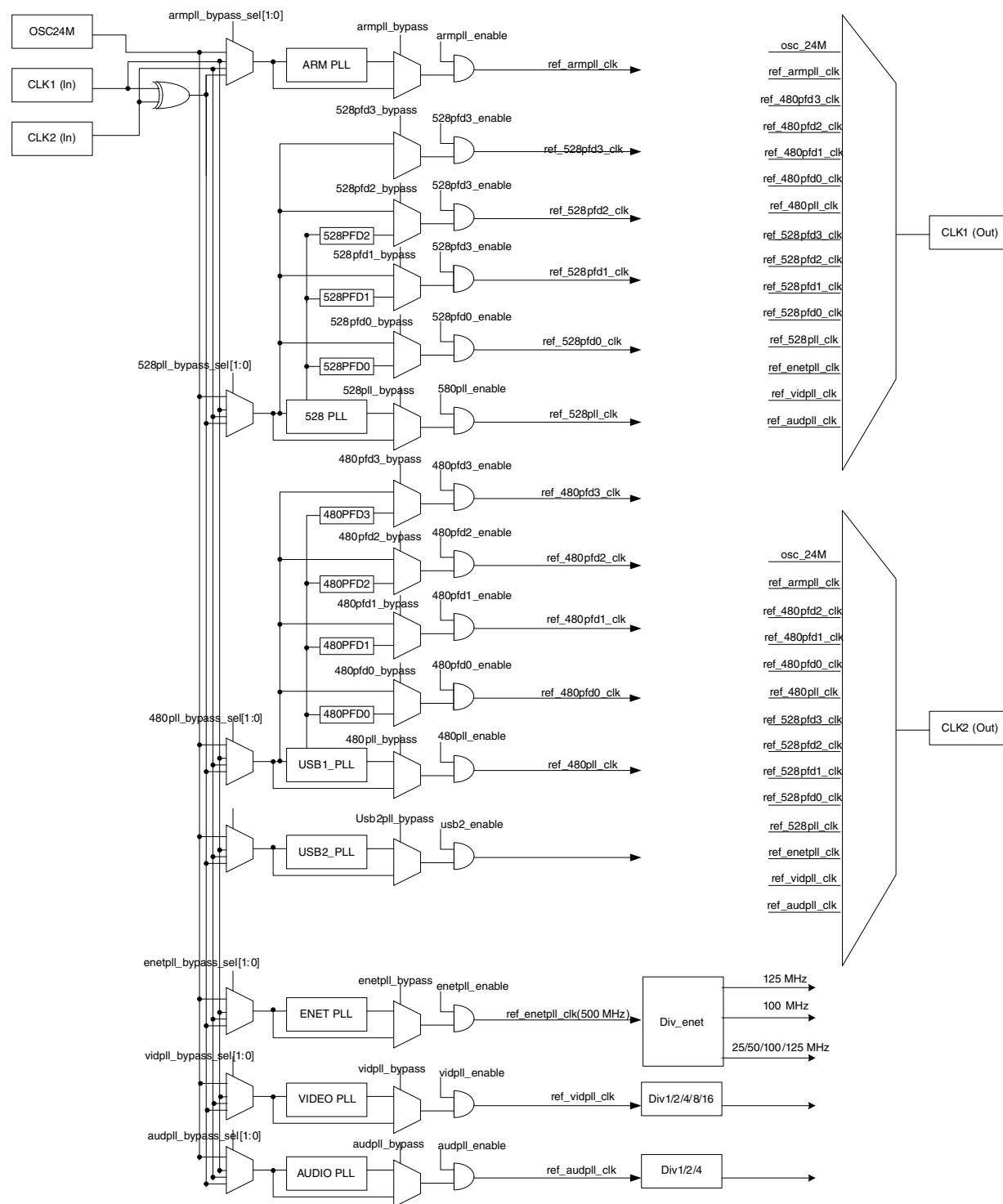
Figure 10-3. Primary Clock Generation
