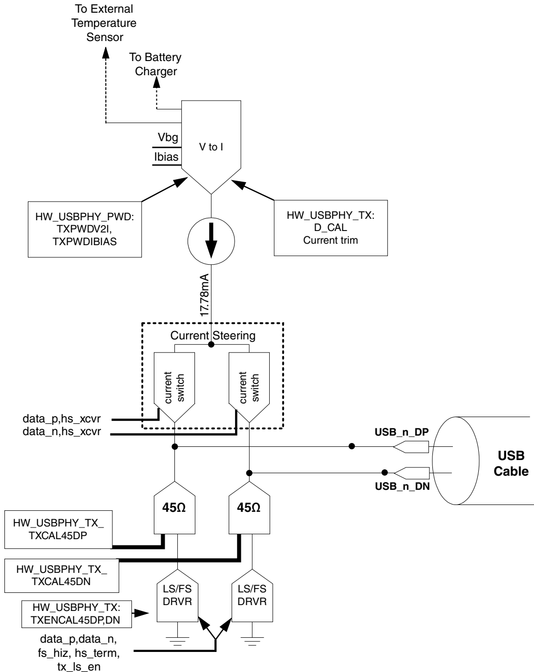
Figure 57-2. USB 2.0 PHY Transmitter Block Diagram
