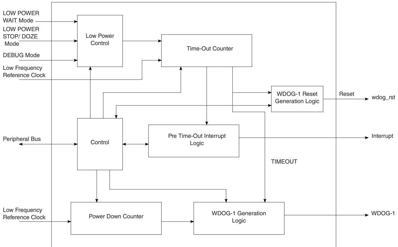
Figure 59-1. WDOG Diagram
