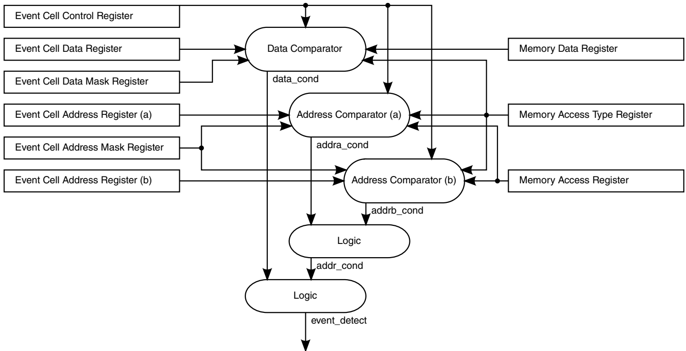
Figure 46-14. Event Cell Architecture
