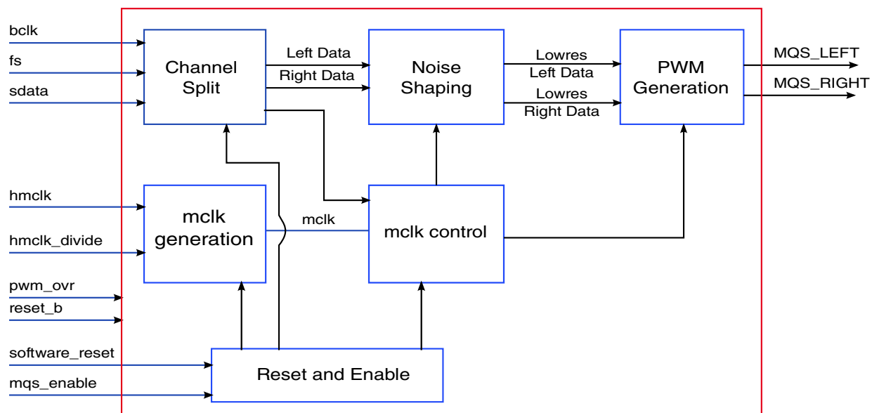
Figure 36-1. Block Diagram
