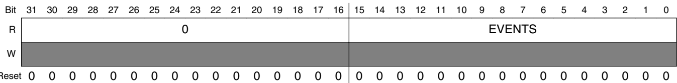
SDMACORE_EVENTS2 field descriptions
