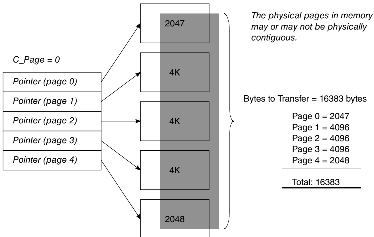
Figure 56-18. Example Mapping of qTD Buffer Pointers to Buffer Pages
