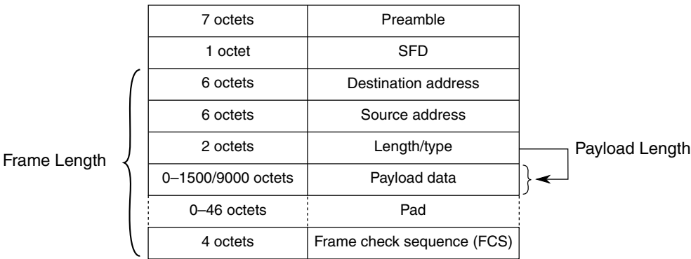
Figure 22-2. MAC frame format overview
