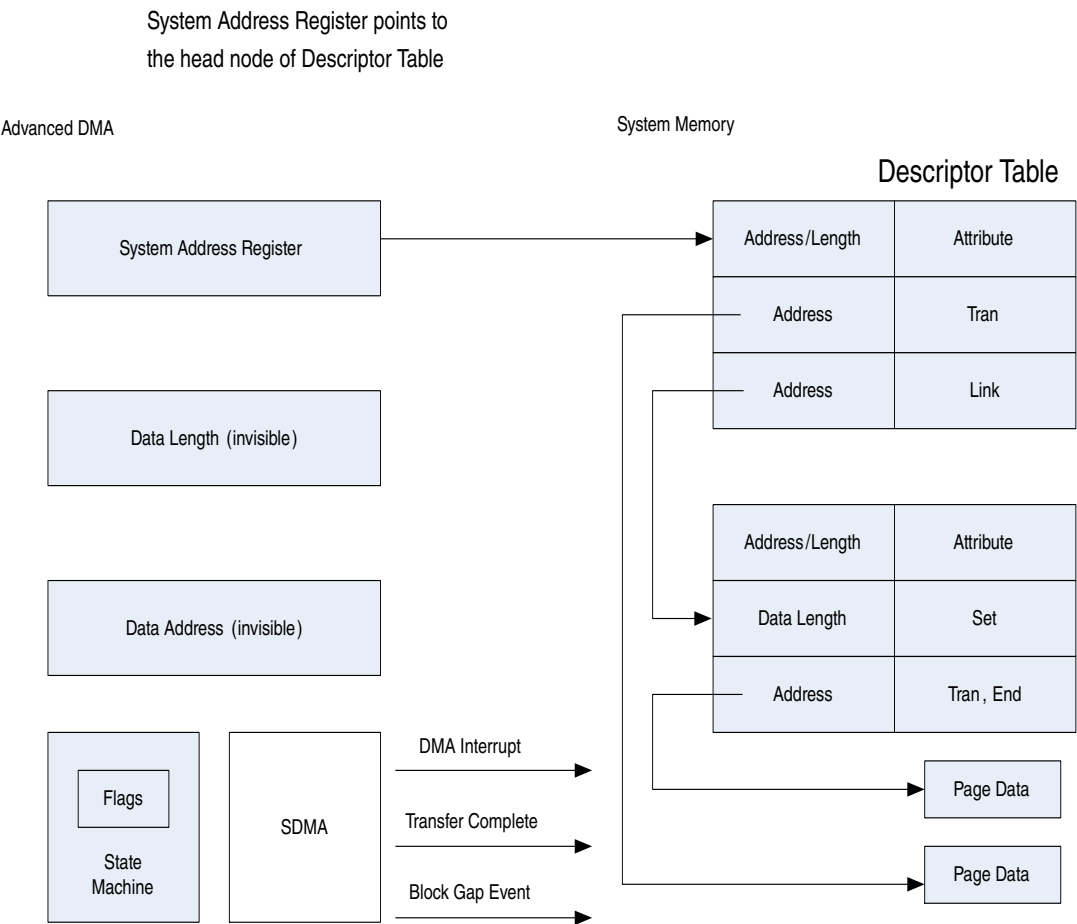
Figure 58-9. Concept and Access Method of ADMA1 Descriptor Table
