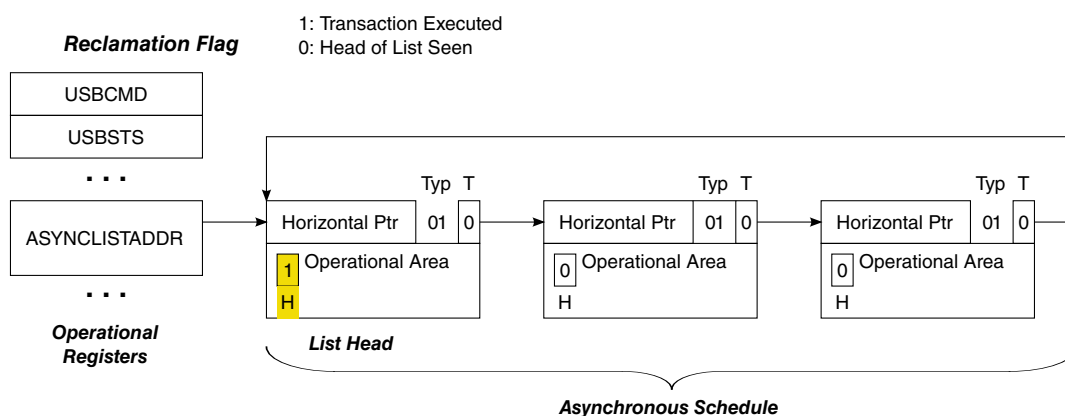
Figure 56-14. Asynchronous Schedule List w/Annotation to Mark Head of List
