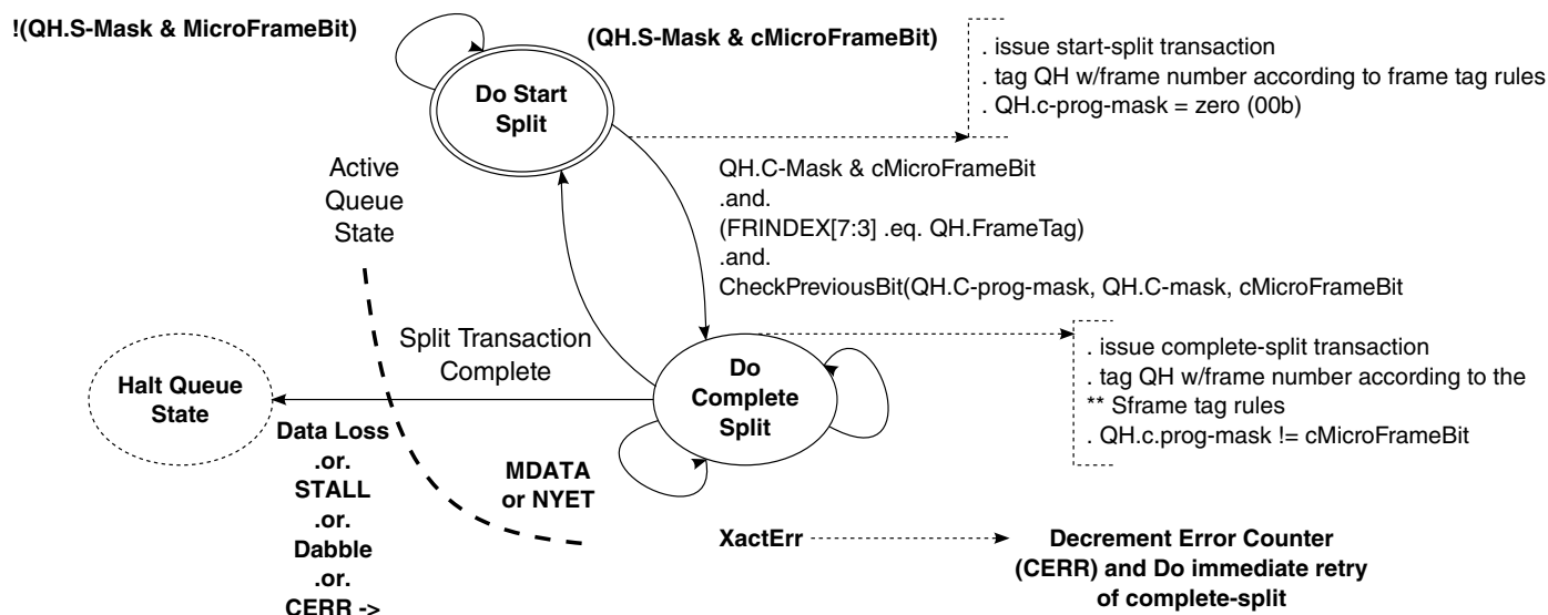
Figure 56-23. Split Transaction State Machine for Interrupt
