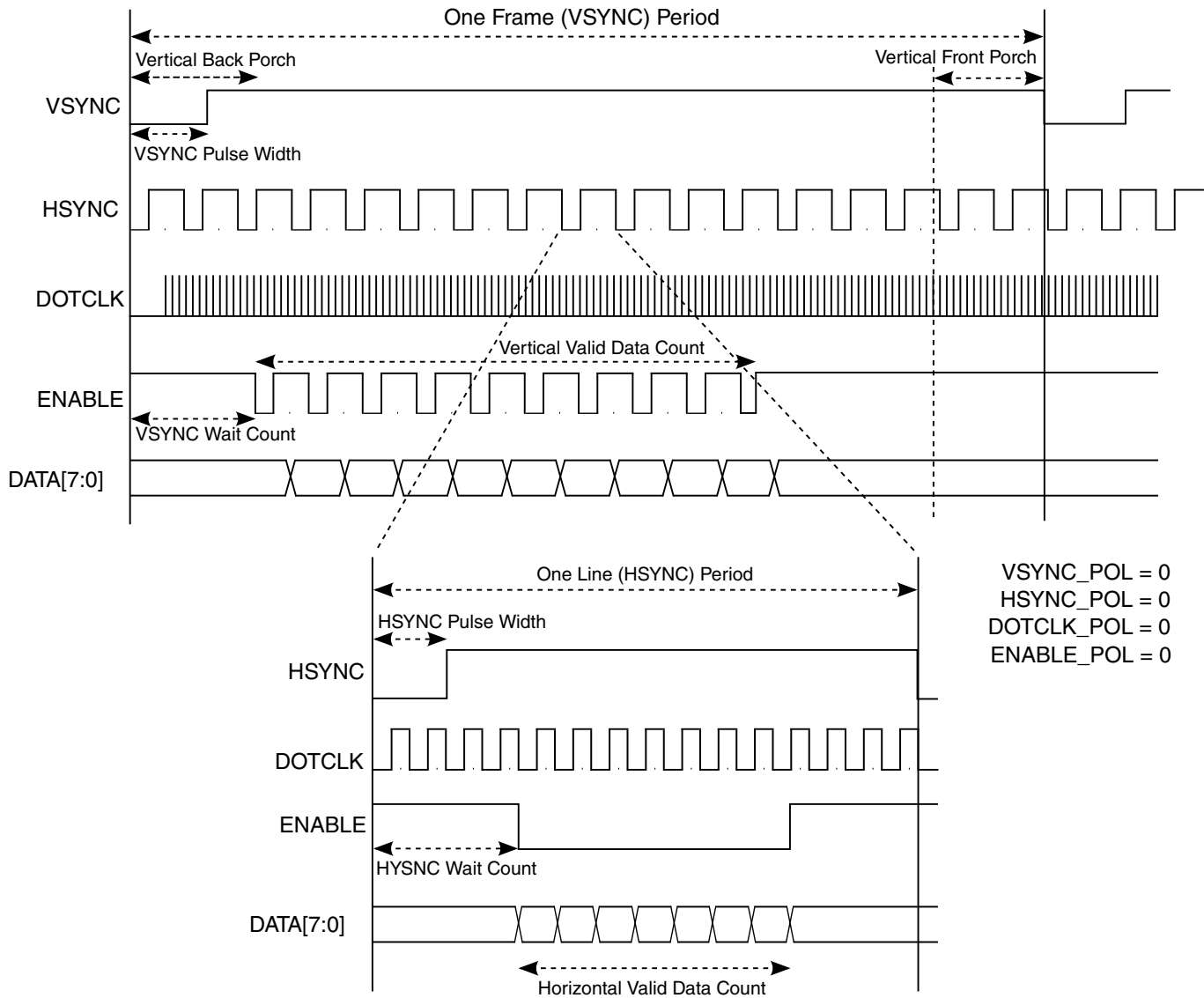
Figure 34-13. DOTCLK protocol with programmable parameters
