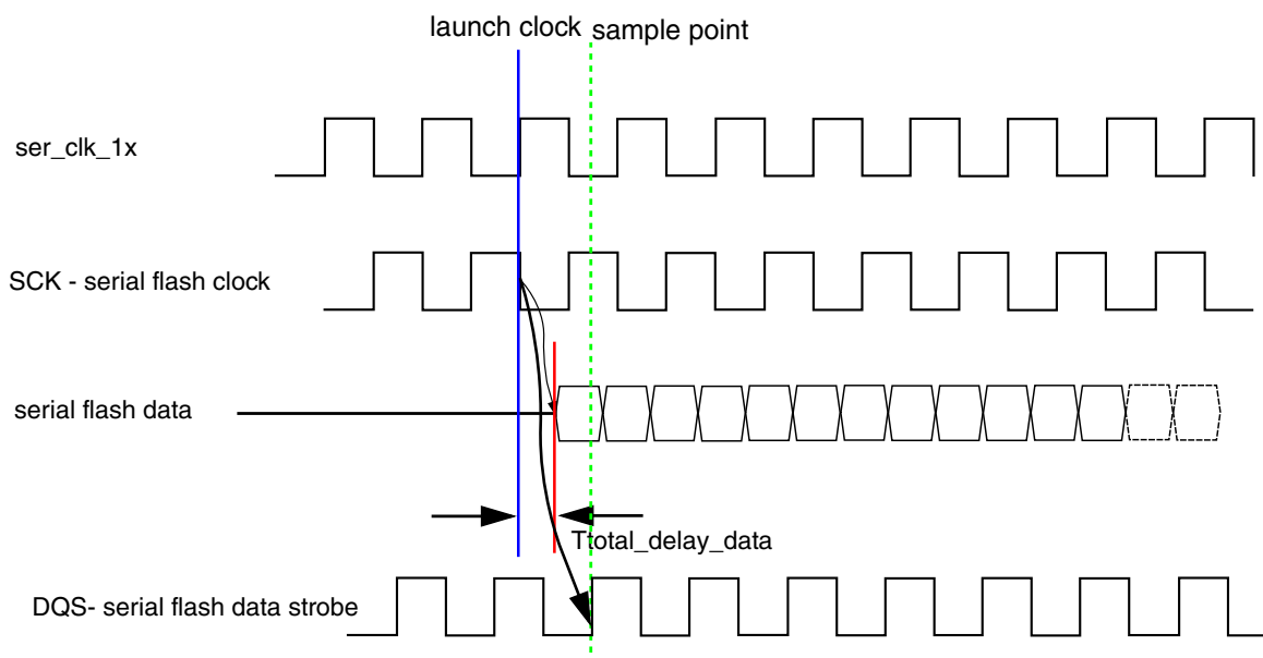
Figure 42-17. Input timing in DDR mode with flash DQS sampling
