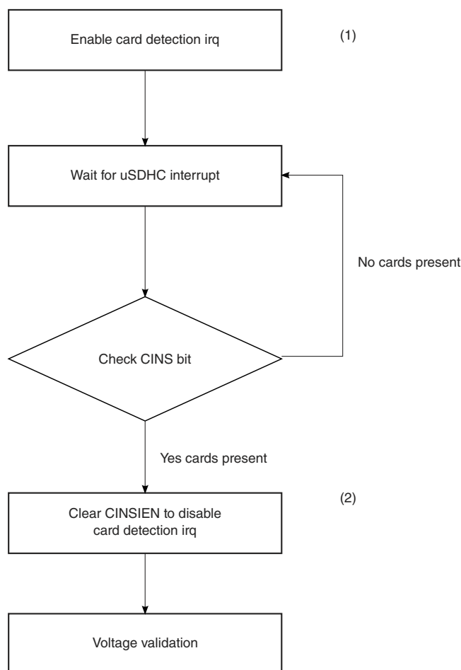
Figure 58-18. Flow Diagram for Card Detection
