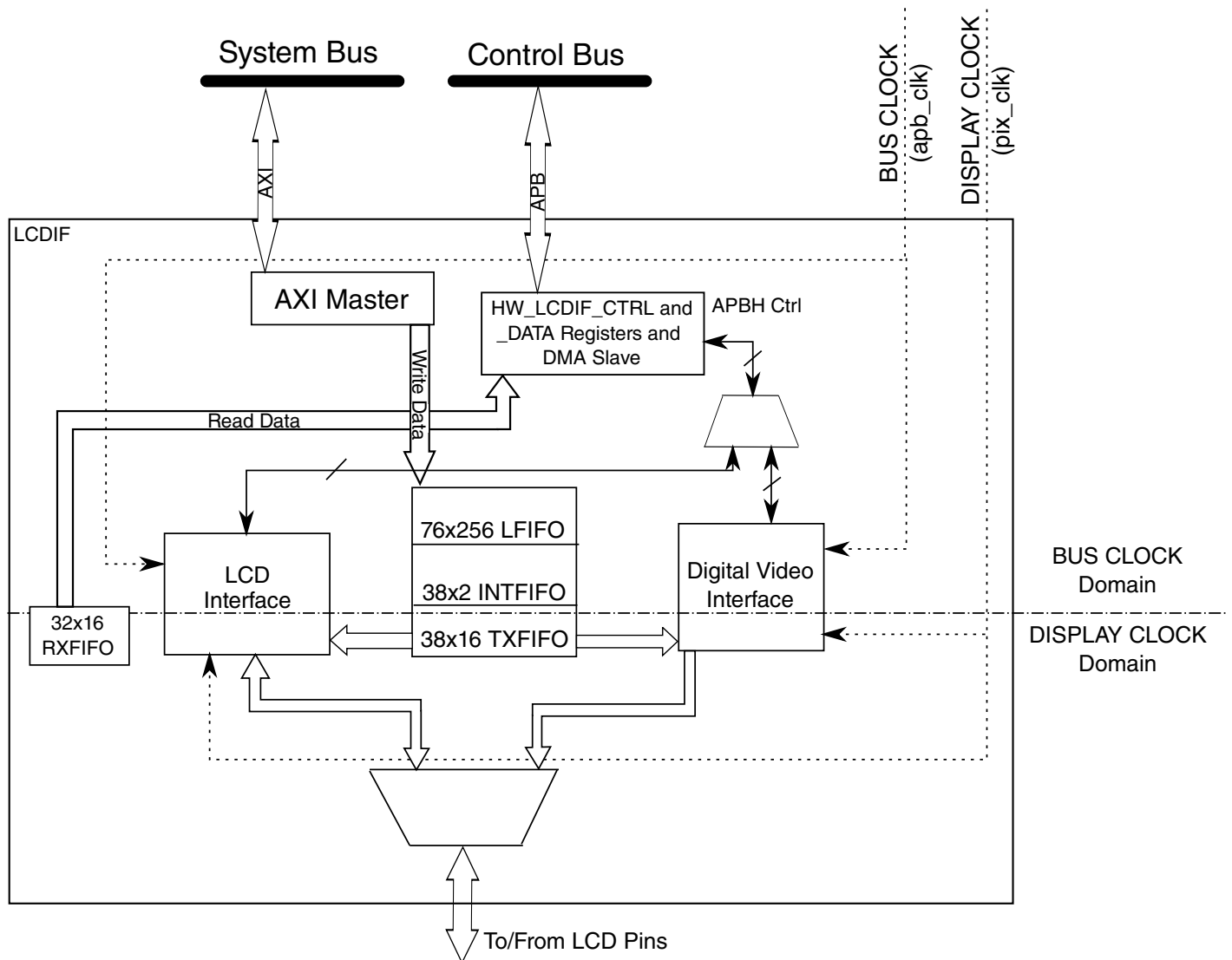
Figure 34-1. Top-Level Block Diagram of eLCDIF subsystem
