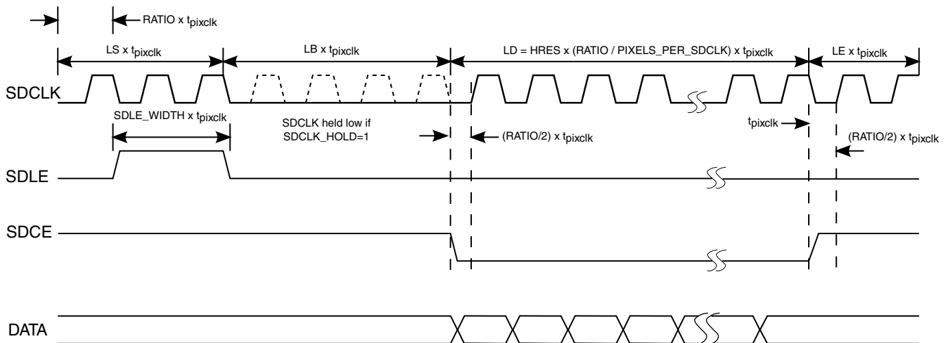
Figure 23-3. Line Timing ( \text{DDR\_MODE} = 0 )
