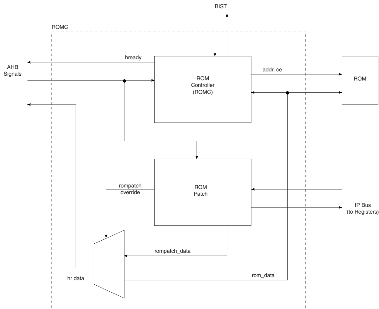
Figure 43-1. ROMC Block Diagram
