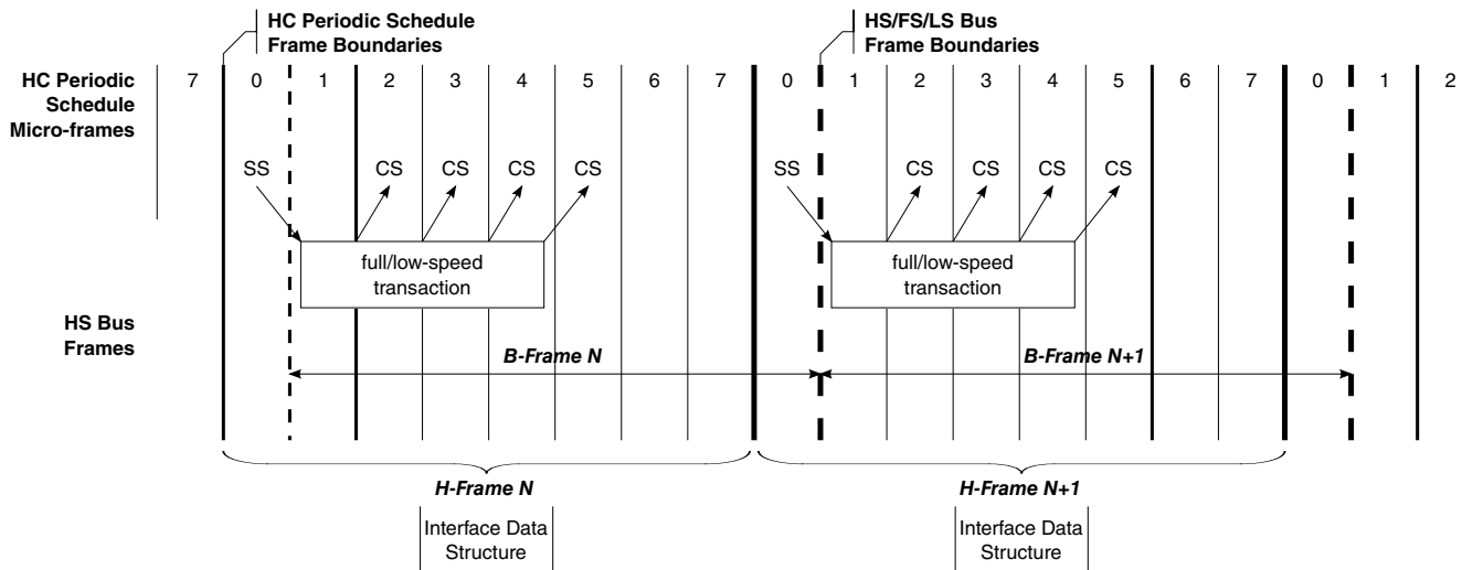
Figure 56-10. Relationship of Periodic Schedule Frame Boundaries to Bus Frame Boundaries
