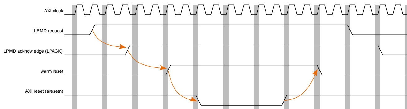
Figure 35-5. Warm Reset Diagram
