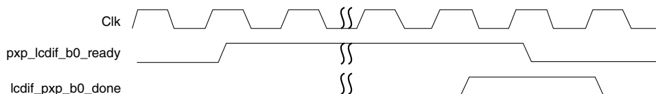
Figure 41-18. Buffer Sharing Protocol
