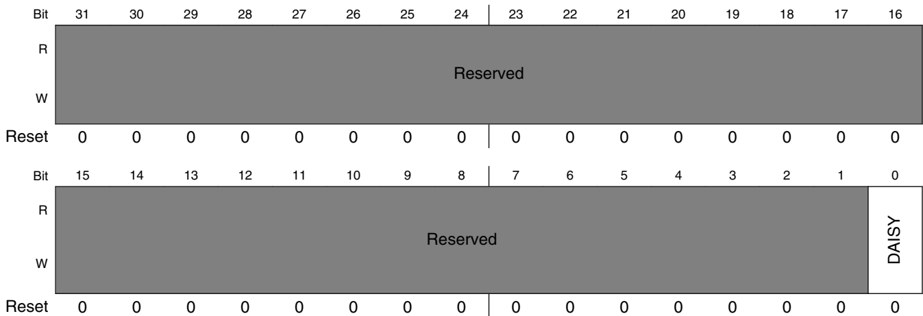
IOMUXC_CSI_DATA14_SELECT_INPUT field descriptions
