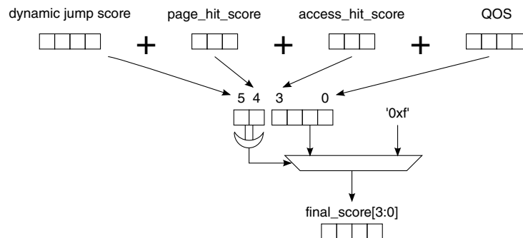
Figure 35-6. Dynamic score/priority calculation
