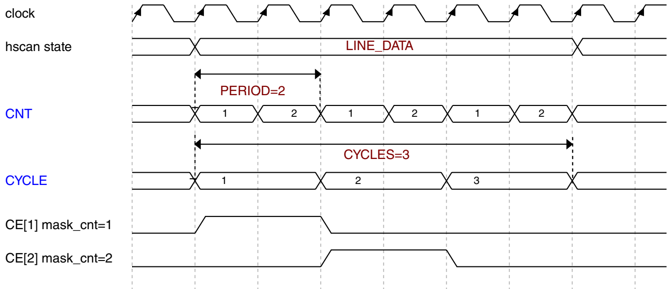
Figure 23-7. Definition of CNT, CYCLE, PERIOD
