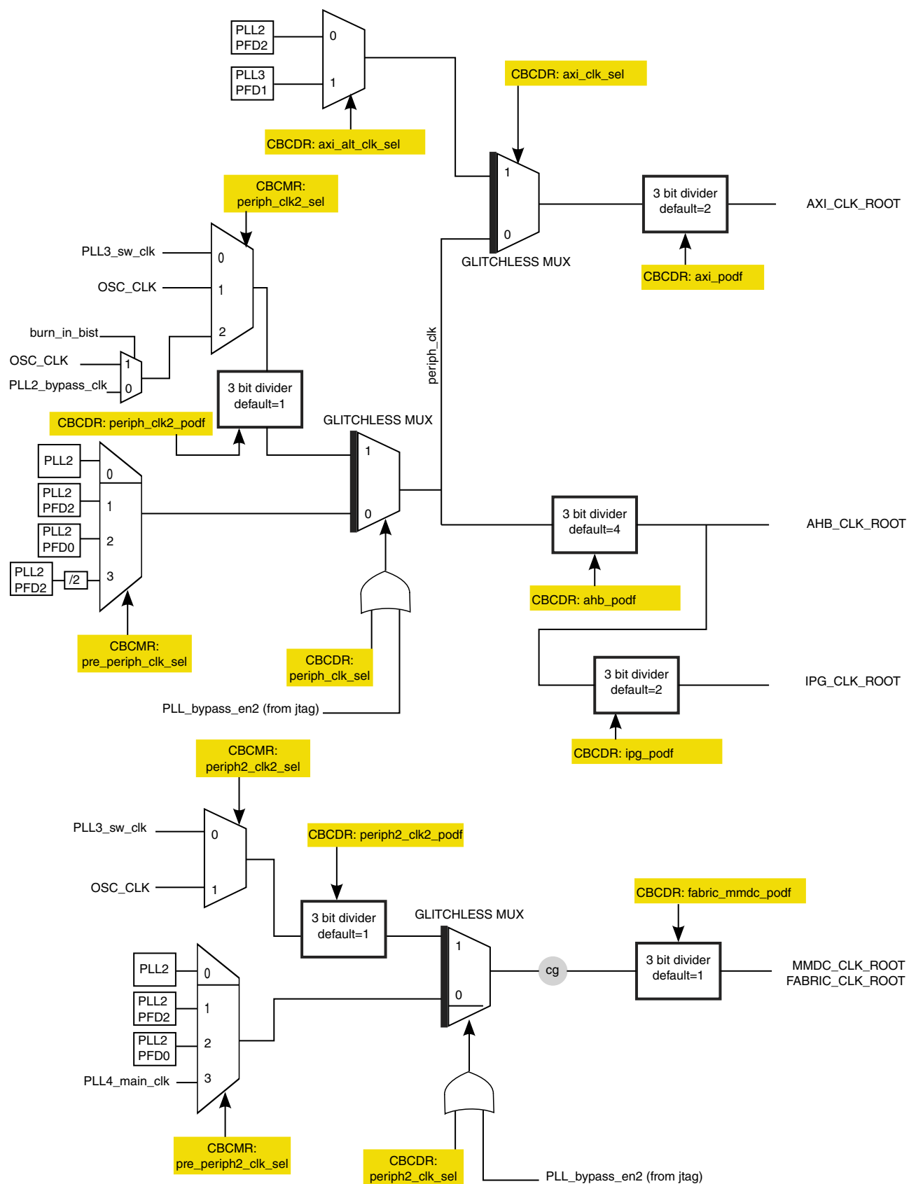
Figure 18-5. BUS clock generation
