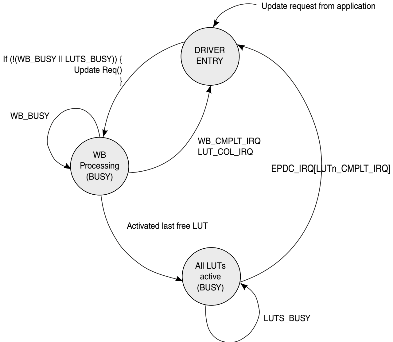
Figure 23-10. Driver Update Flow
