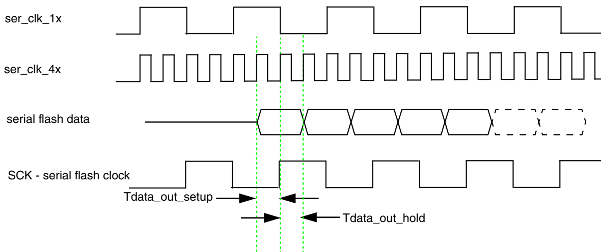
Figure 42-20. Output timing in DDR mode
