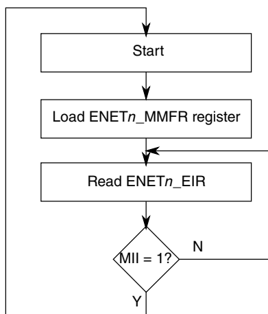
Figure 22-18. MDIO access overview
