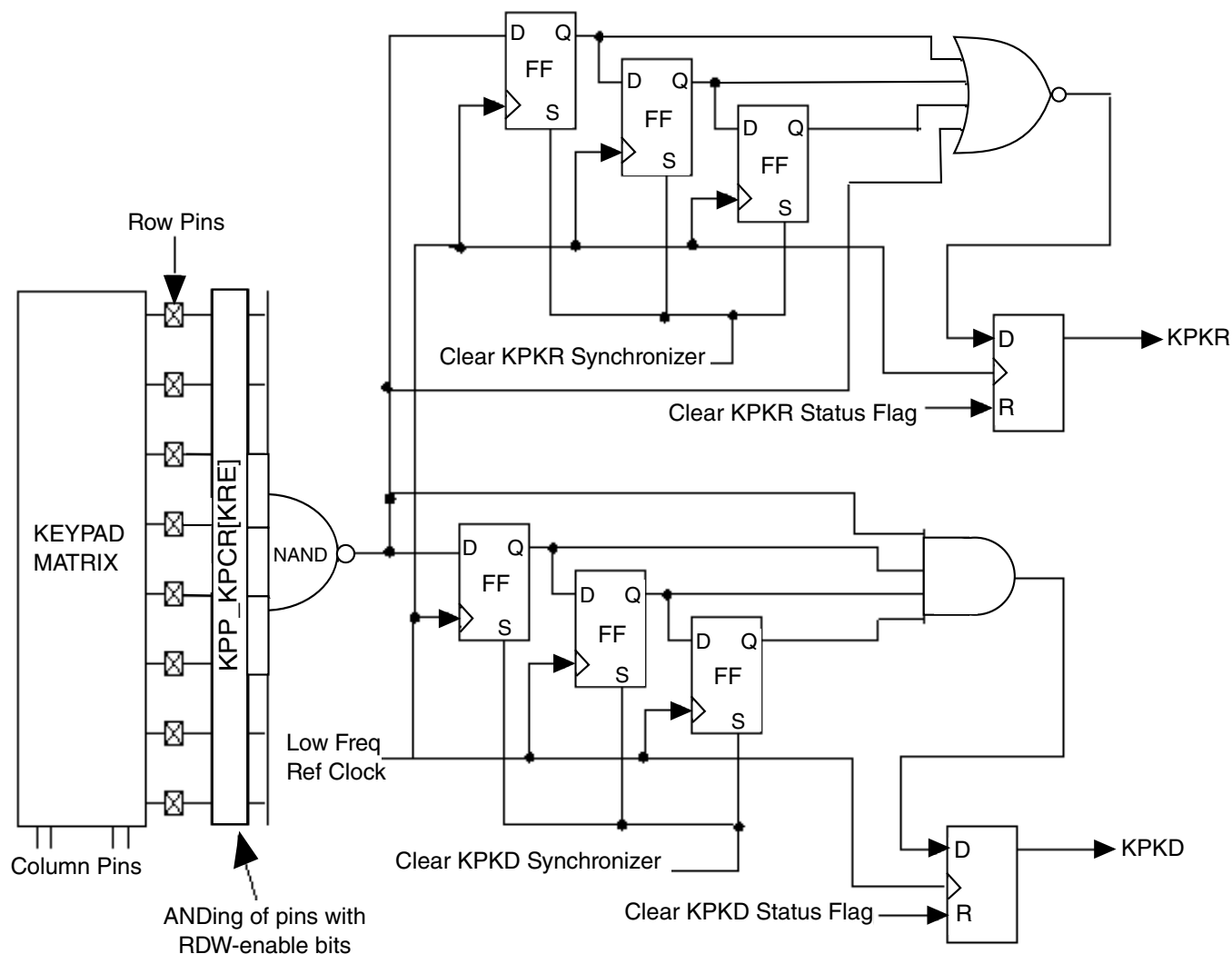
Figure 33-2. Keypad Synchronizer Functional Diagram
