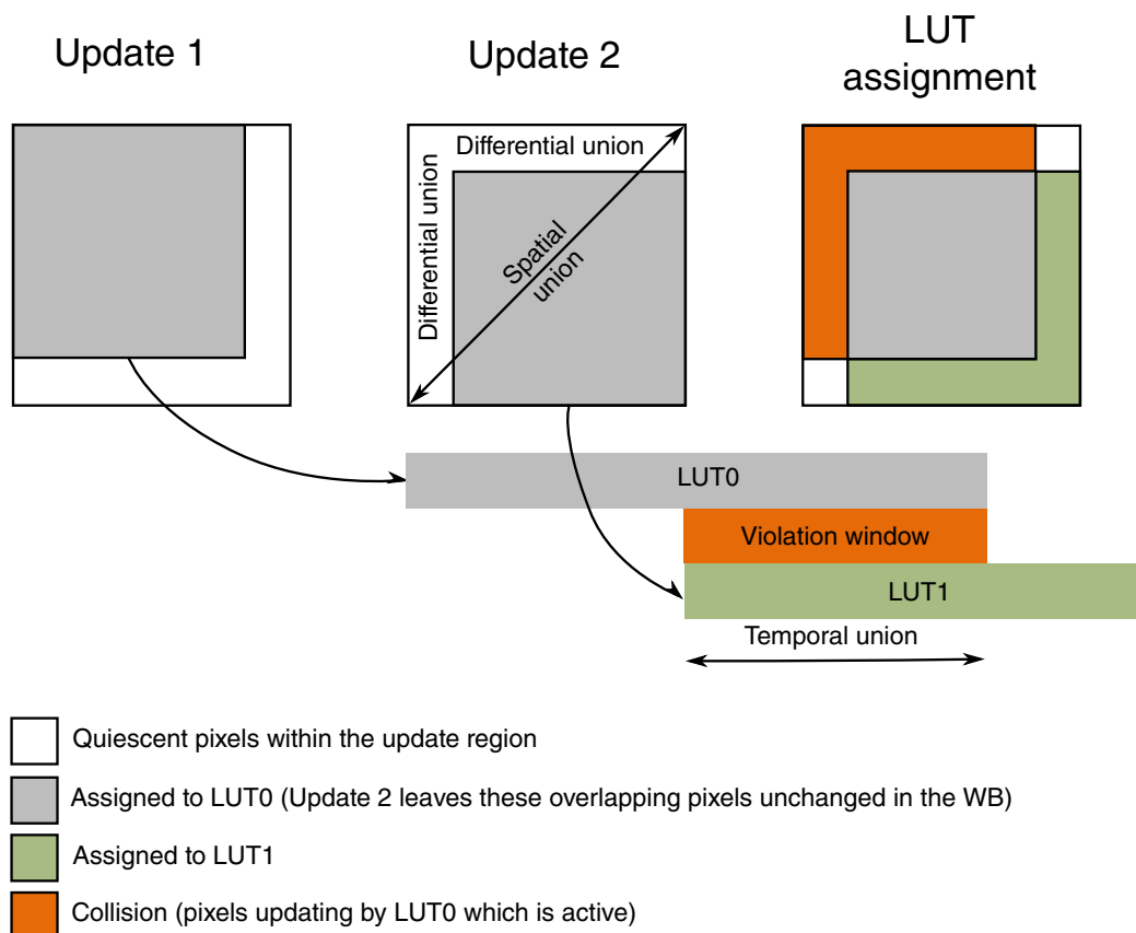
Figure 23-8. Partial Update Collision Handling
