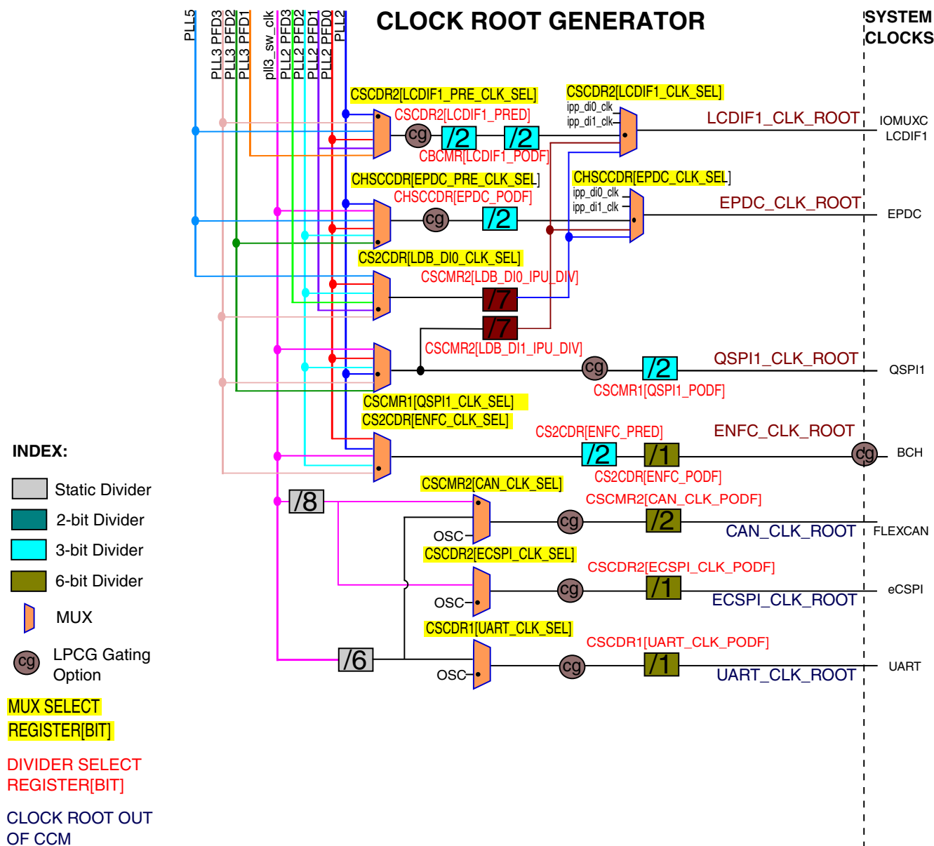
Figure 18-3. Clock Tree - Part 2
