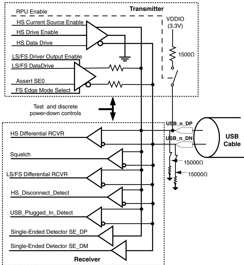
Figure 57-1. USB 2.0 PHY Analog Transceiver Block Diagram
