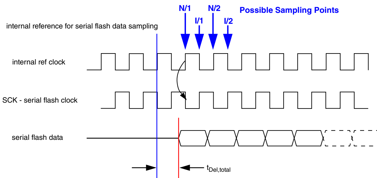
Figure 42-11. Serial Flash Sampling Clock Timing
