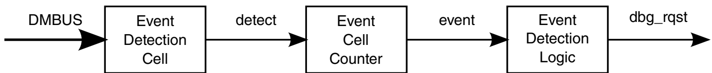
Figure 46-13. Event Detection Unit
