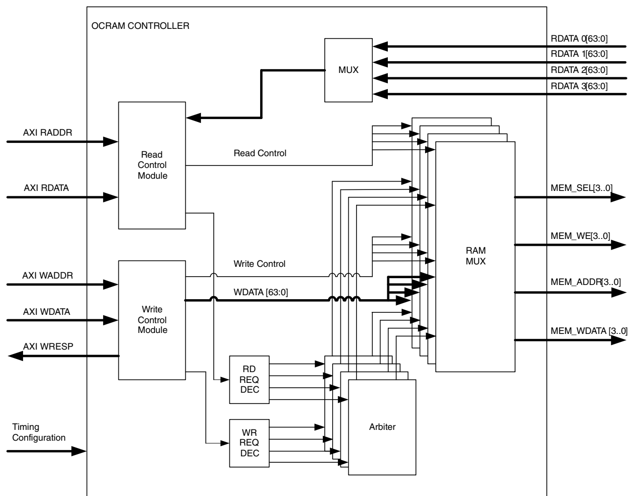
Figure 38-1. On-chip RAM Block Diagram
