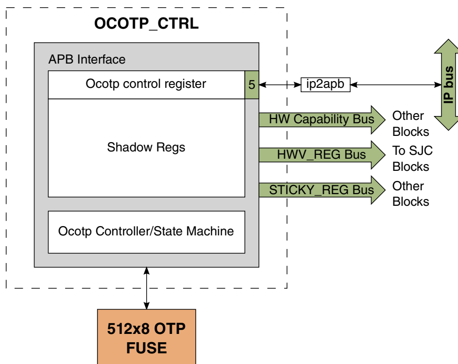
Figure 37-1. OCOTP System Level Diagram
