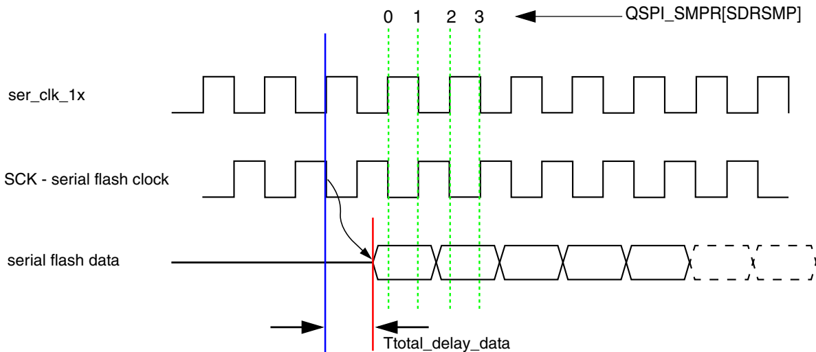
Figure 42-13. Internal sample SDR
