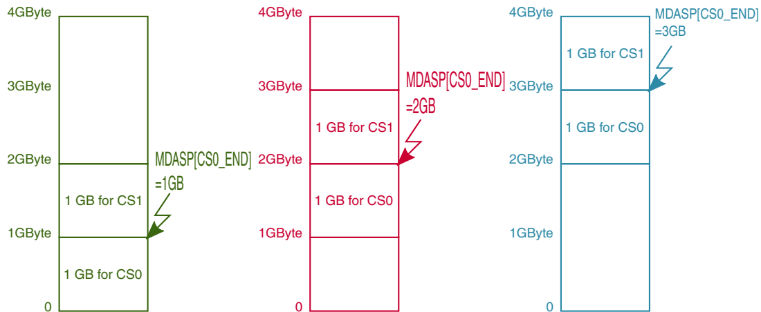
Figure 35-3. Chip select partition—1 Gbyte per chip select
