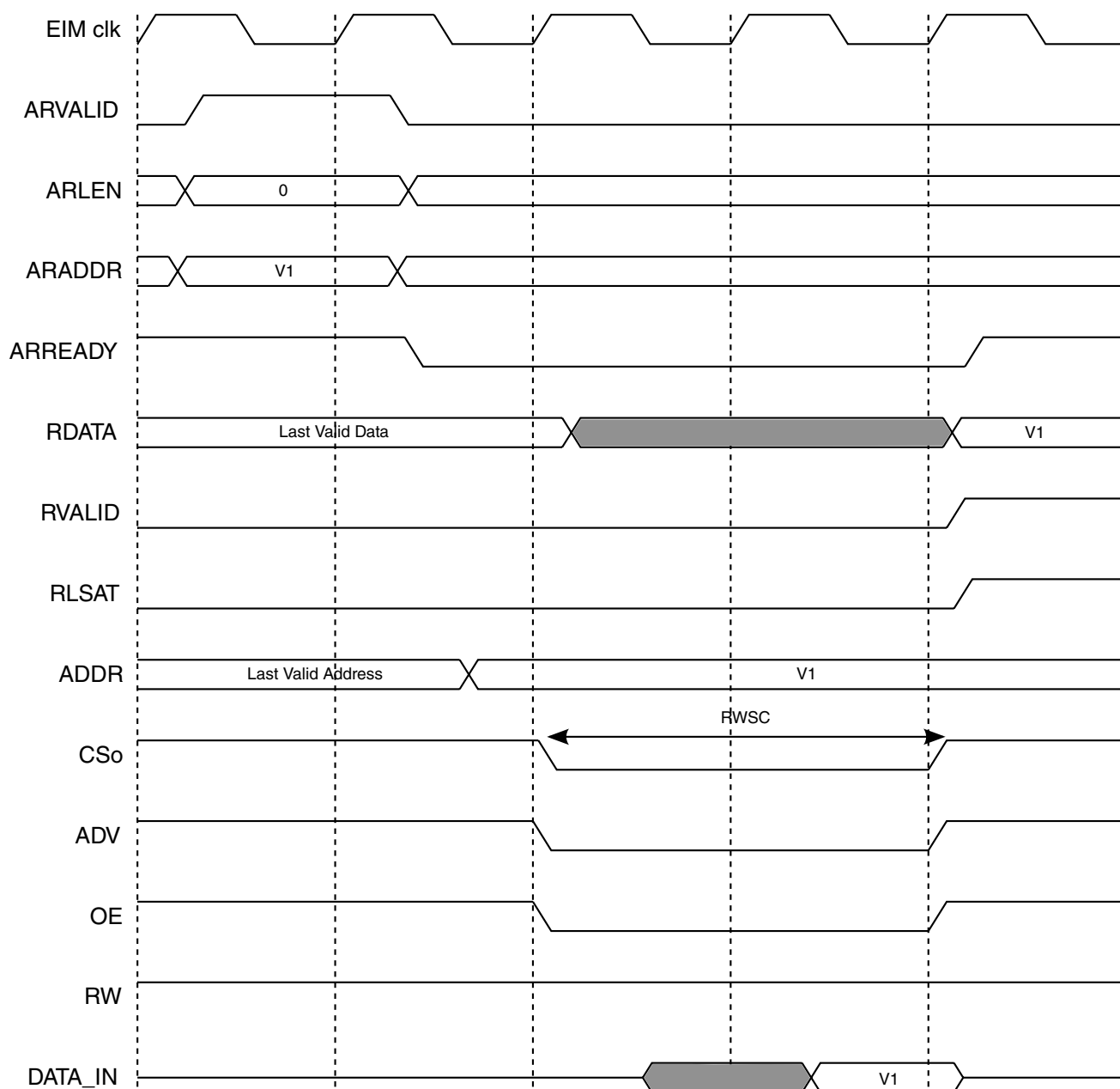
Figure 21-2. Read Access, RWSC=2,RCSA=0,OEA=0,RCSN=0,OEN=0, RAL=1
