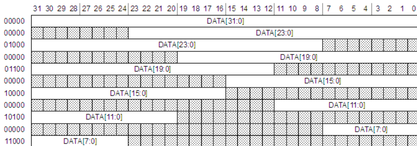
Figure 45-3. SAI first bit shifted, LSB first
