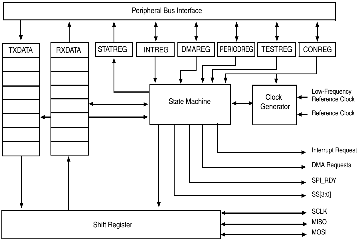
Figure 20-1. ECSPI Block Diagram
