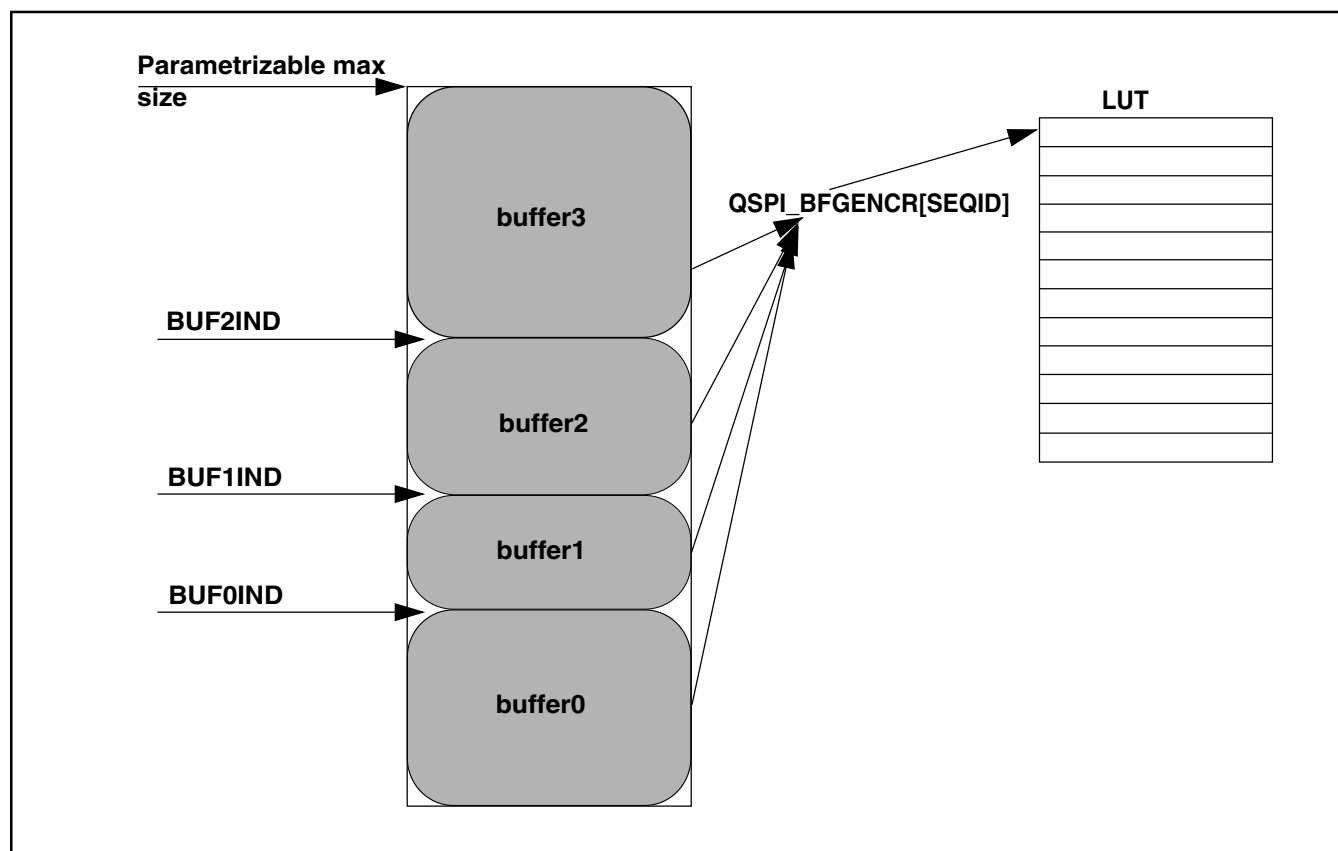
Figure 42-4. Flexible AHB Buffers
