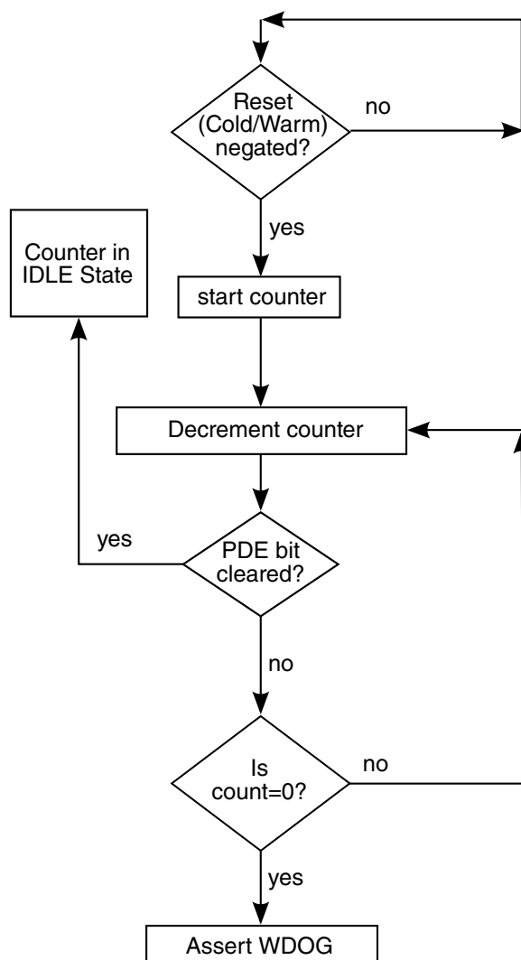
Figure 59-6. Power-Down Counter Flow Diagram
