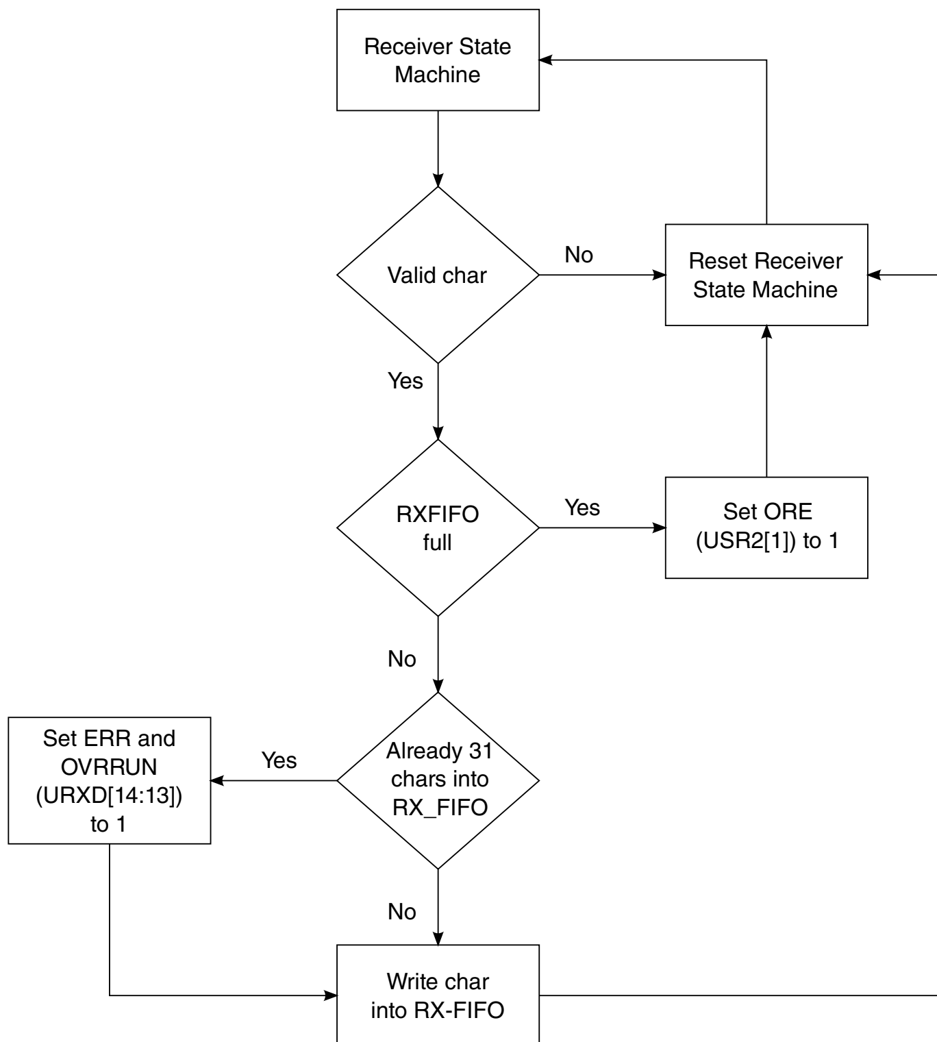
Figure 55-5. Receiver Flow Chart
