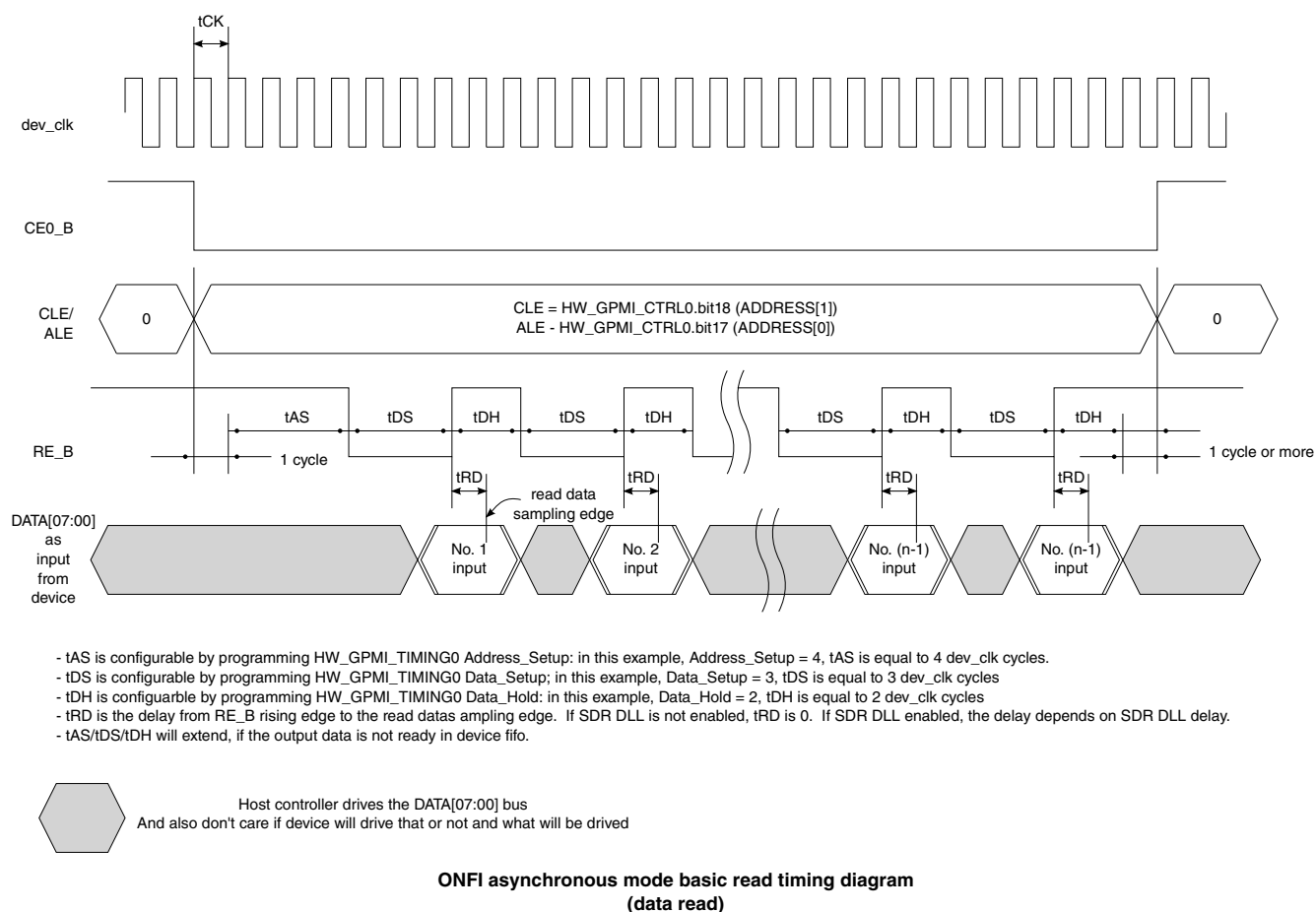
Figure 29-3. ONFI Asynchronous Mode Basic Read Timing Diagram (data read)
