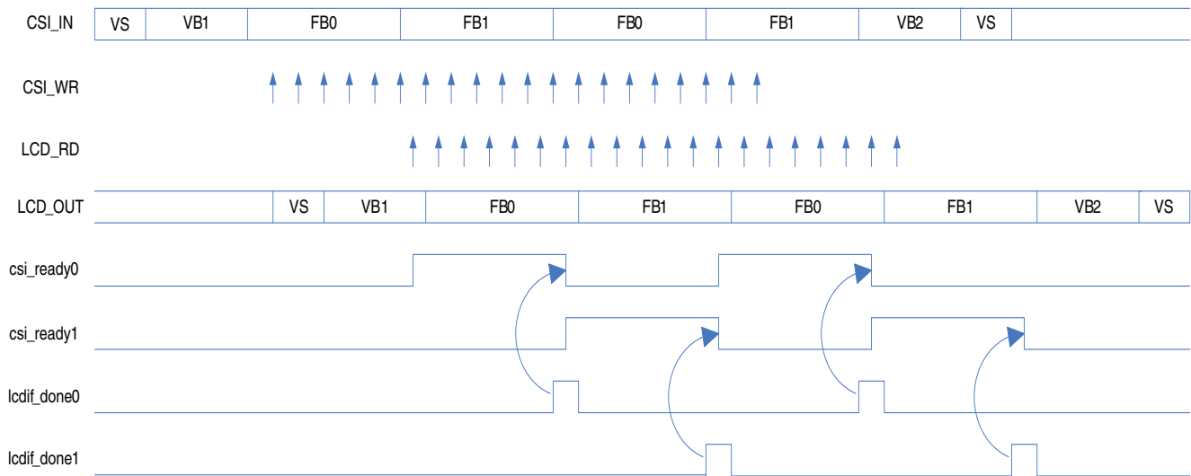
Figure 34-14. CSI HandShake Interface
