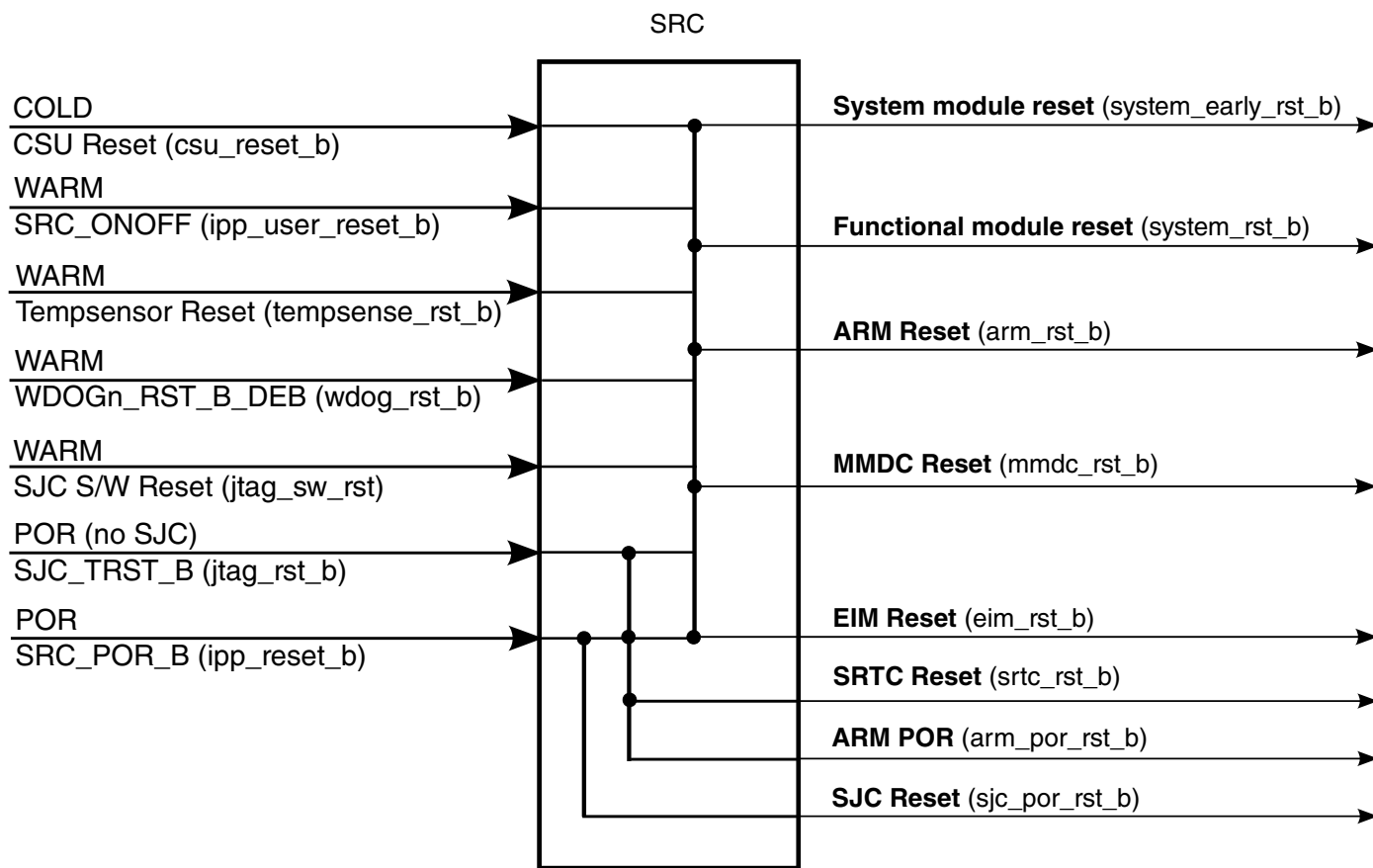
Figure 51-5. SRC inputs and outputs
