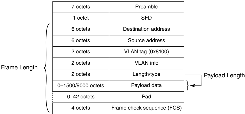
Figure 22-3. VLAN-tagged MAC frame format overview
