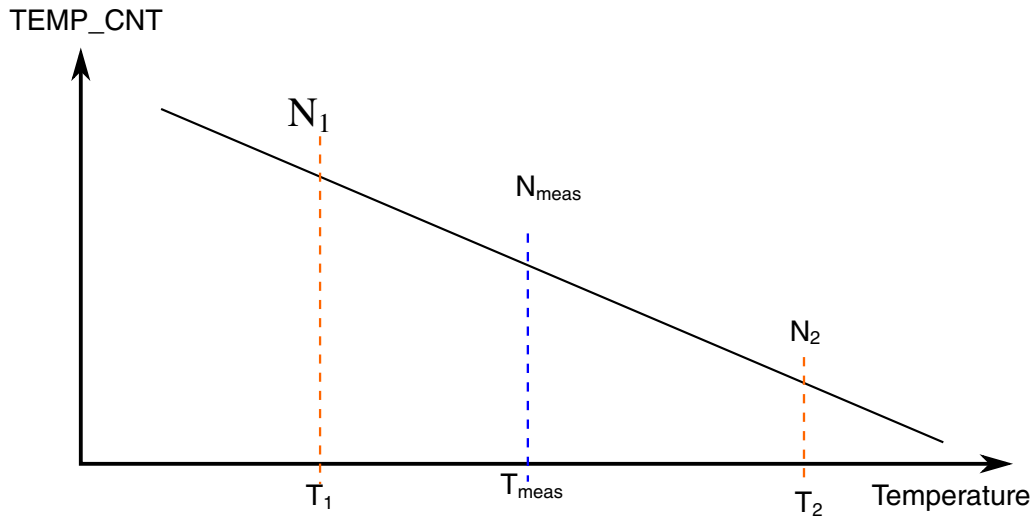
Figure 52-2. Temperature Measurement Cycle
