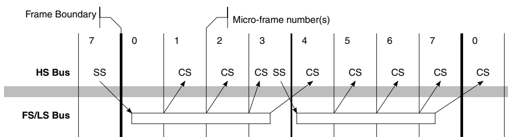
Figure 56-9. Frame Boundary Relationship between HS bus and FS/LS Bus
