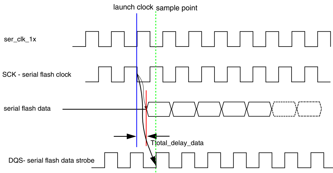
Figure 42-16. Input timing in SDR mode with flash DQS sampling
