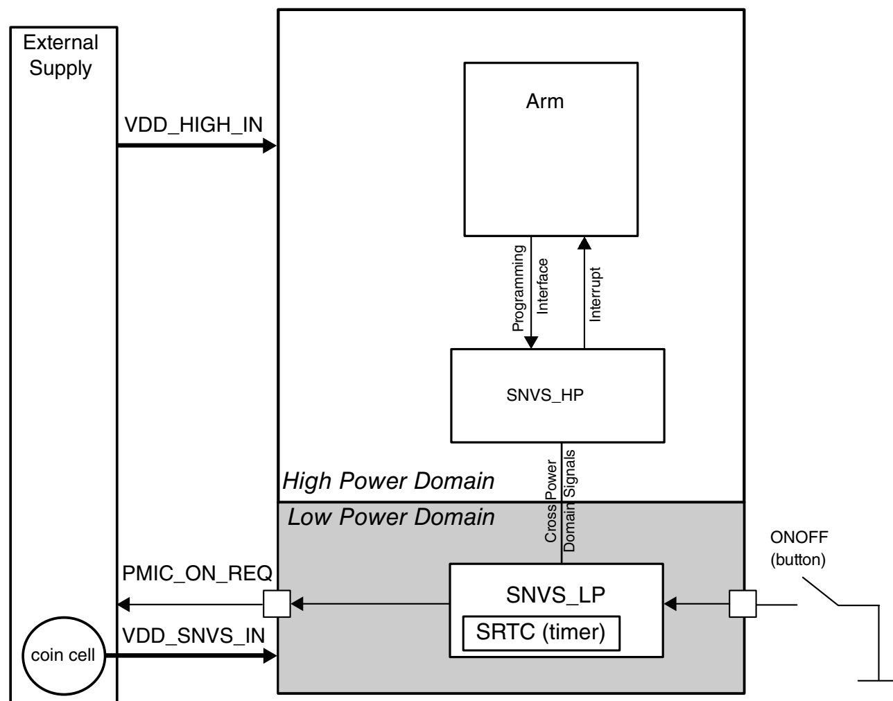
Figure 48-1. SNVS Power Domains
