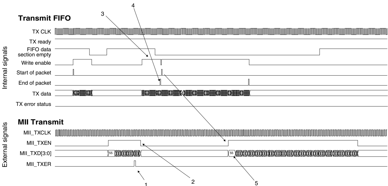
Figure 22-16. Transmit FIFO underflow protection
