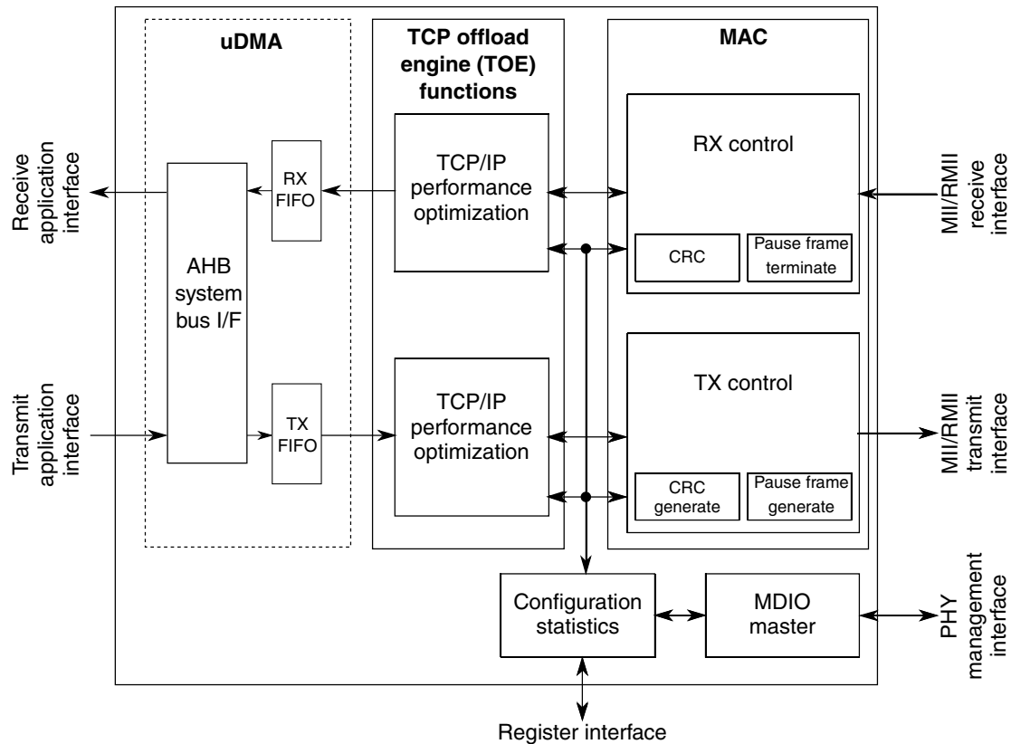
Figure 22-1. Ethernet MAC-NET core block diagram
