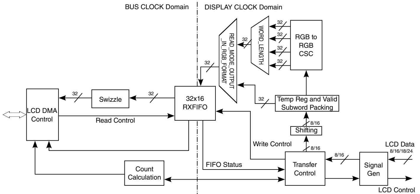
Figure 34-7. MPU Read Data Path
