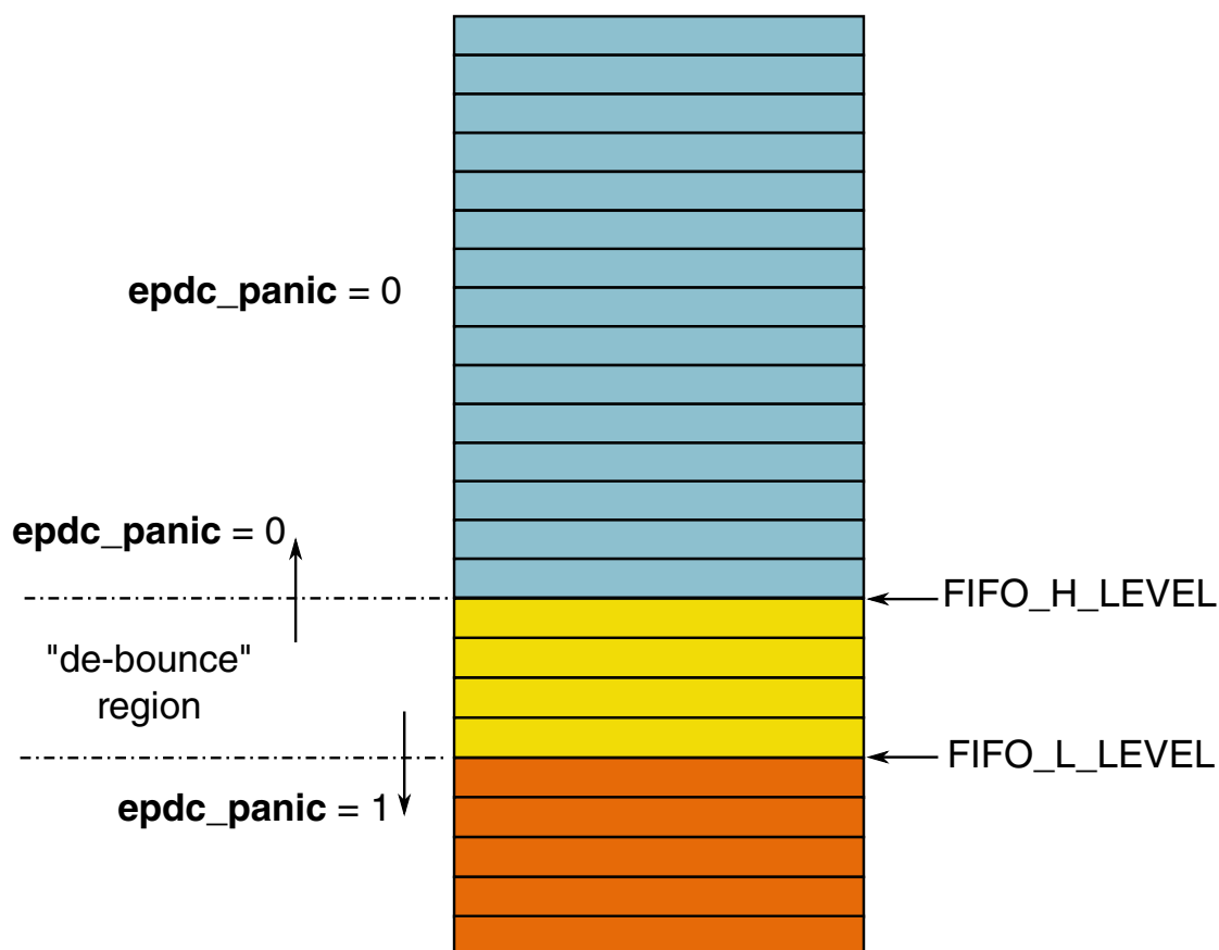
Figure 23-12. FIFO Priority Elevation
