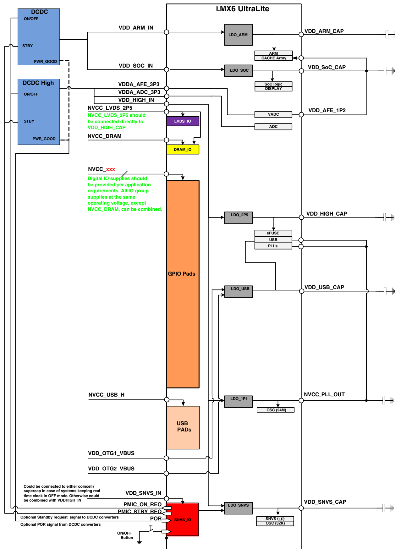
Figure 10-10. Supplying i.MX6ULL power using integrated PMU i.MX6ULL Applications Processor Reference Manual, Rev. 1, 11/2017
