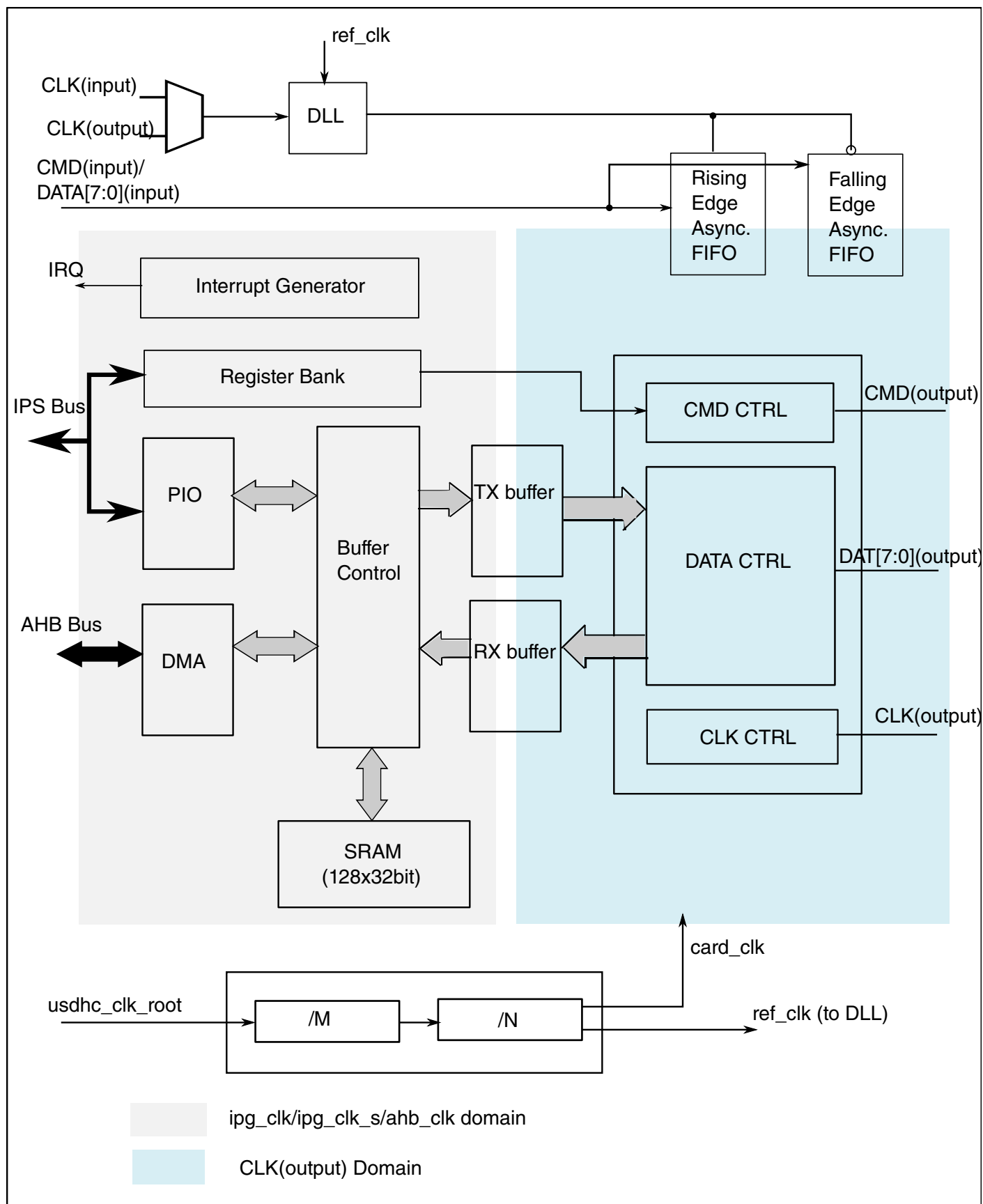
Figure 58-2. ultra Secure Digital Host Controller Block Diagram
