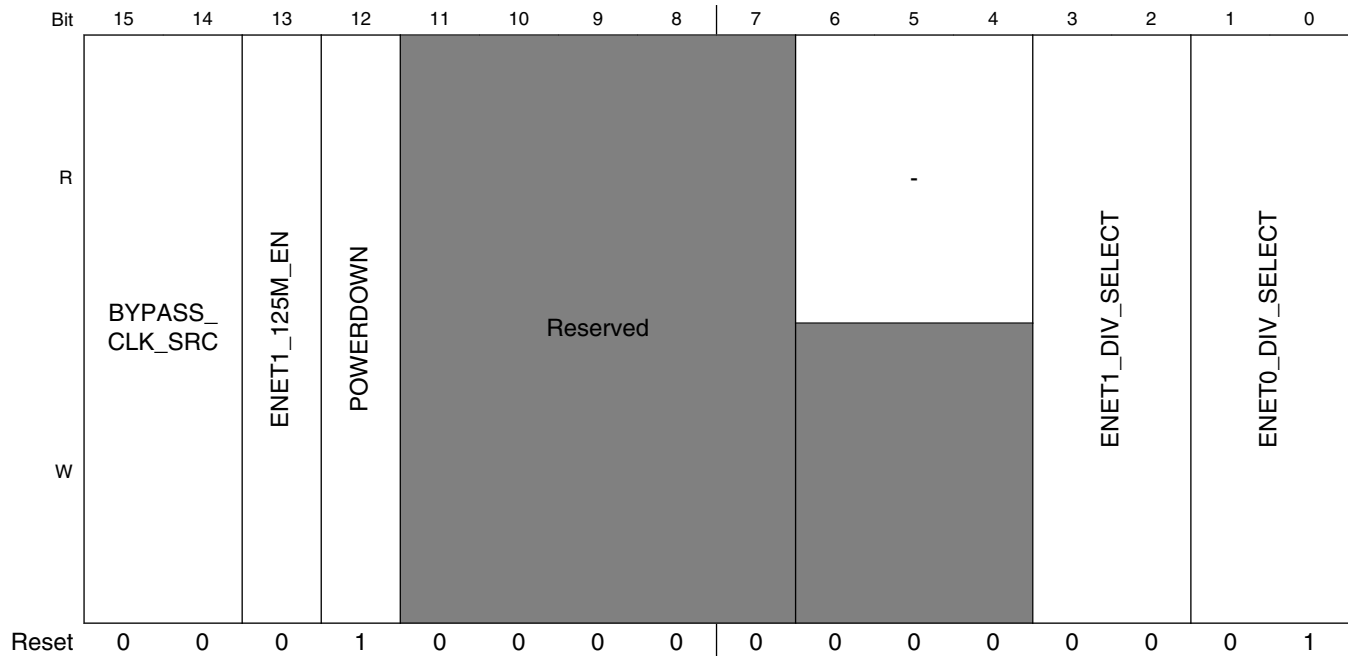
CCM_ANALOG_PLL_ENETn field descriptions
