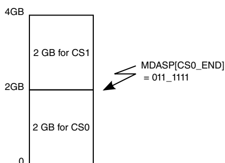
Figure 35-2. Chip select partition—2 Gbytes per chip select
