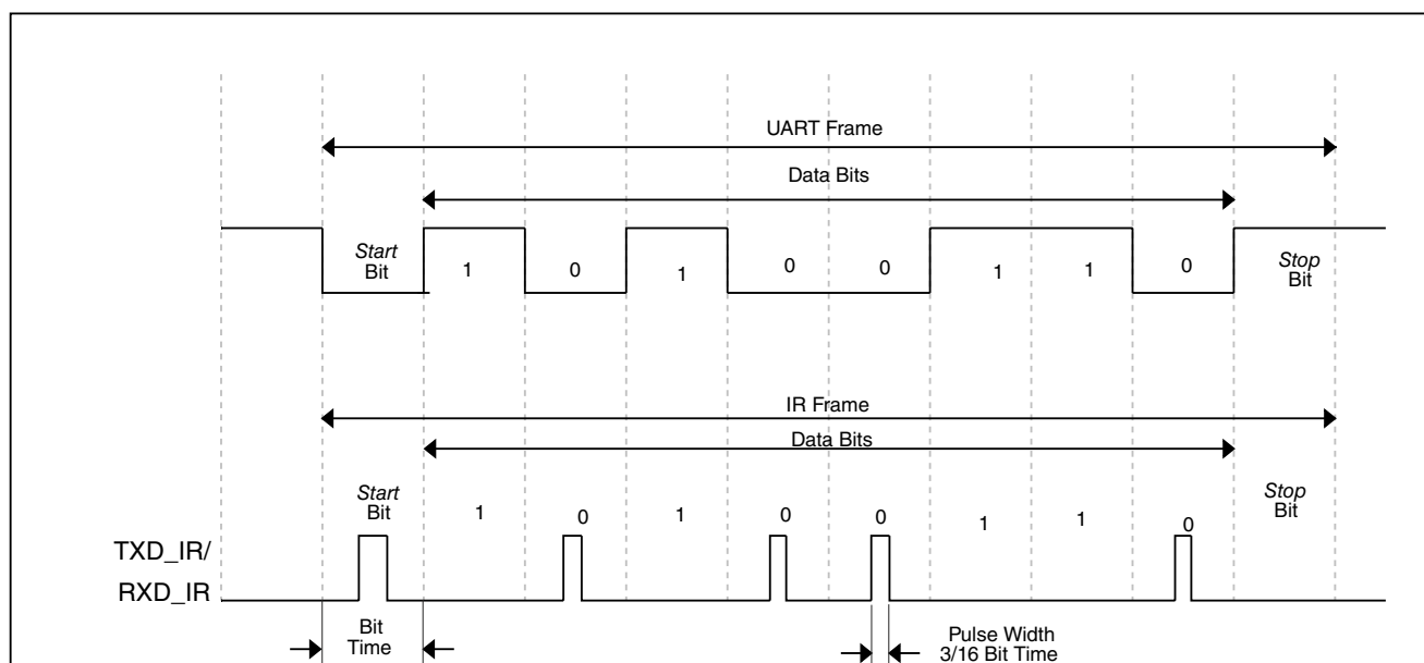
Figure 55-13. Timing diagram of Low Speed IR (<=115.2 Kbit/s) Data Line
