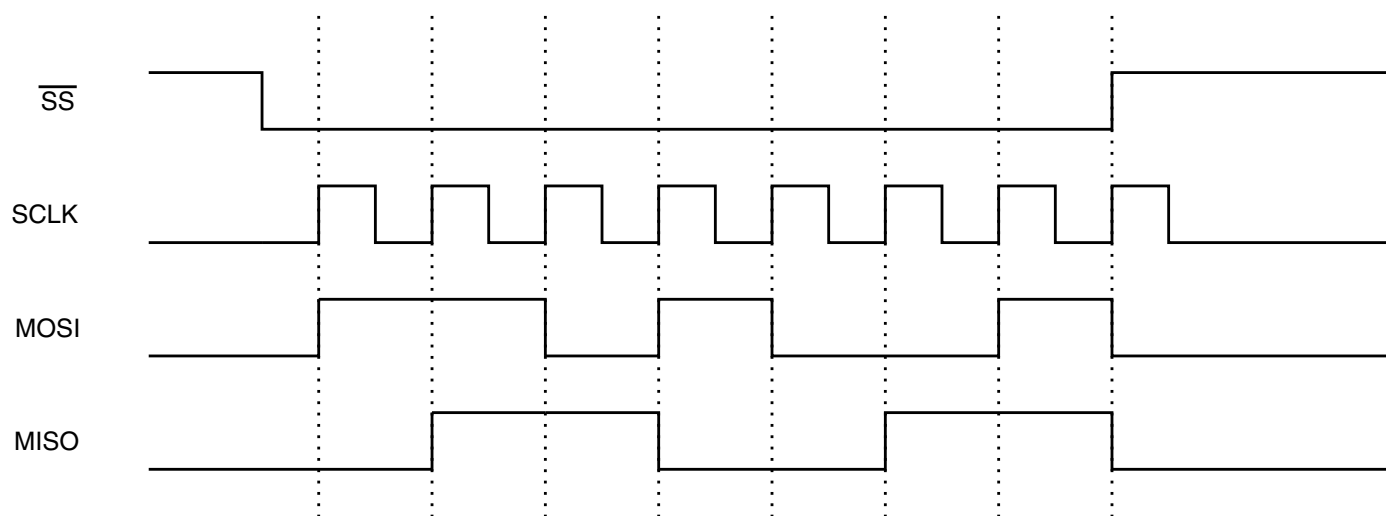
Figure 20-11. Advancing the Data FIFO on the Rising Edge of \overline{SS}
