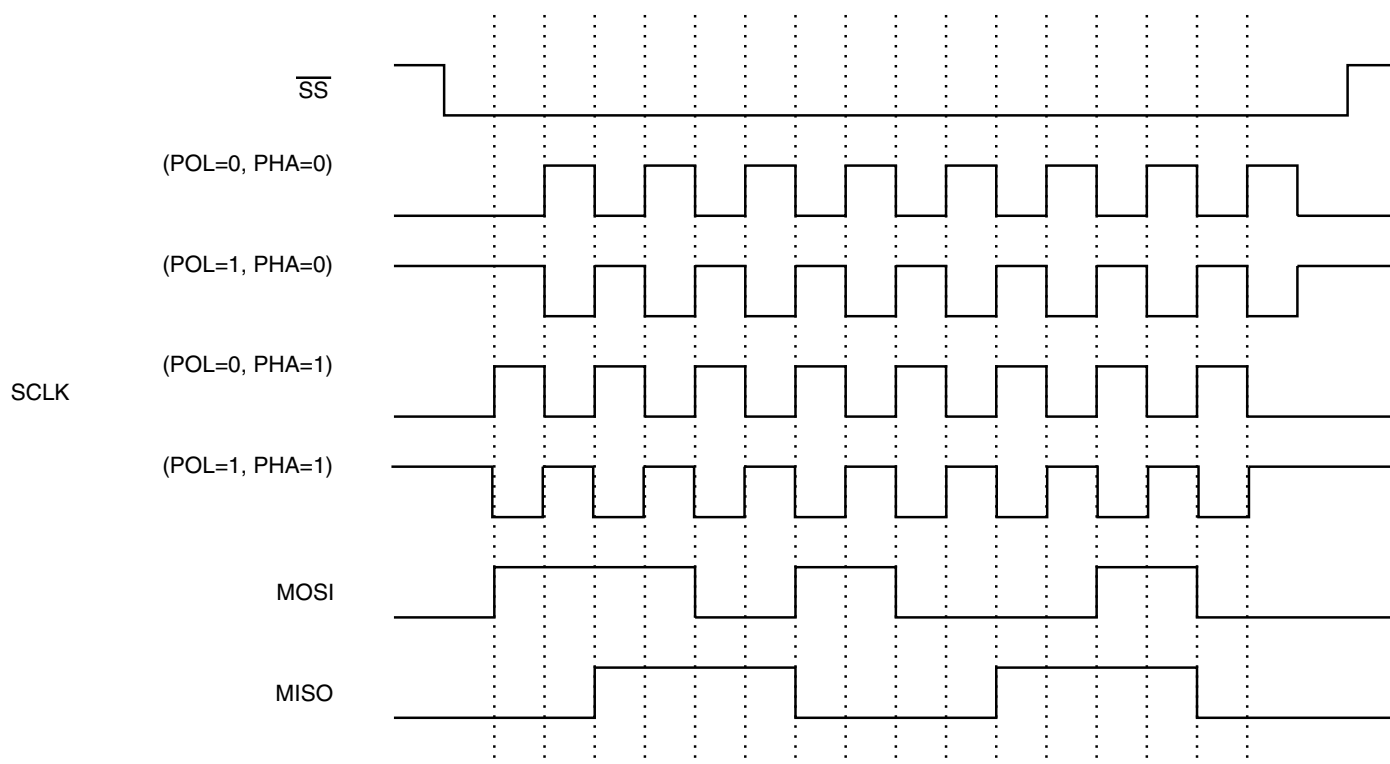
Figure 20-10. SPI Burst with Different POL and PHA Configurations
