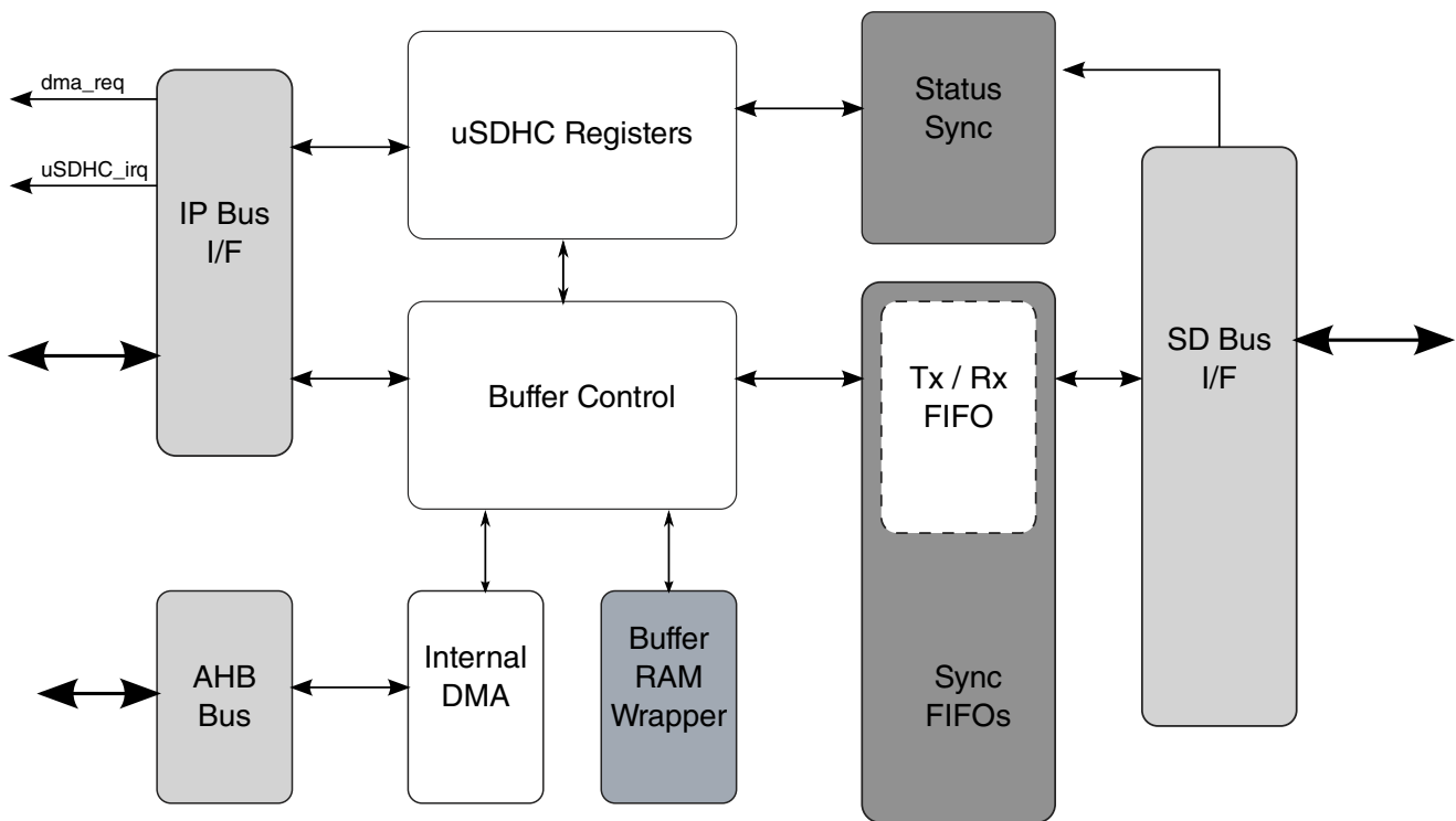
Figure 58-3. uSDHC Buffer Scheme
