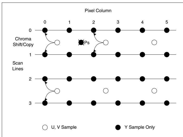
Figure 41-7. YUV Sample Positioning, 4:2:0
