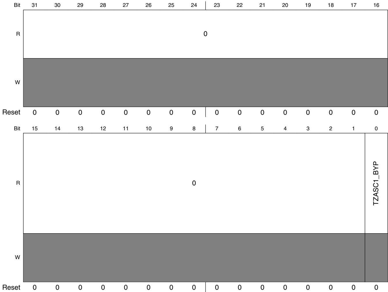
IOMUXC_GPR_GPR9 field descriptions
