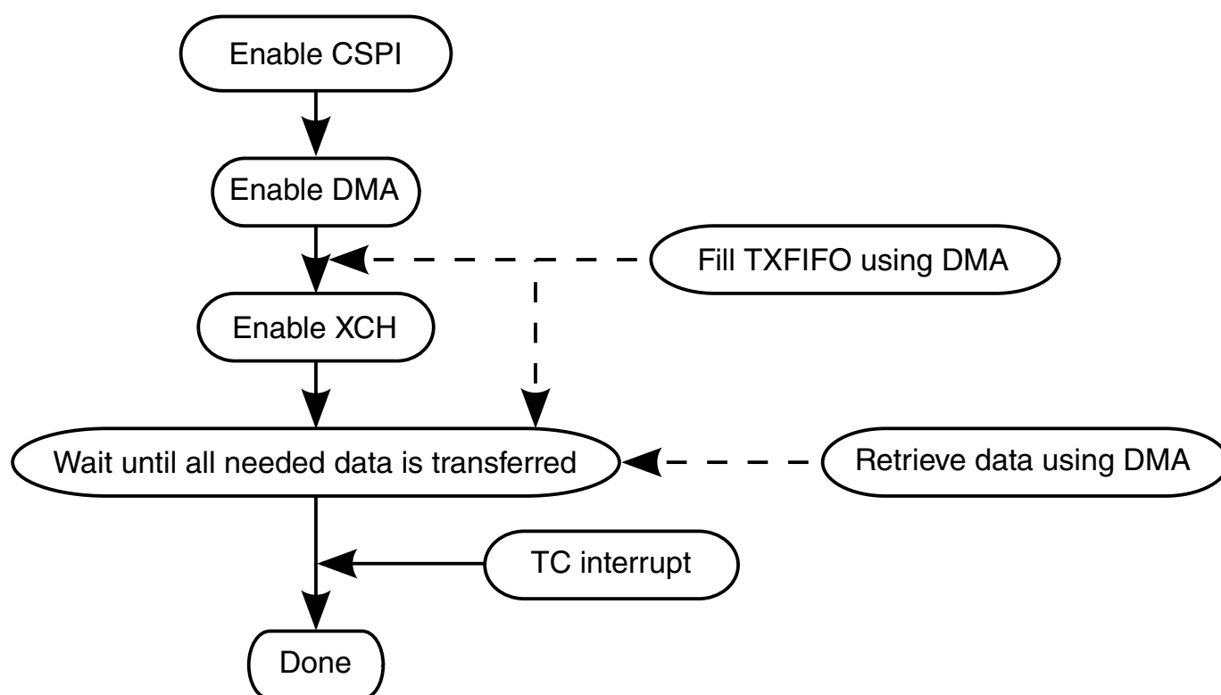
Figure 20-13. Program Sequence of SPI Burst Using DMA
