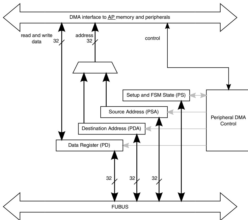
Figure 46-10. Peripheral DMA structure
