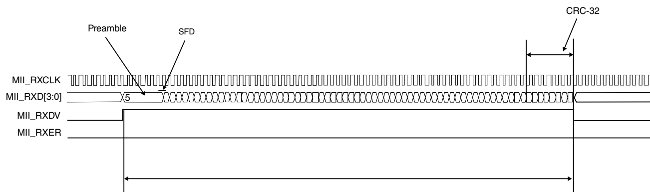
Figure 22-25. MII receive operation
