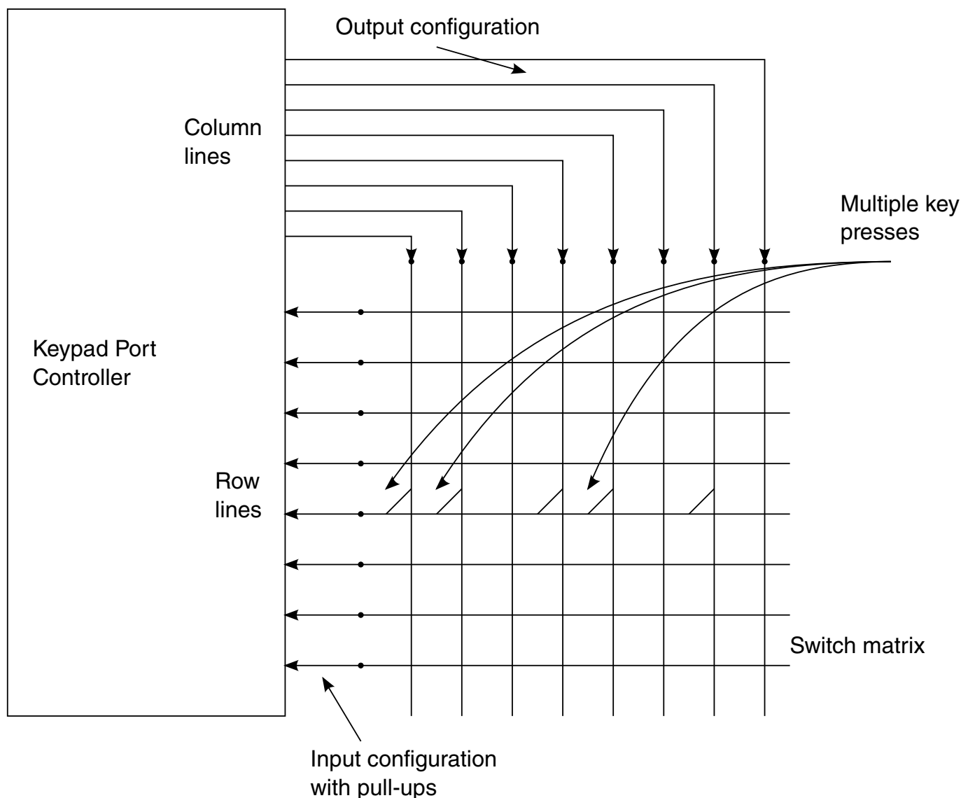
Figure 33-4. Multiple Key Presses on Same Row Line (Simplified View)
