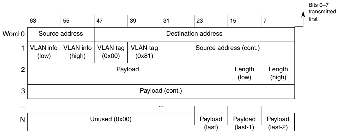
Figure 22-15. VLAN-tagged frame 64-bit mapping example
