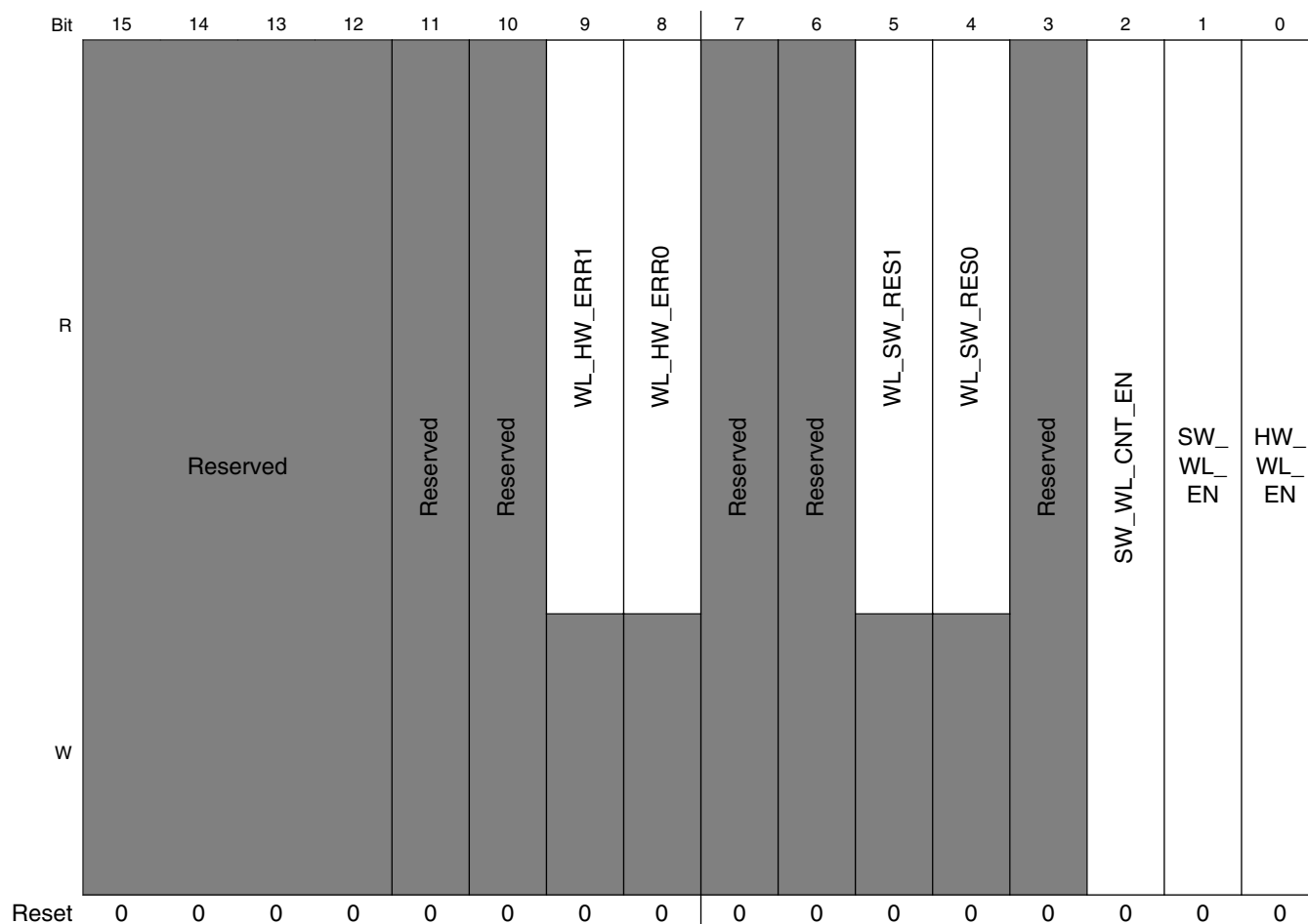
MMDC_MPWLGCRCR field descriptions
