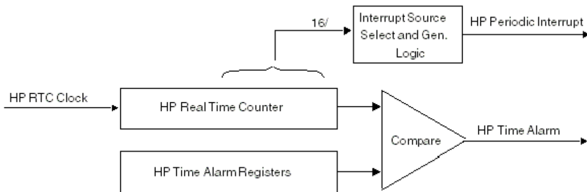
Figure 48-2. SNVS_HP RTC, alarm, and interrupts
