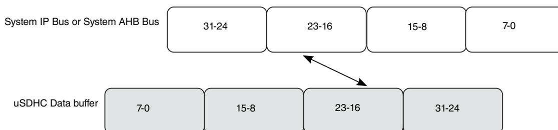
Figure 58-4. Data Swap between System Bus and uSDHC Data Buffer in Byte Little Endian Mode
