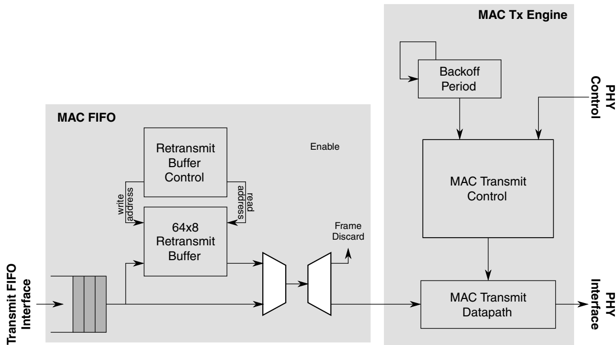
Figure 22-7. Packet re-transmit overview
