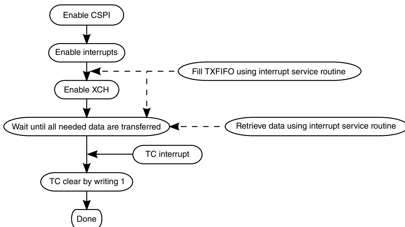
Figure 20-12. Program Sequence of SPI Burst Using Interrupt Control
