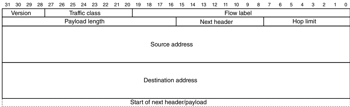
Figure 22-4. IPv6 header format
