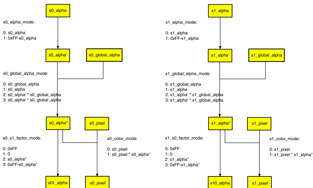
Figure 41-9. Porter-Duff Alpha Blend
