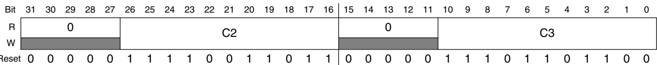
PXP_HW_PXP_CSC1_COEF2 field descriptions
