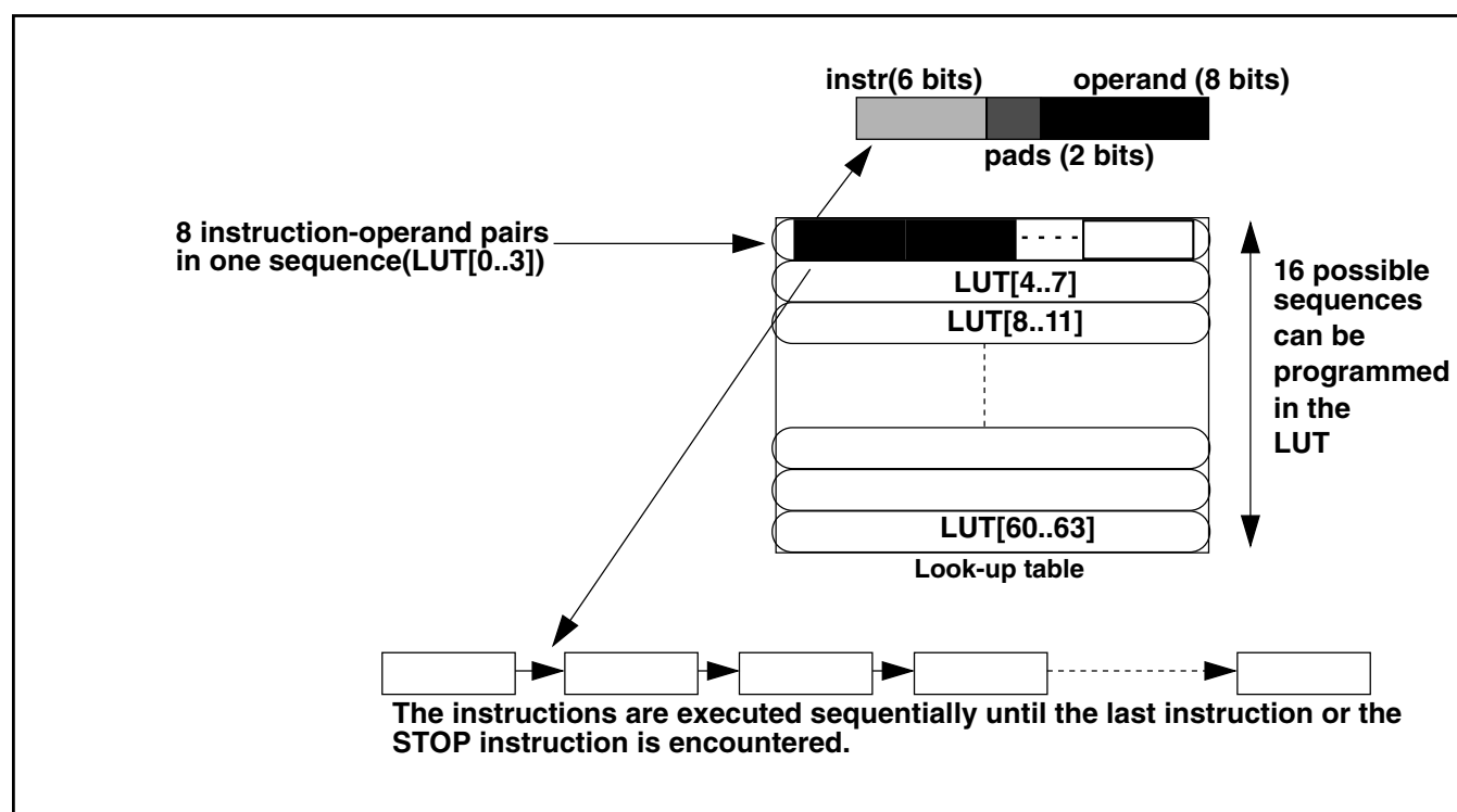
Figure 42-5. LUT and sequence structure
