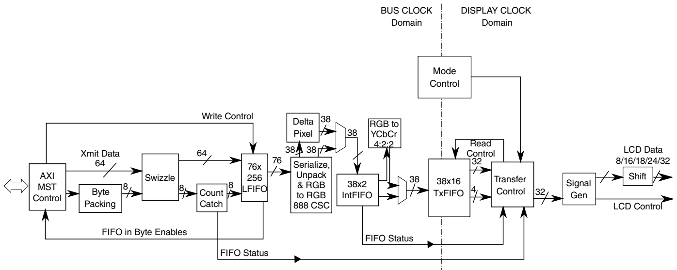
Figure 34-2. General Operations in Write Data Path
