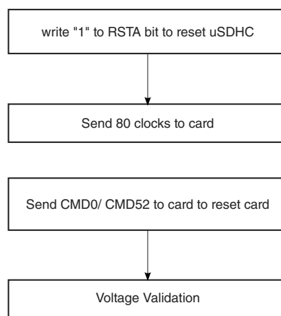
Figure 58-19. Flow Chart for Reset of the uSDHC and SD I/O Card
