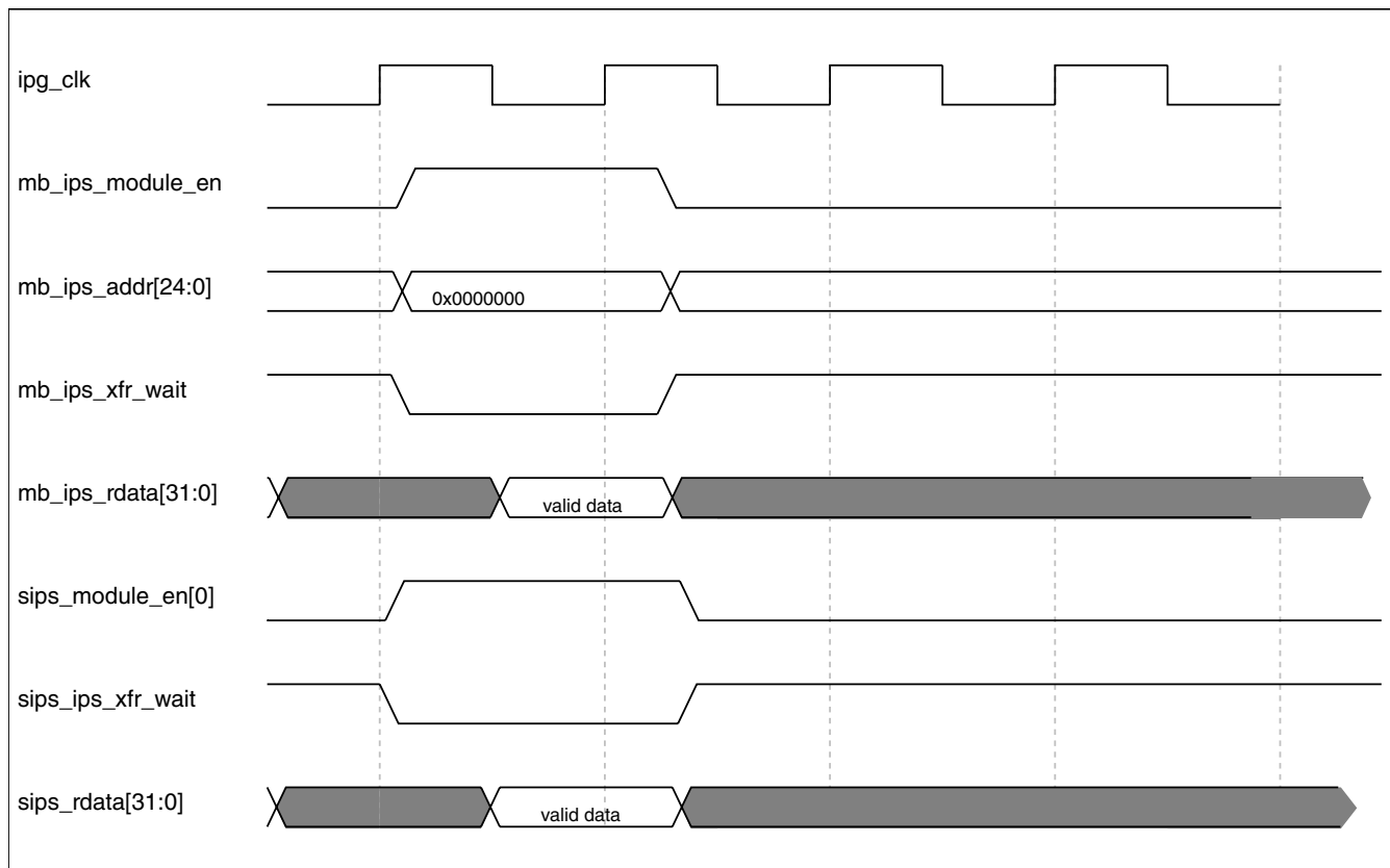
Figure 49-2. Example of one master request, no SPBA arbitration
