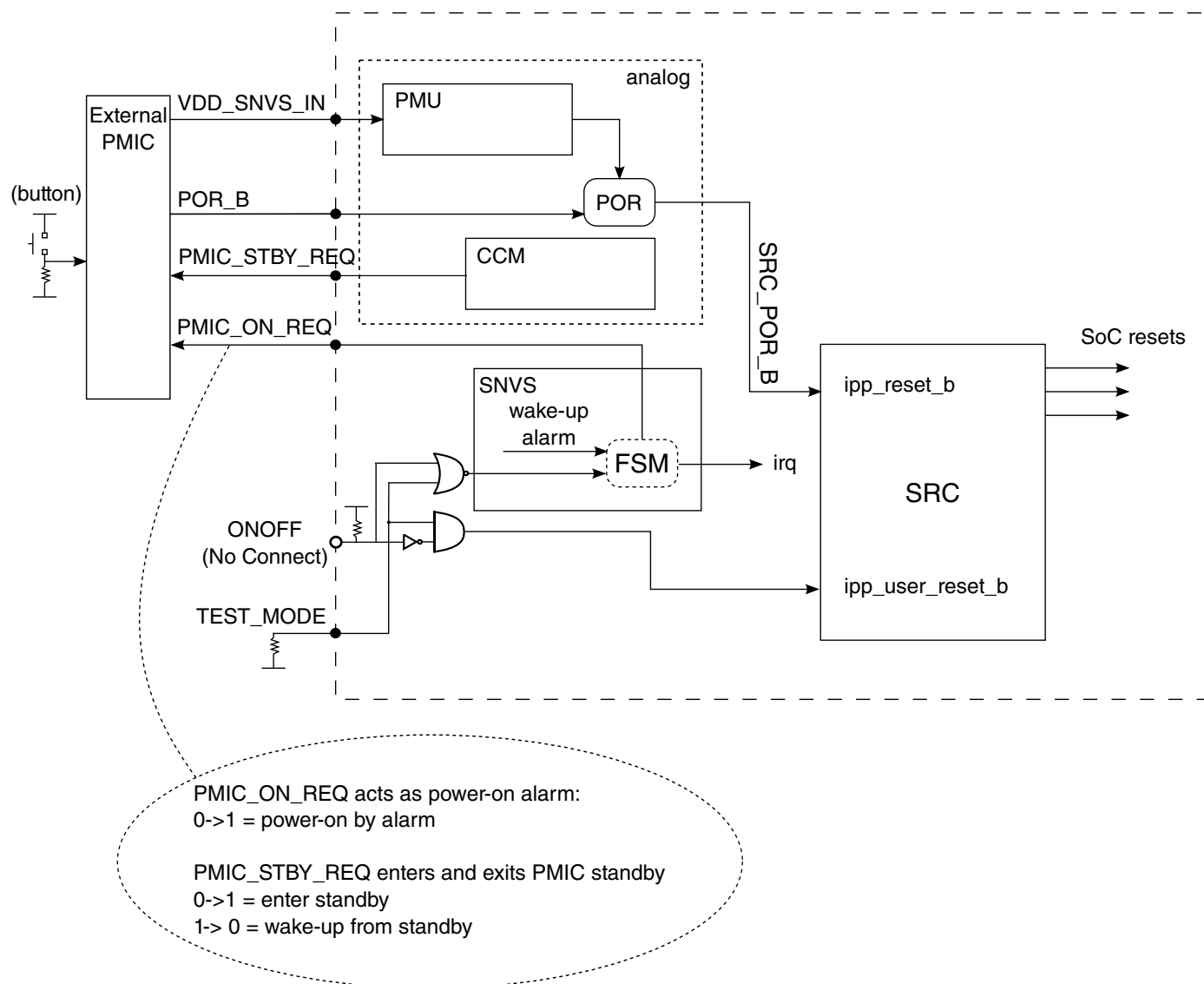
Figure 51-2. Chip reset scheme under external PMIC control
