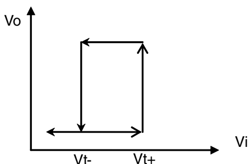
Figure 28-4. Schmitt trigger transfer characteristic
