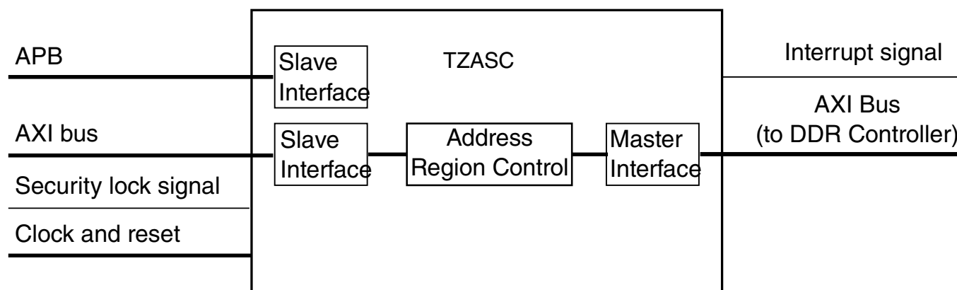
Figure 54-1. TZASC Block Diagram
