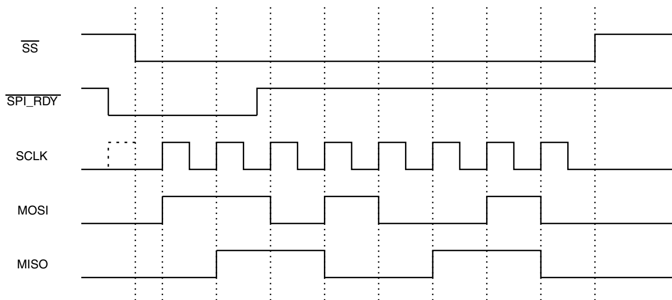
Figure 20-5. Relationship Between a SPI Burst and SPI_RDY: Falling-Edge Triggered
