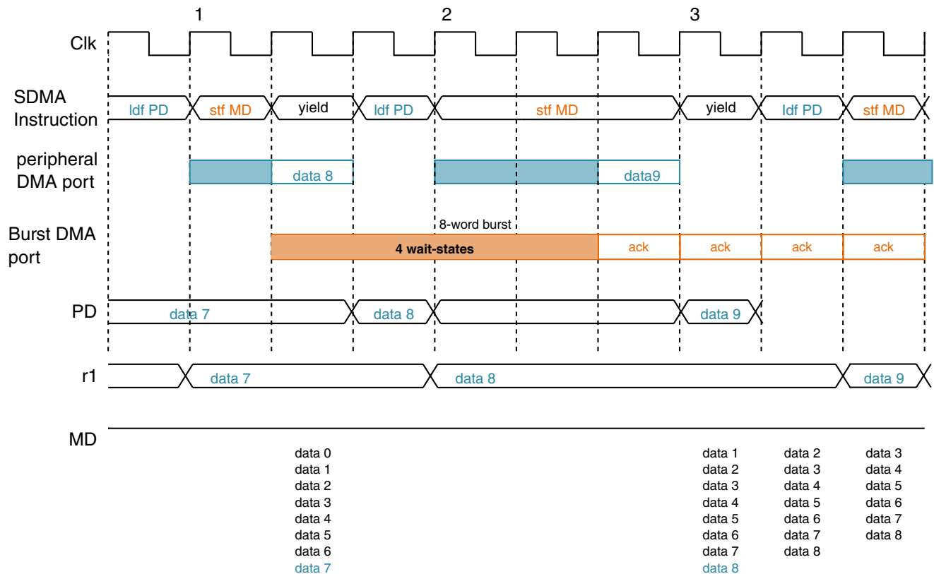
Figure 46-22. Peripheral to External Memory Example (2)
