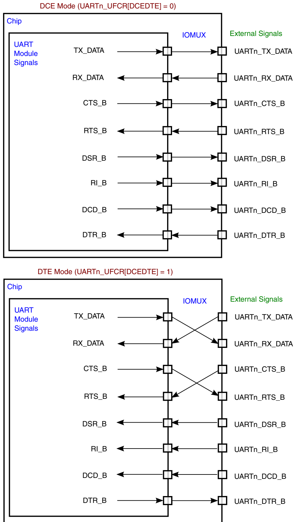
Figure 55-2. UART external signals to module signals routing with respect to DCE/DTE mode
