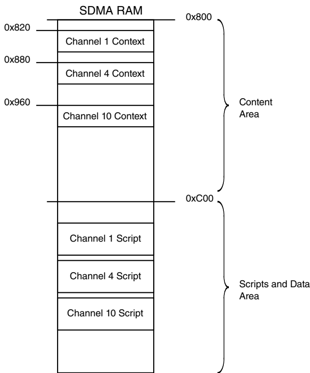
Figure 46-18. Example of SDMA RAM After Boot Session
