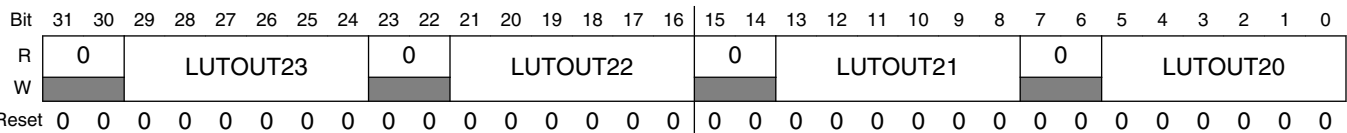
PXP_HW_PXP_WFE_B_STG2_5X6_OUT0_5 field descriptions
