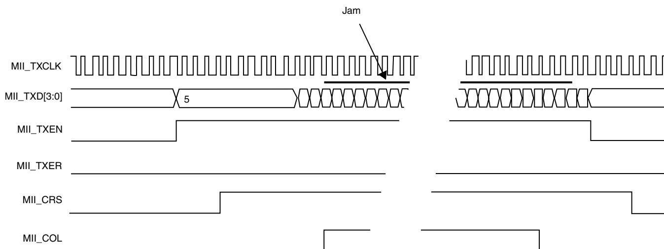
Figure 22-24. MII transmit operation — transmission with collision
