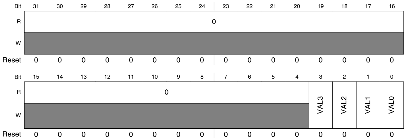
PXP_HW_PXP_WFE_B_SW_FLAG_REGS field descriptions
