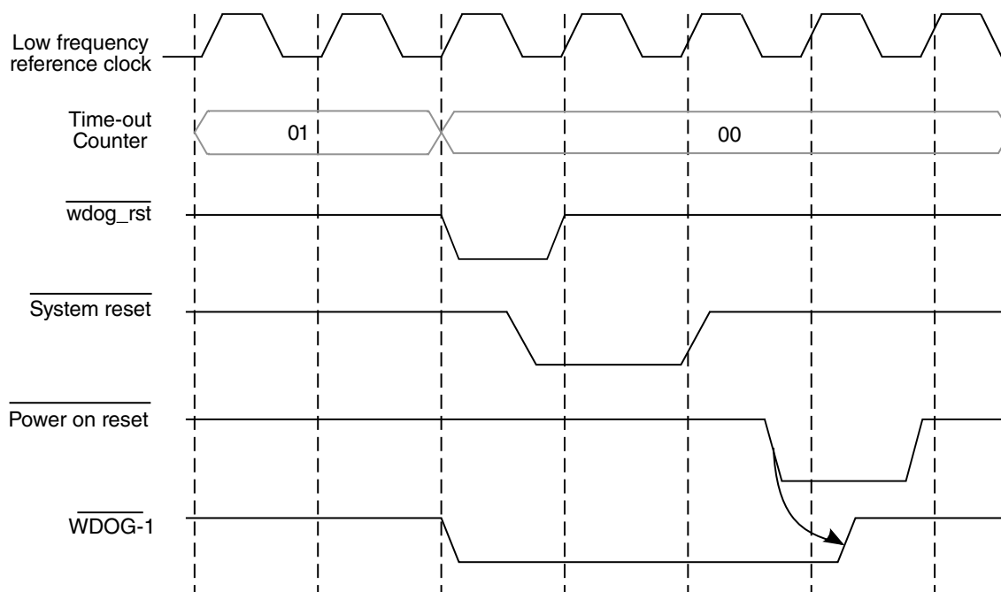
Figure 59-5. WDOG timeout condition/WDT bit is set
