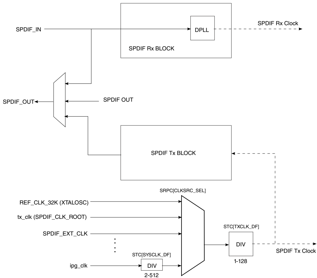
Figure 50-2. SPDIF Transceiver Clock Diagram
