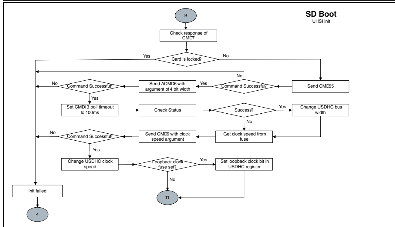
Figure 8-15. Expansion device (MMCSD/eSD/SDXC) boot flow (4 of 6) i.MX 6ULL Applications Processor Reference Manual, Rev. 1, 11/2017
