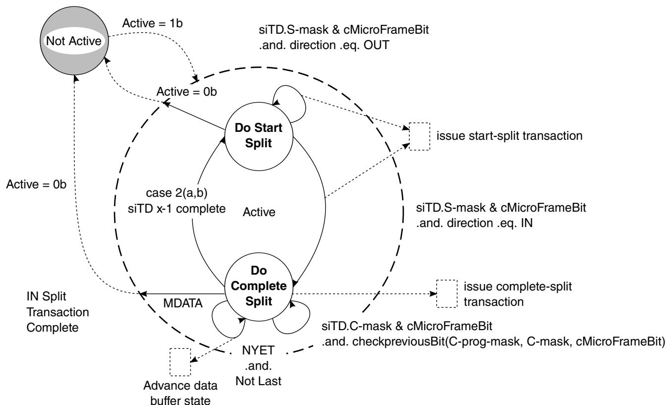
Figure 56-26. Split Transaction State Machine for Isochronous
