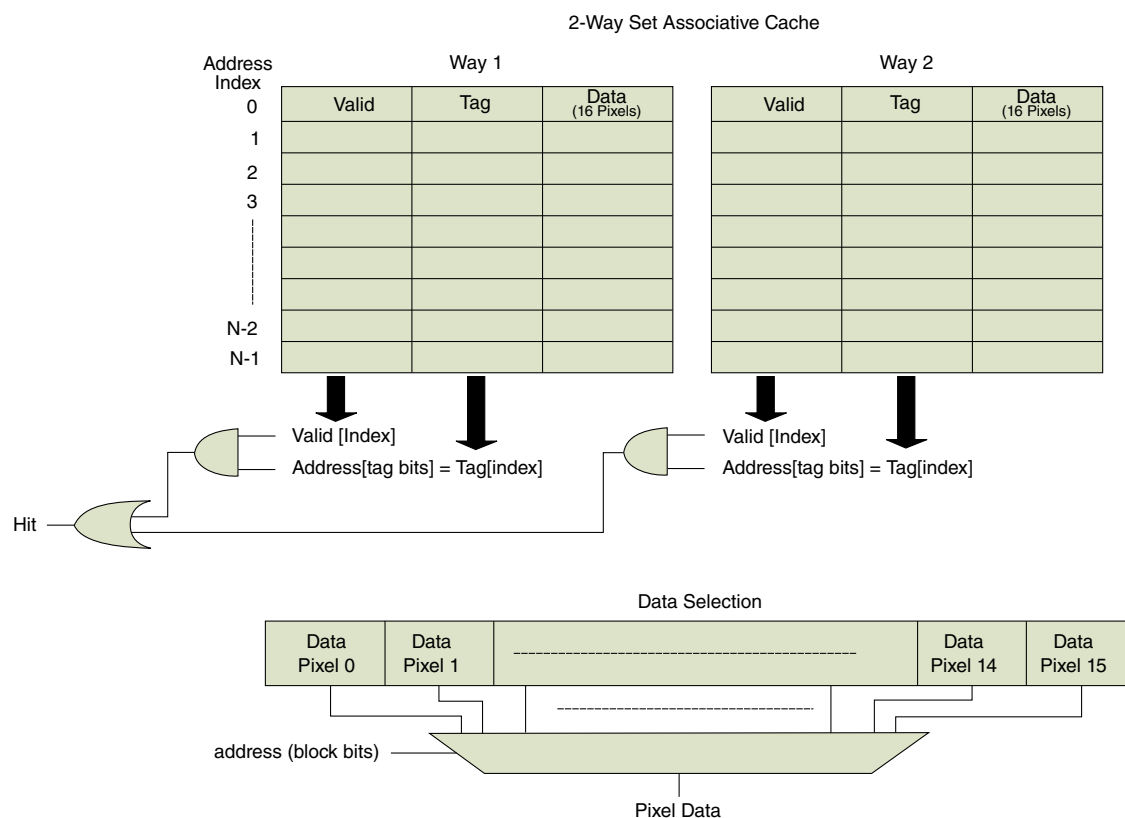
Figure 41-10. 2-Way Set Associative Cache and Data Selection
