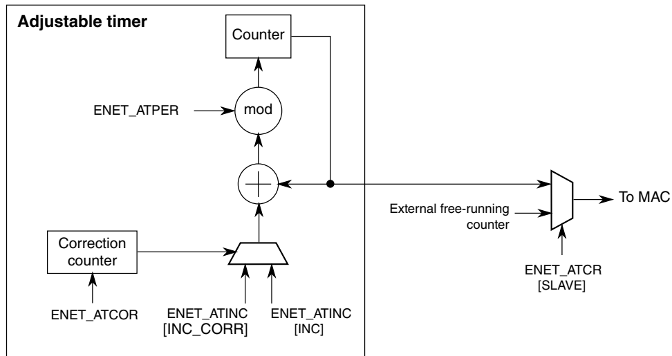
Figure 22-10. Adjustable timer implementation detail
