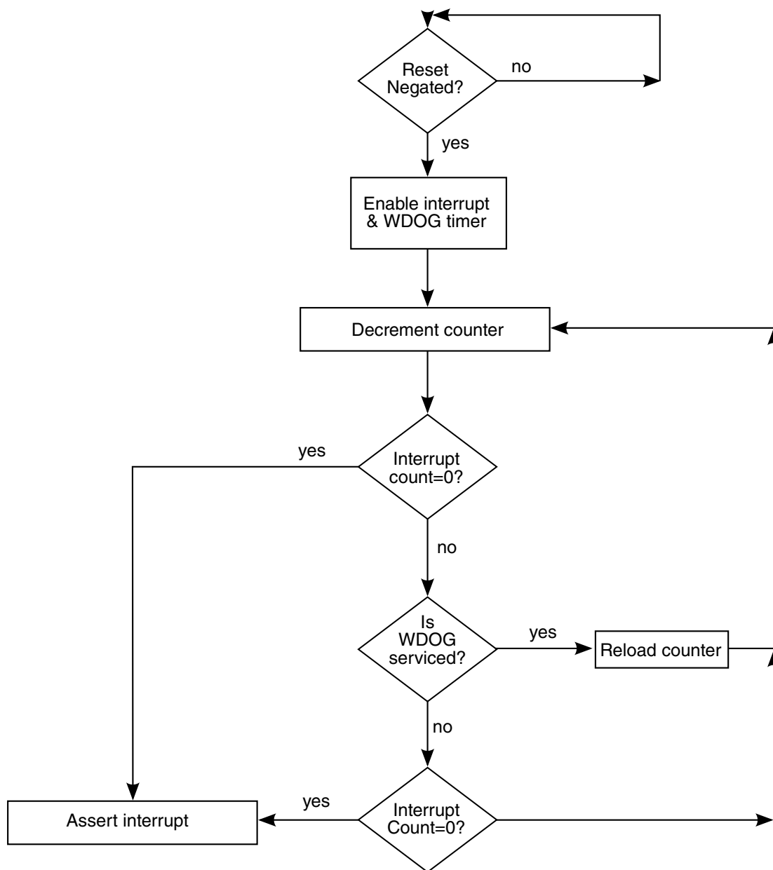
Figure 59-7. Interrupt Generation Flow Diagram
