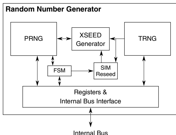
Figure 44-1. RNG block diagram
