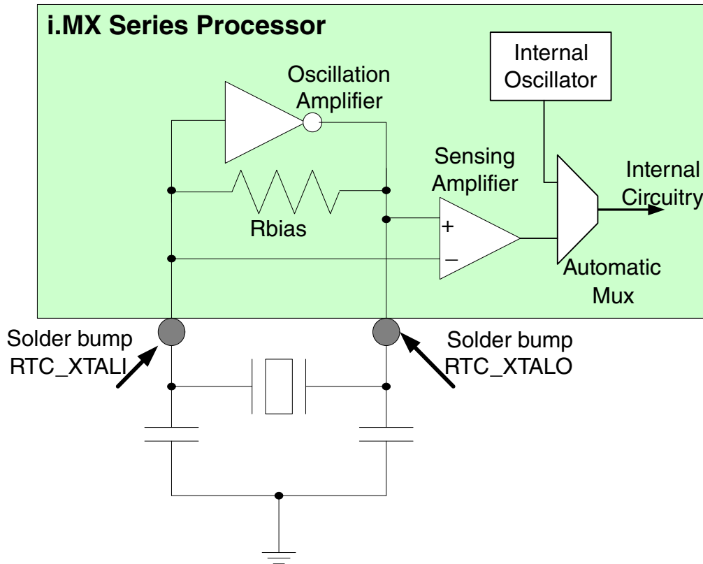
Figure 60-2. Oscillator Configuration (32 kHz)
