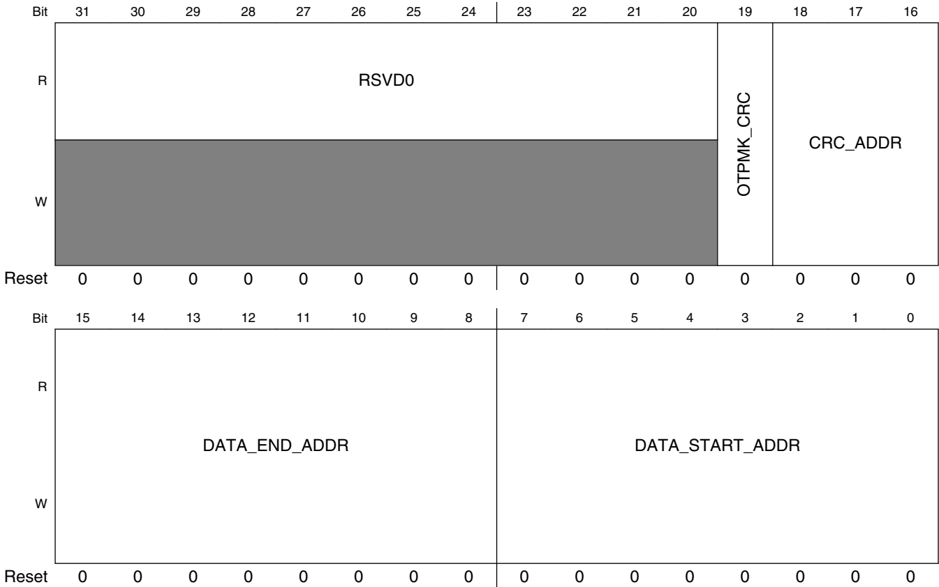
OCOTP_CRC_ADDR field descriptions
