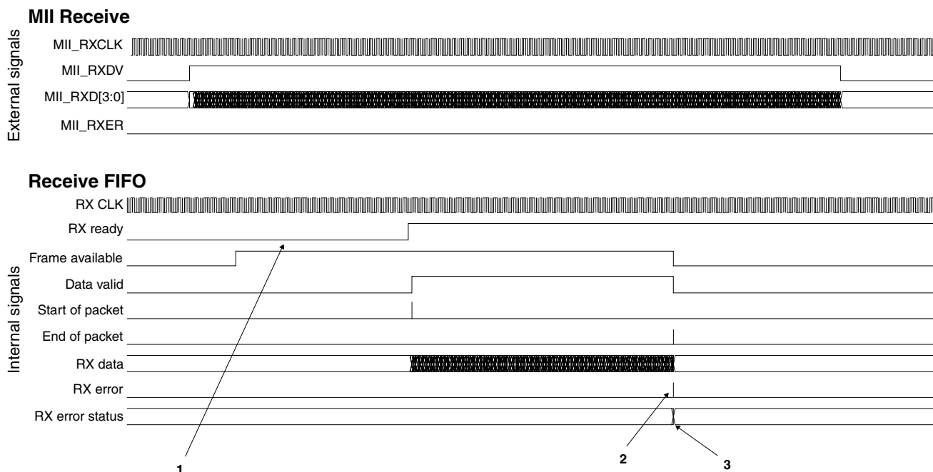
Figure 22-17. Receive FIFO overflow protection
