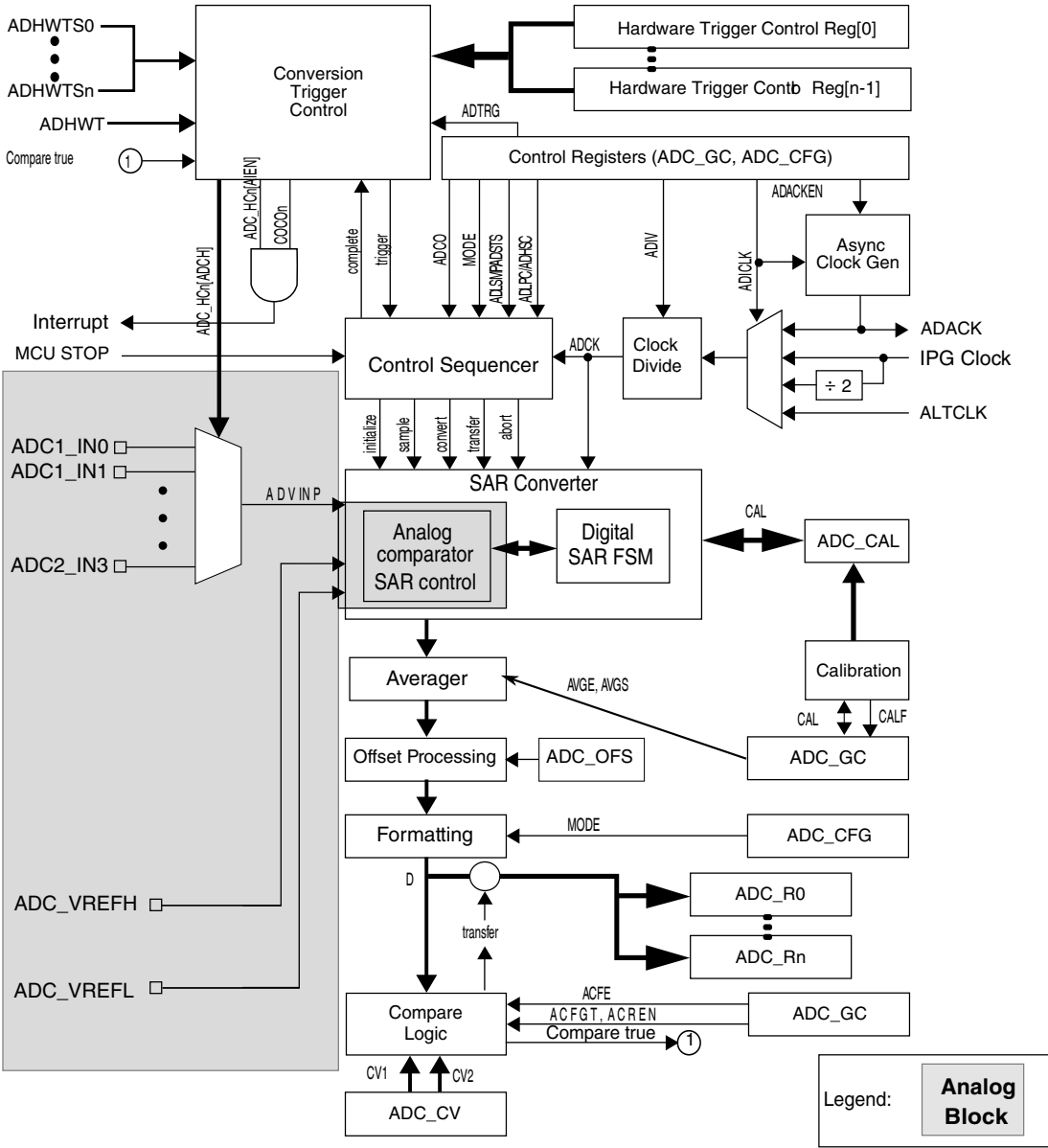
Figure 13-2. ADC block diagram
