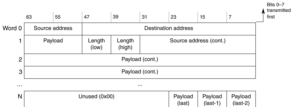
Figure 22-14. Normal Ethernet frame 64-bit mapping example
