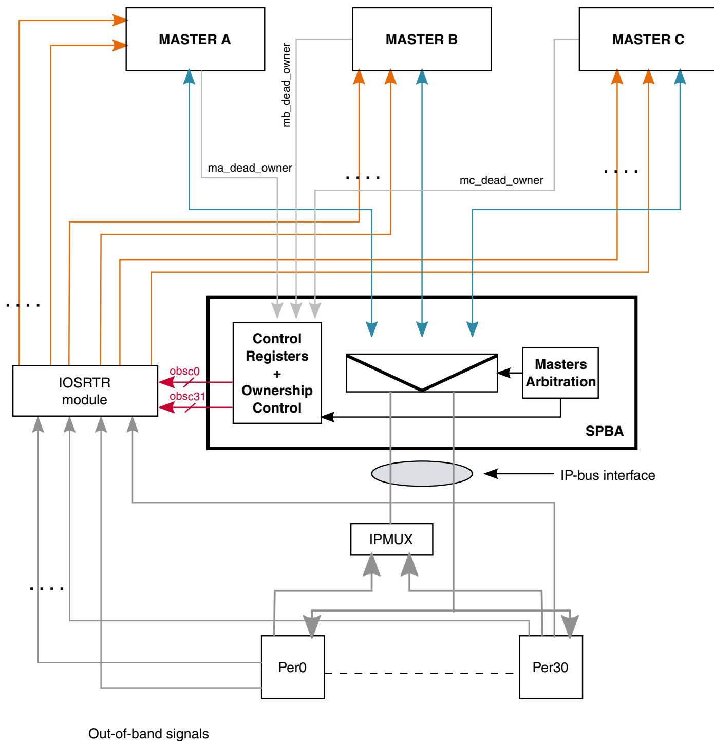
Figure 49-1. SPBA Block Diagram
