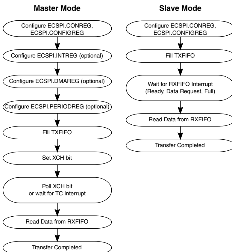
Figure 20-14. Flowchart of the ECSPI Operation
