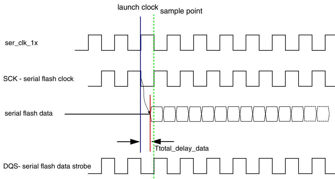
Figure 42-15. Input timing in DDR mode with loopback DQS sampling
