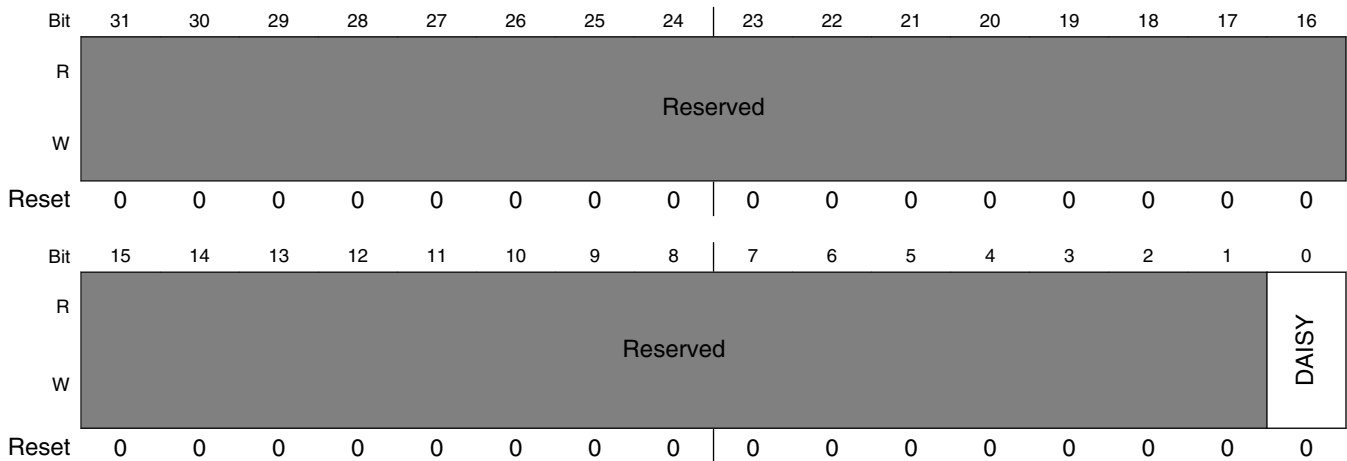
IOMUXC_ECSPi1_SCLK_SELECT_INPUT field descriptions
