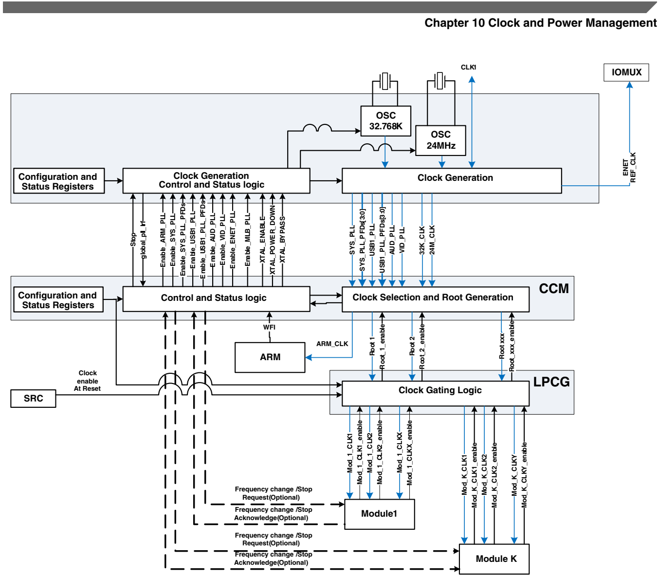
Figure 10-2. Clock Management System
