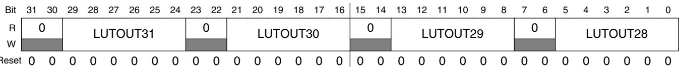
PXP_HW_PXP_WFE_B_STG2_5X6_OUT0_7 field descriptions
