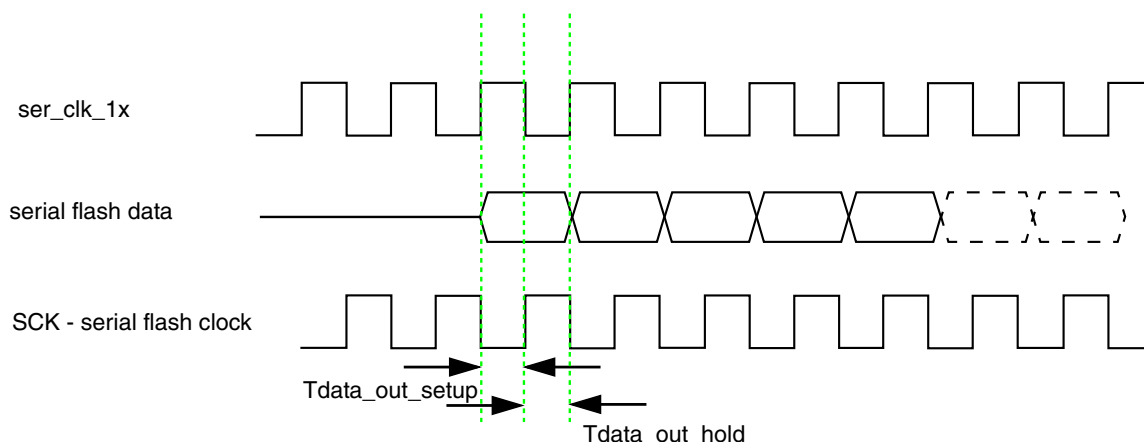
Figure 42-19. Output timing in SDR mode
