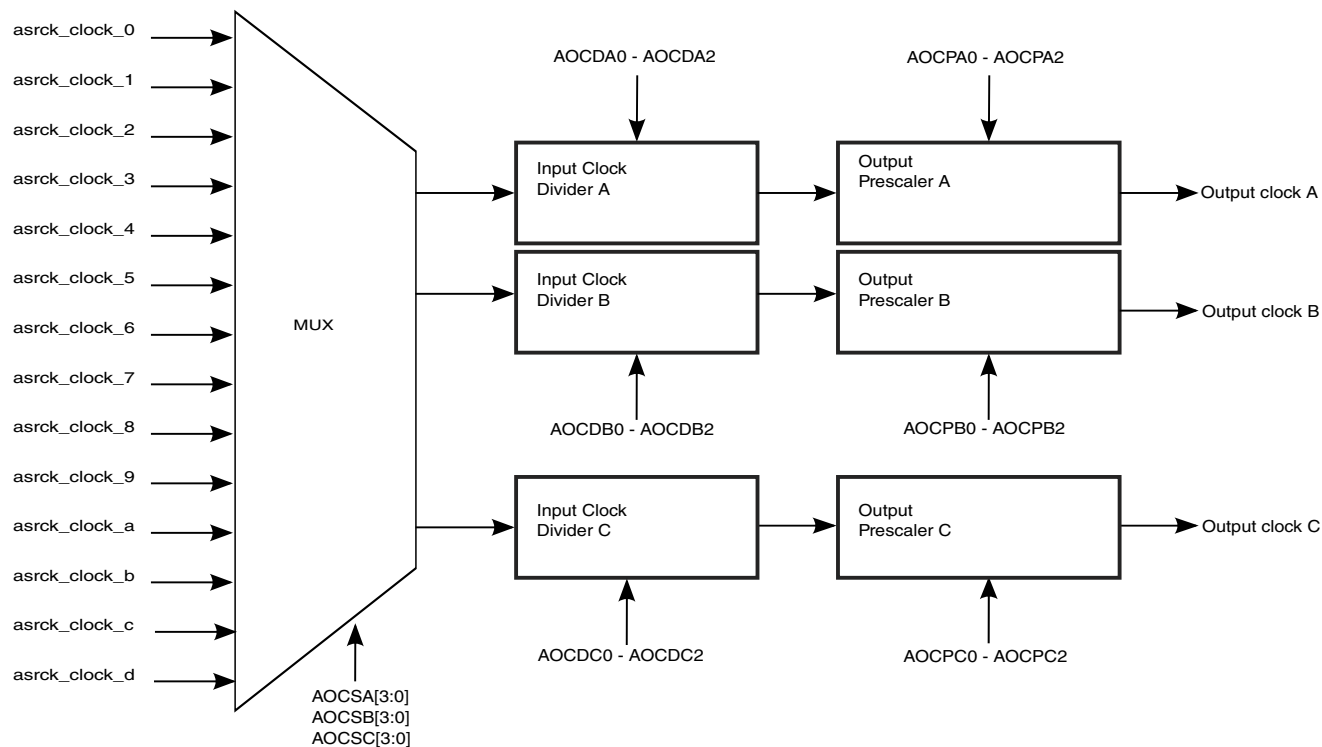
Figure 16-4. Clock Source Selector and Divider
