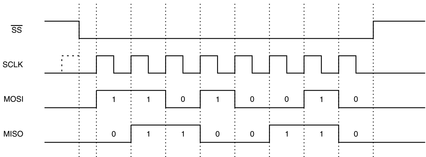
Figure 20-4. Typical SPI Burst (8-bit Transfer)
