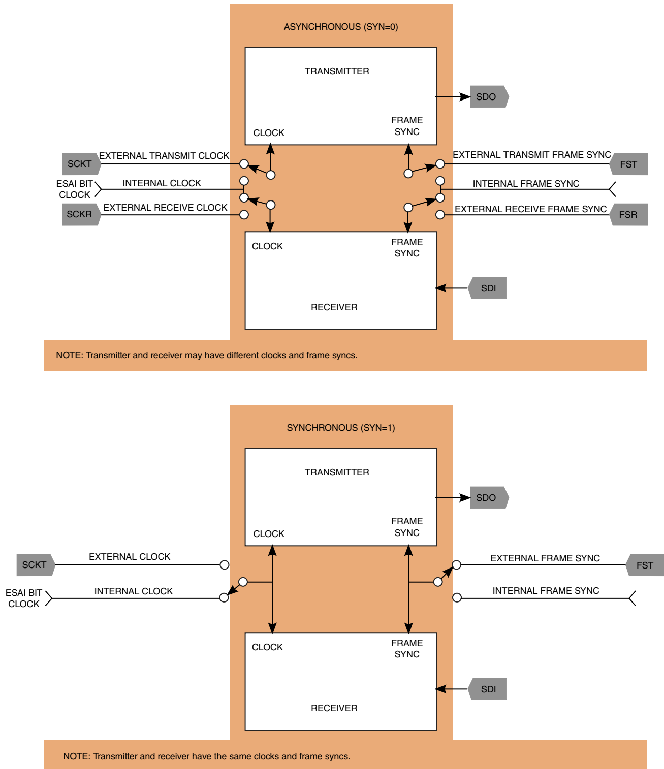
Figure 25-4. SAICR SYN Bit Operation
