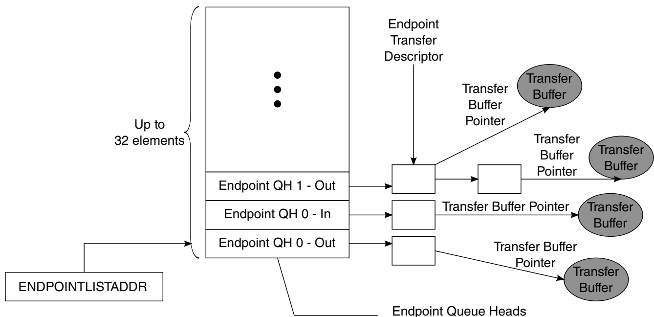
Figure 56-27. EndPoint Queue Head Organization
