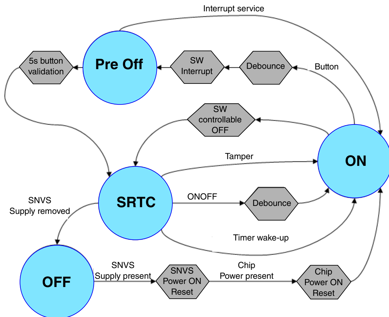
Figure 51-3. Chip on/off state flow diagram
