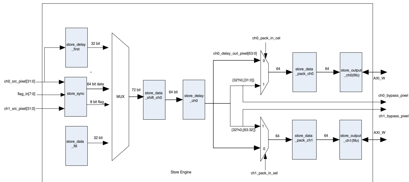
Figure 41-29. High Level Block Diagram
