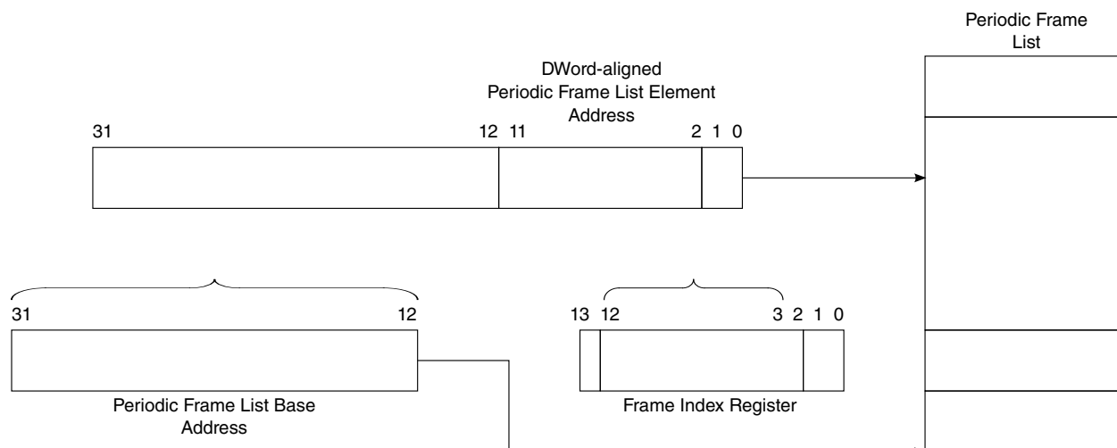
Figure 56-6. Derivation of Pointer into Frame List Array
