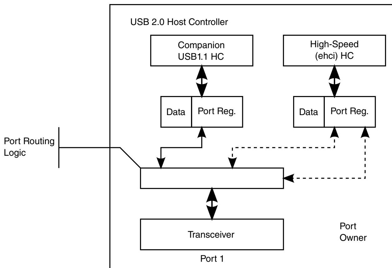
Figure 56-4. Example USB 2.0 Host Controller Port Routing Block Diagram
