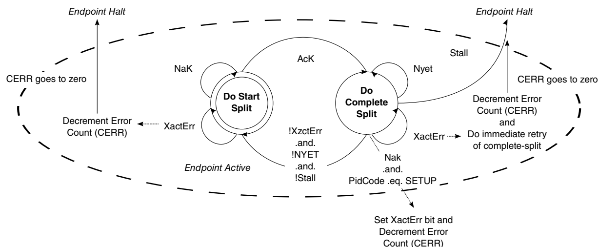
Figure 56-19. Host Controller Asynchronous Schedule Split-Transaction State Machine
