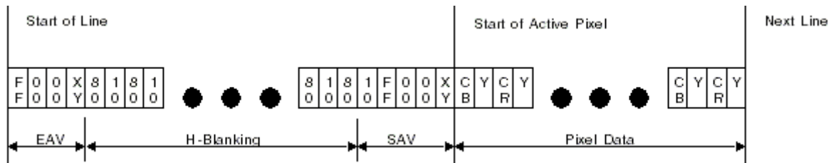
Figure 19-3. CCIR656 General Line Timing
