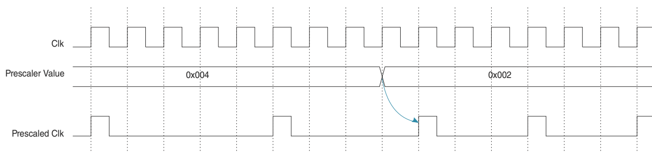
Figure 30-3. Prescaler Value Change Timing Diagram
