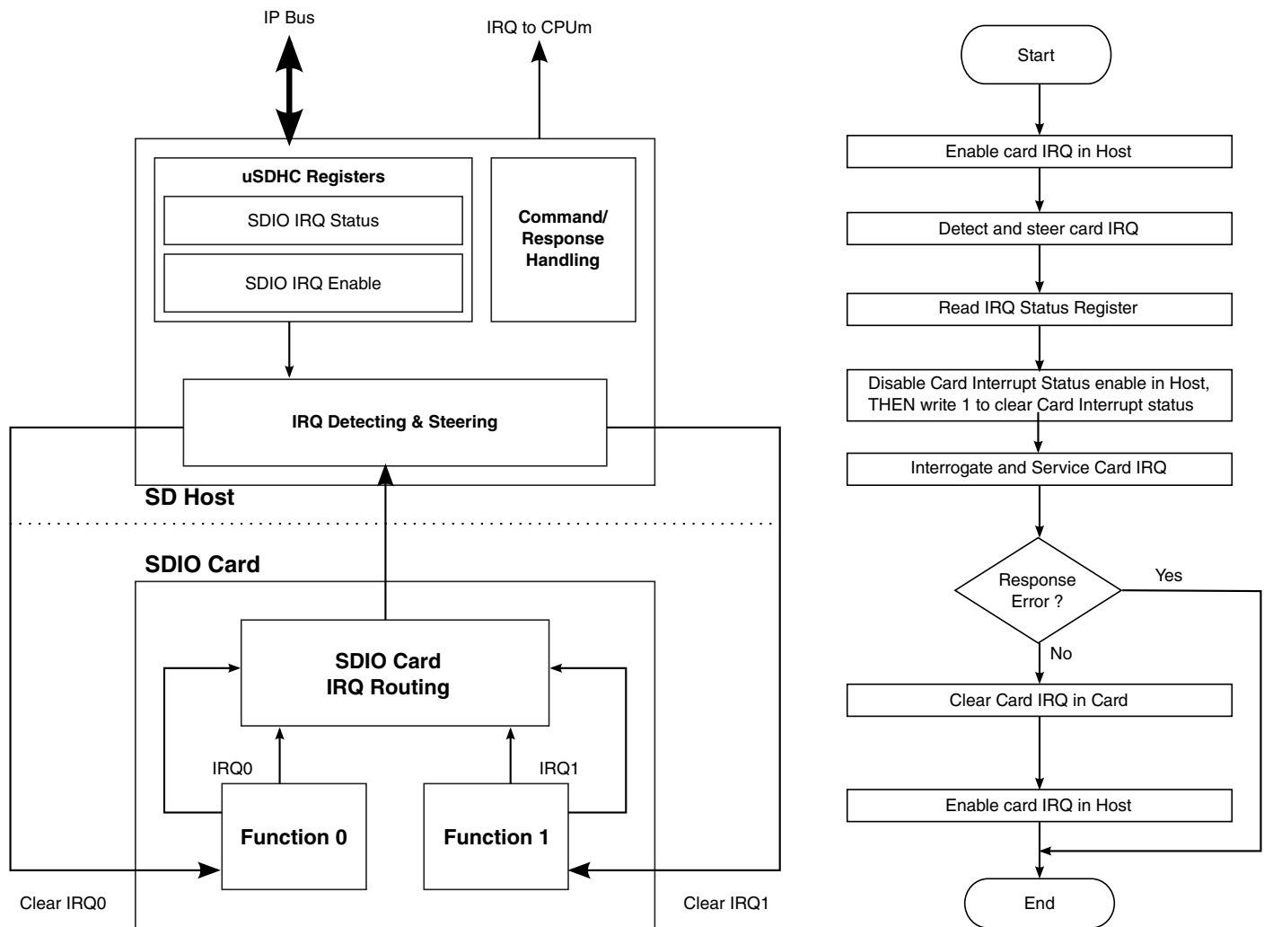
Figure 58-15. Card Interrupt Scheme and Card Interrupt Detection and Handling Procedure
