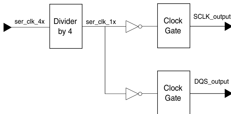
Figure 42-2. Flash Clock Diagram
