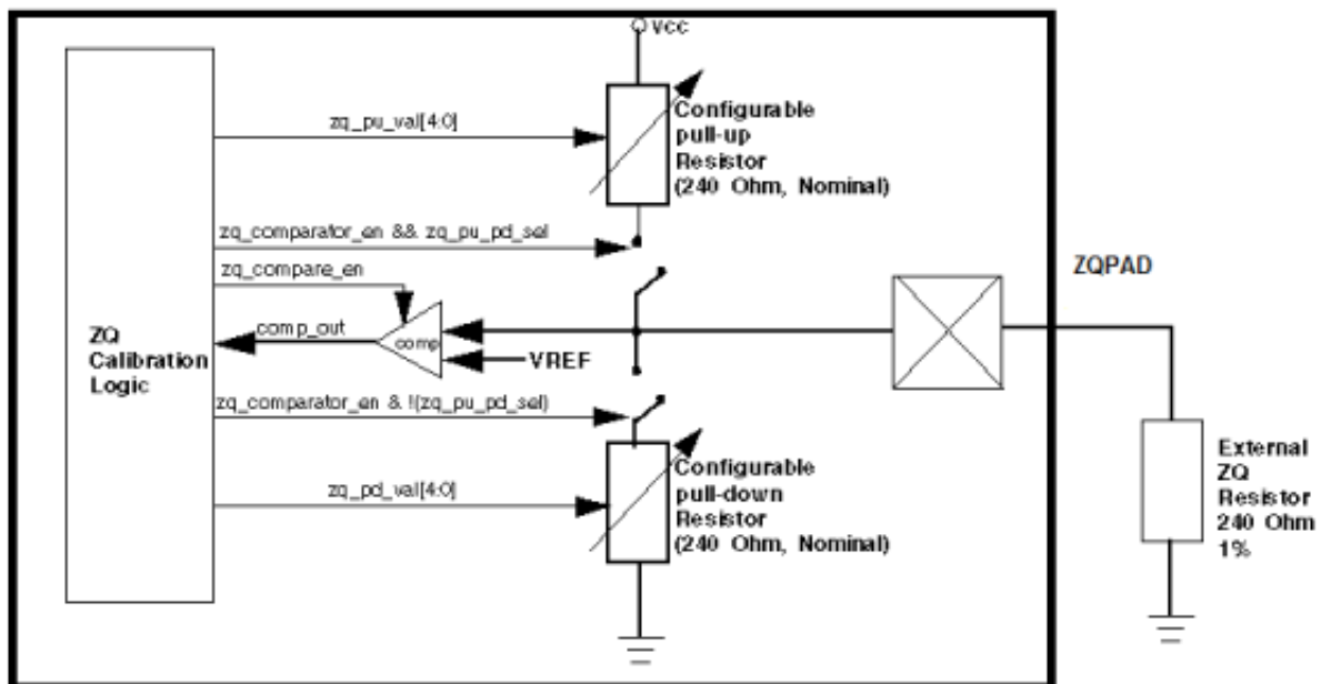
Figure 35-8. MMDC ZQ IF with PAD
