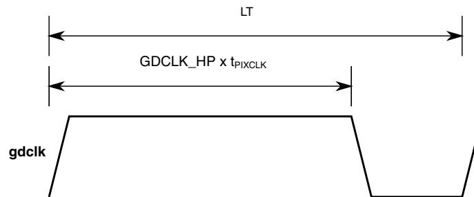
Figure 23-6. GDCLK Duty Cycle
