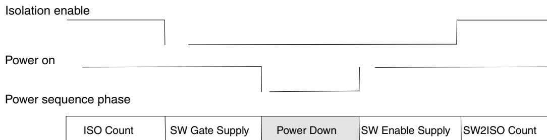
Figure 10-8. SOC_PD isolation and power on switch flow
