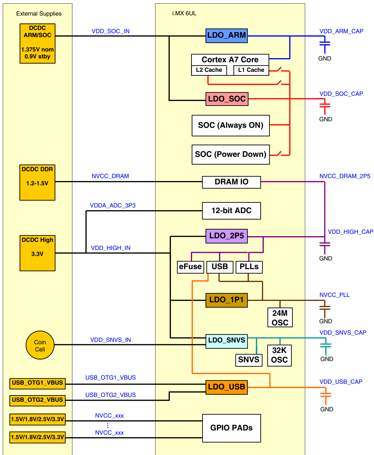
Figure 39-1. Power system overview
