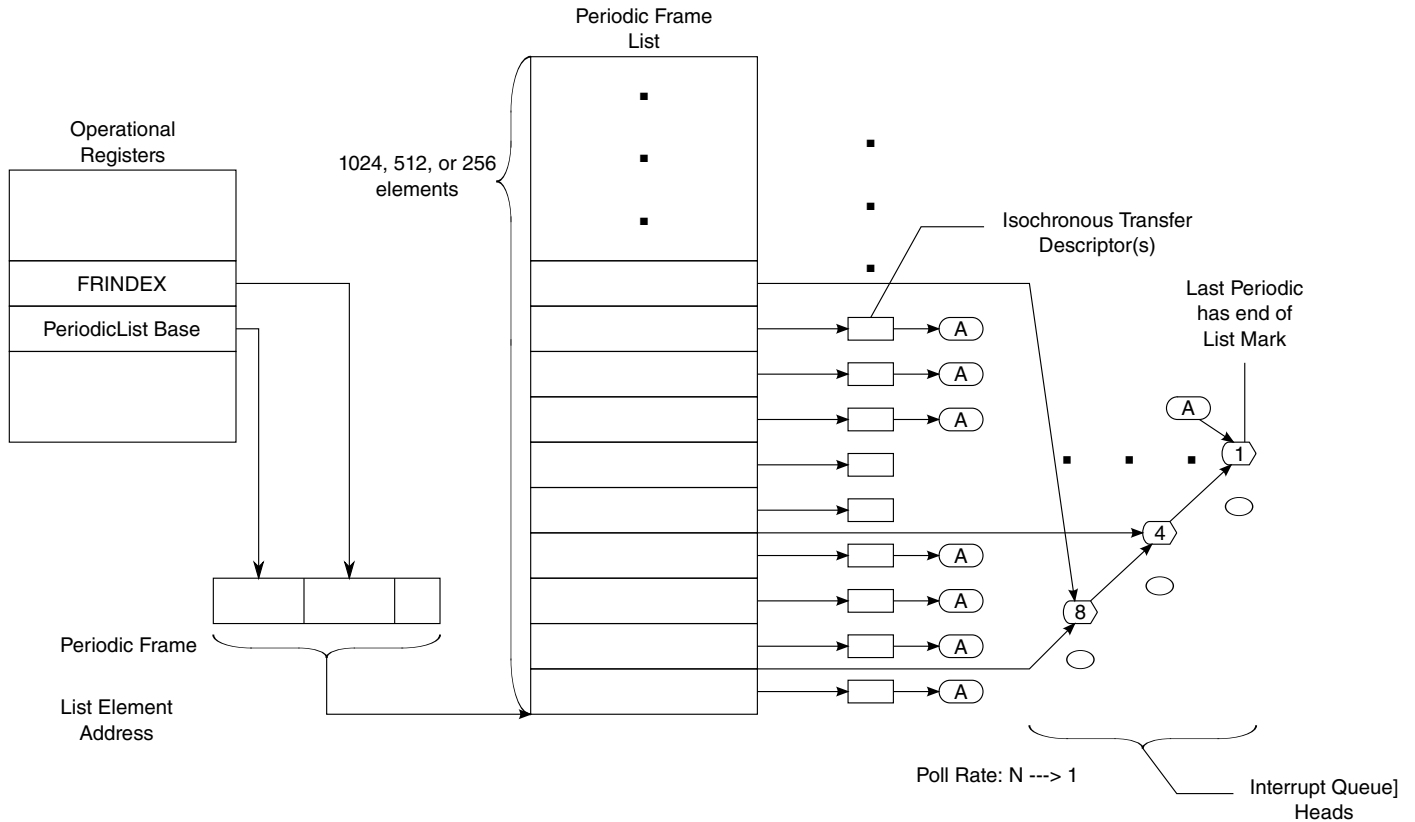
Figure 56-2. Periodic Schedule Organization
