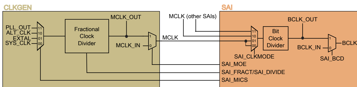
Figure 45-2. SAI master clock generation
