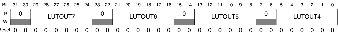
PXP_HW_PXP_WFE_B_STG2_5X6_OUT3_1 field descriptions
