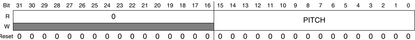
PXP_HW_PXP_OUT_PITCH field descriptions
