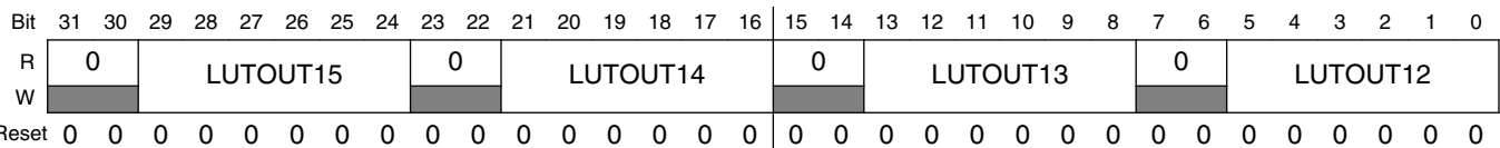
PXP_HW_PXP_WFE_B_STG2_5X6_OUT1_3 field descriptions
