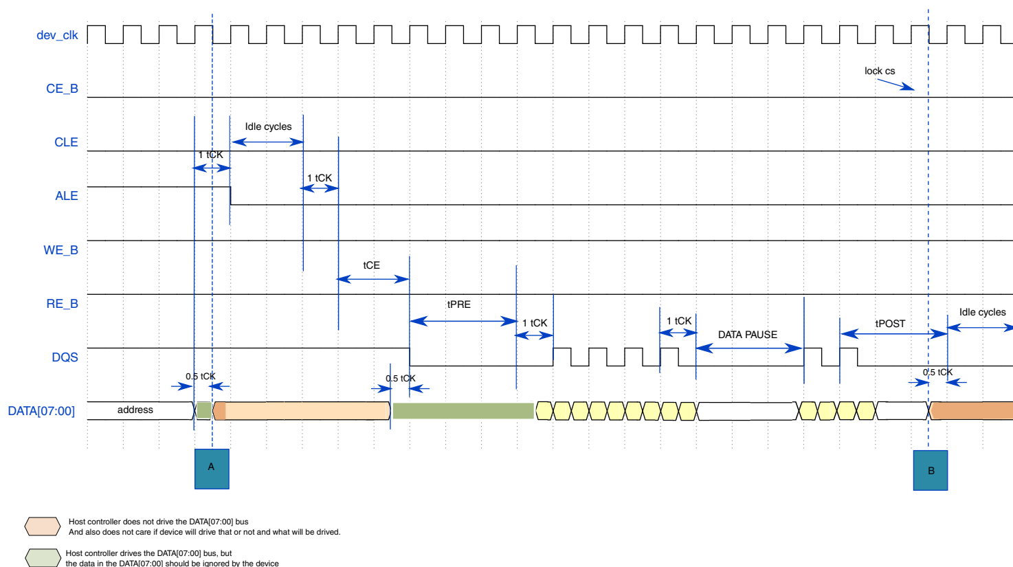
Figure 29-16. Toggle Mode Program Timing Diagram (B)
