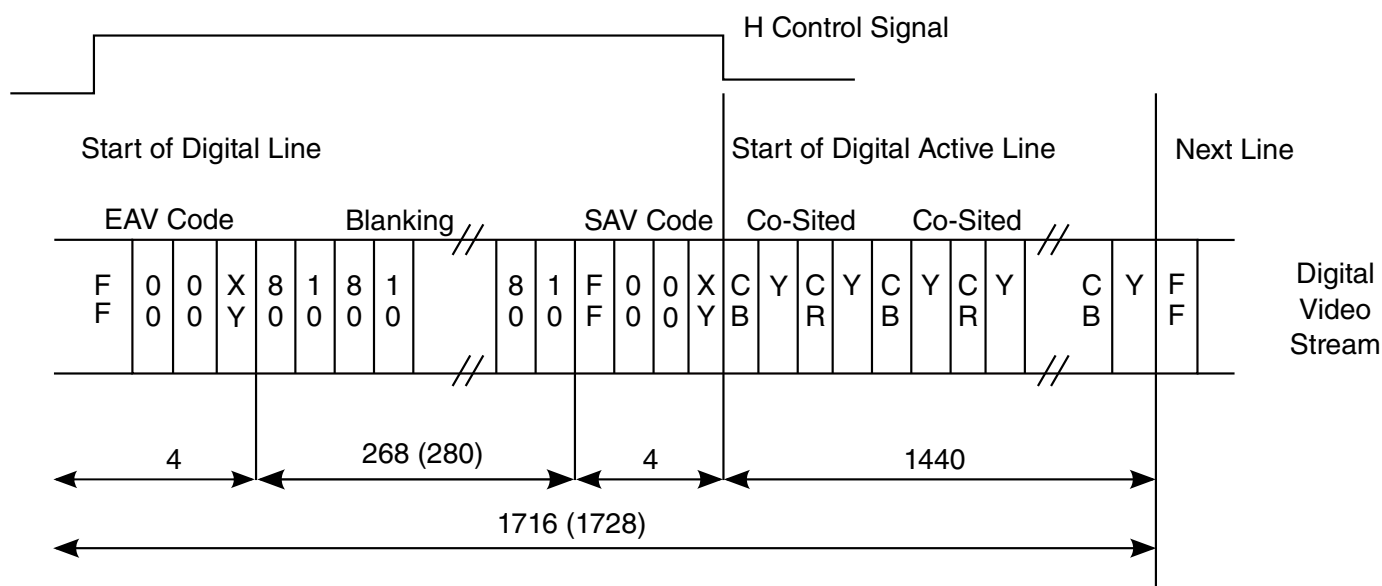
Figure 34-15. Digital Video Interface
