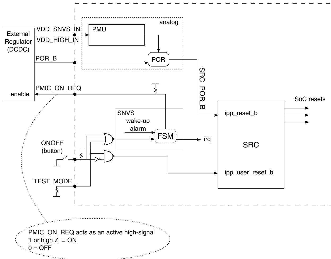
Figure 51-1. Chip reset scheme under PMU control
