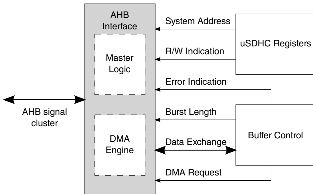
Figure 58-7. DMA AHB Interface Block
