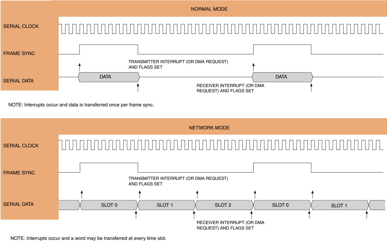
Figure 25-5. Normal and Network Operation
