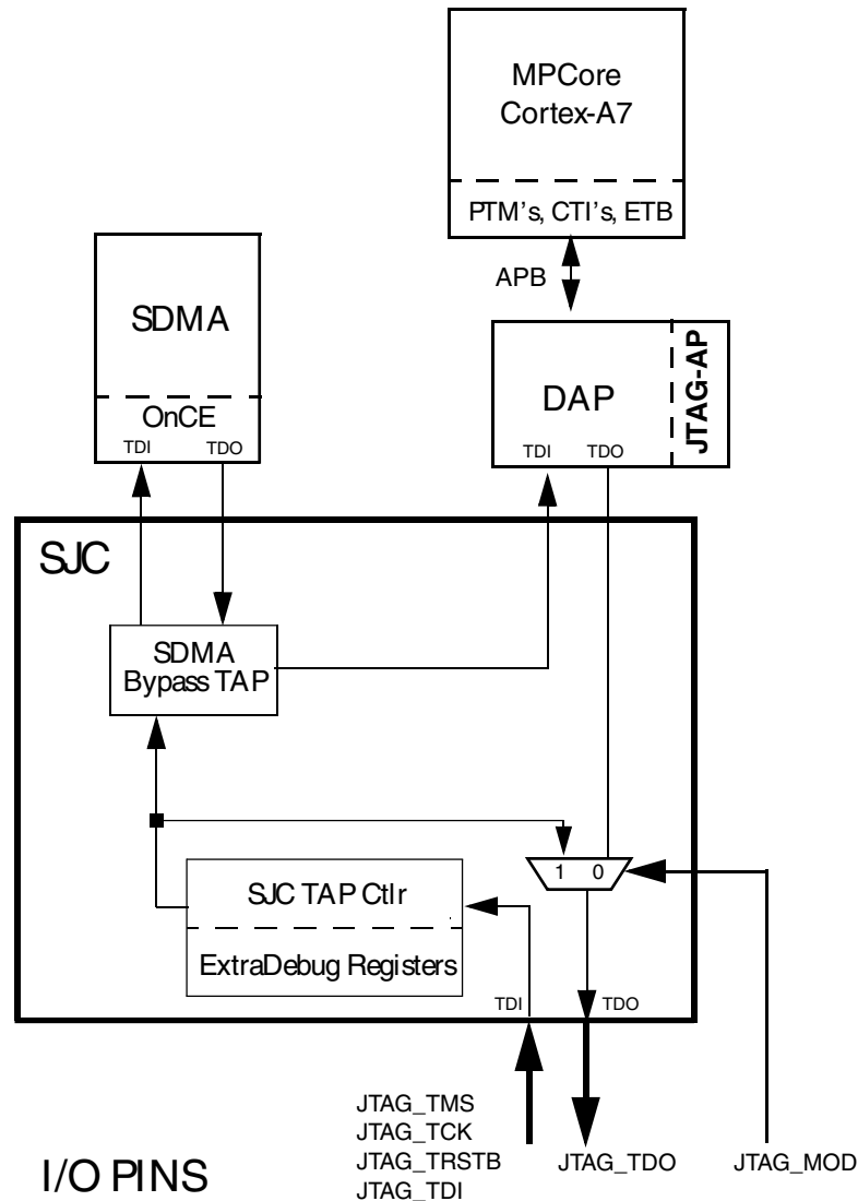
Figure 47-1. System JTAG Controller (SJC) Block Diagram
