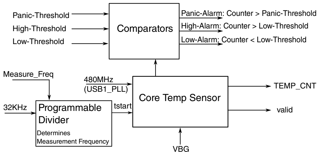
Figure 52-1. High Level Temp Sensor System Diagram
