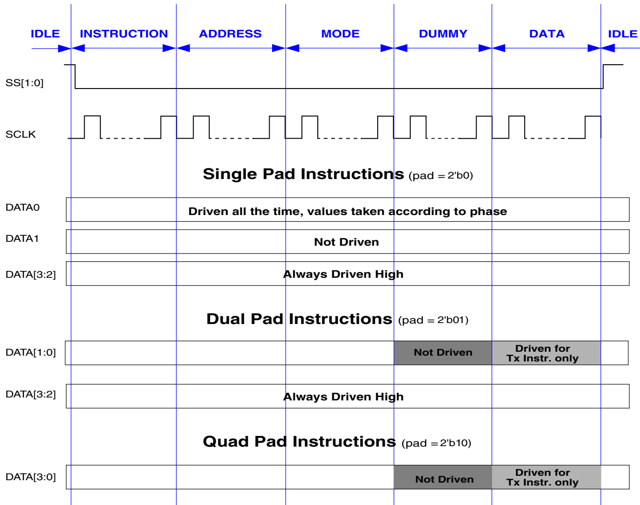
Figure 42-3. Serial Flash Access Scheme
