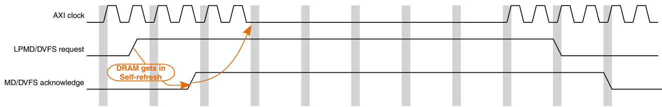
Figure 35-4. LPMD/DVFS Hardware/Software Handshaking
