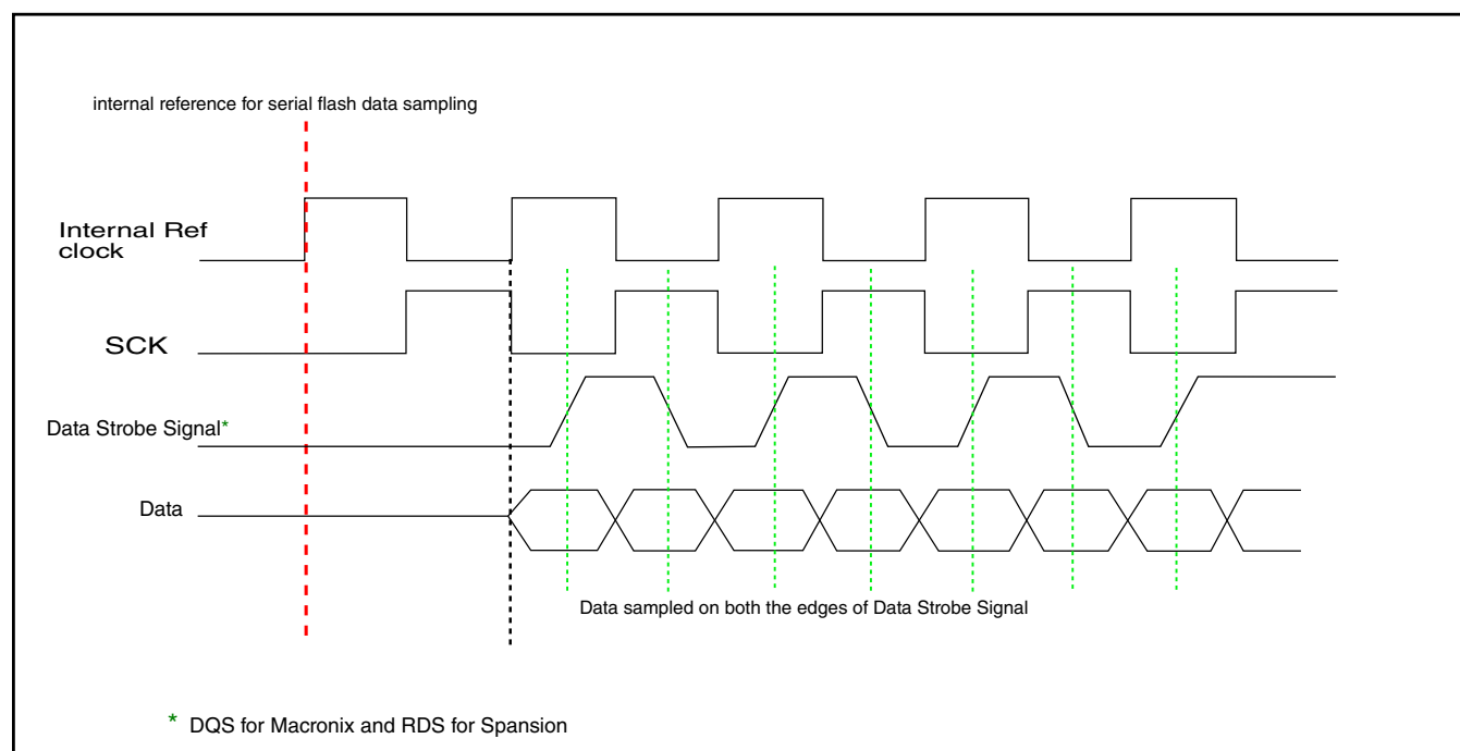
Figure 42-18. Data strobe signal functionality
