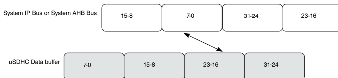
Figure 58-5. Data Swap between System Bus and uSDHC Data Buffer in Half Word Big Endian Mode
