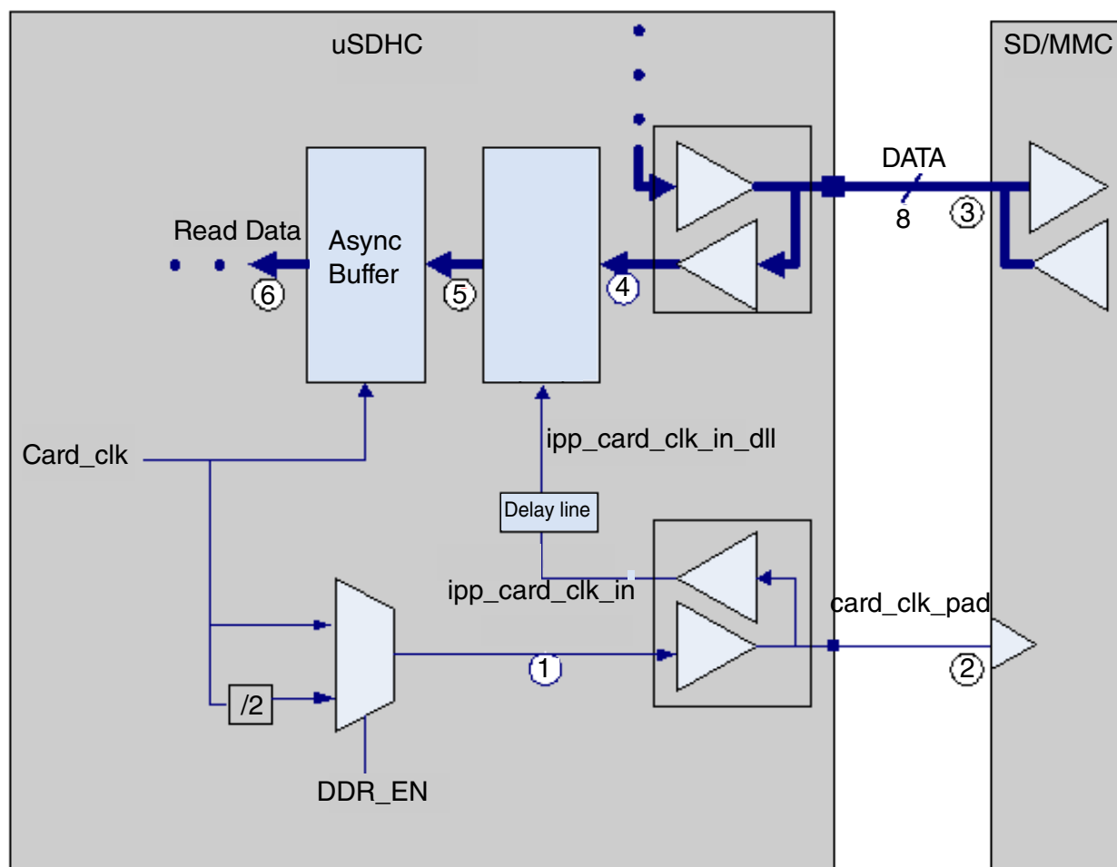
Figure 58-20. DLL(Delay Line) in Read Path
