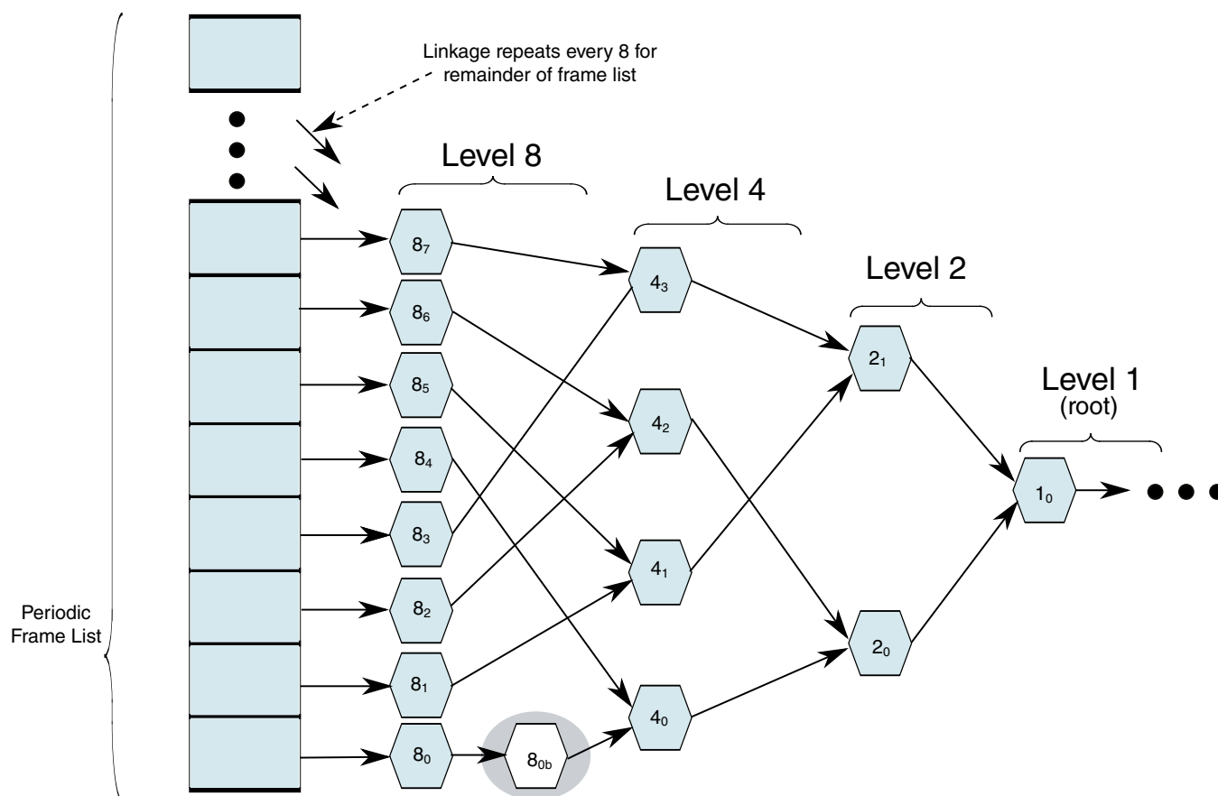
Figure 56-21. General Structure of EHCI Periodic Schedule Utilizing Interrupt Spreading
