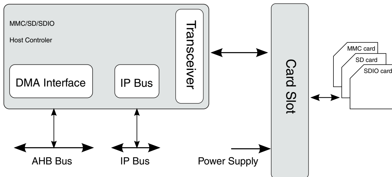
Figure 58-1. System Connection of the uSDHC
