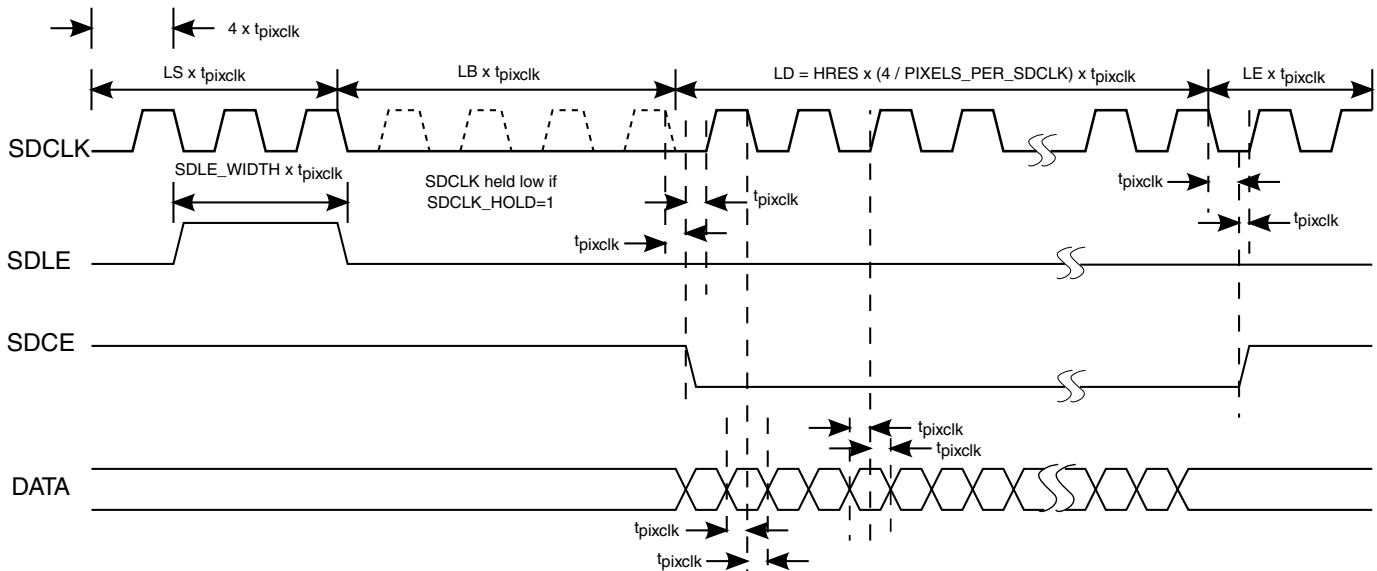
Figure 23-4. Line Timing (DDR_MODE = 1) - RATIO = 4
