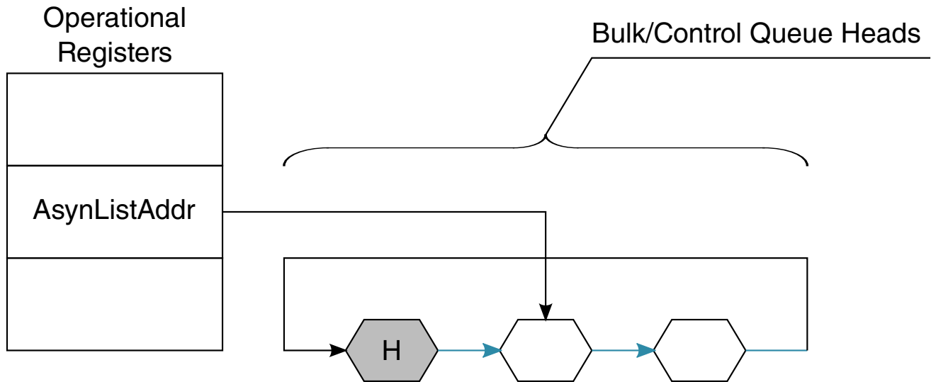
Figure 56-3. Asynchronous Schedule Organization
