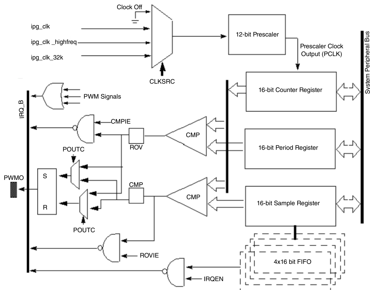
Figure 40-1. Pulse-Width Modulator Block Diagram
