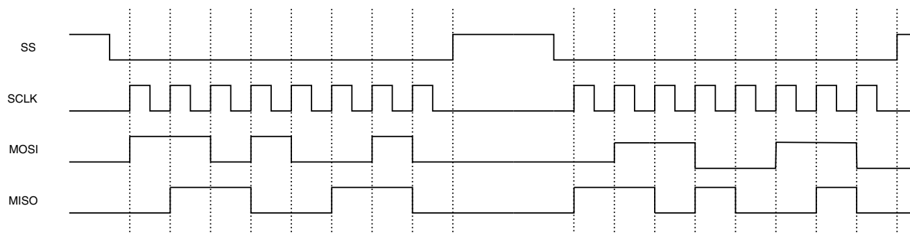
Figure 20-9. SPI Bursts While SS_CTL[3:0] is Set
