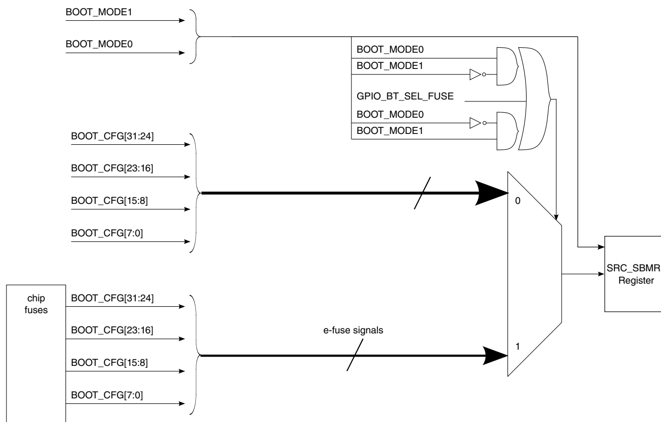
Figure 51-6. Boot mode information
