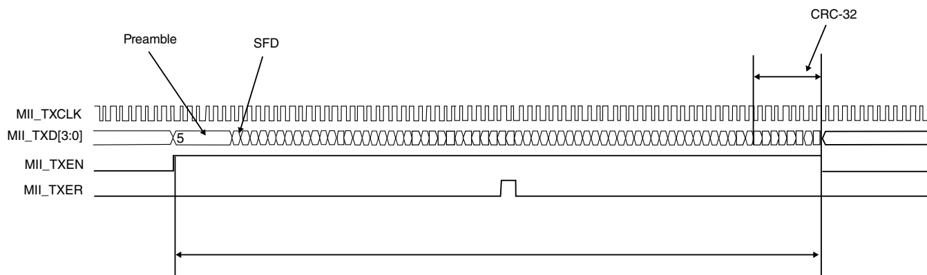
Figure 22-23. MII transmit operation — errored frame
