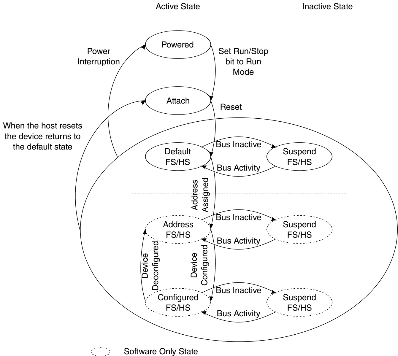
Figure 56-28. Device State Diagram
