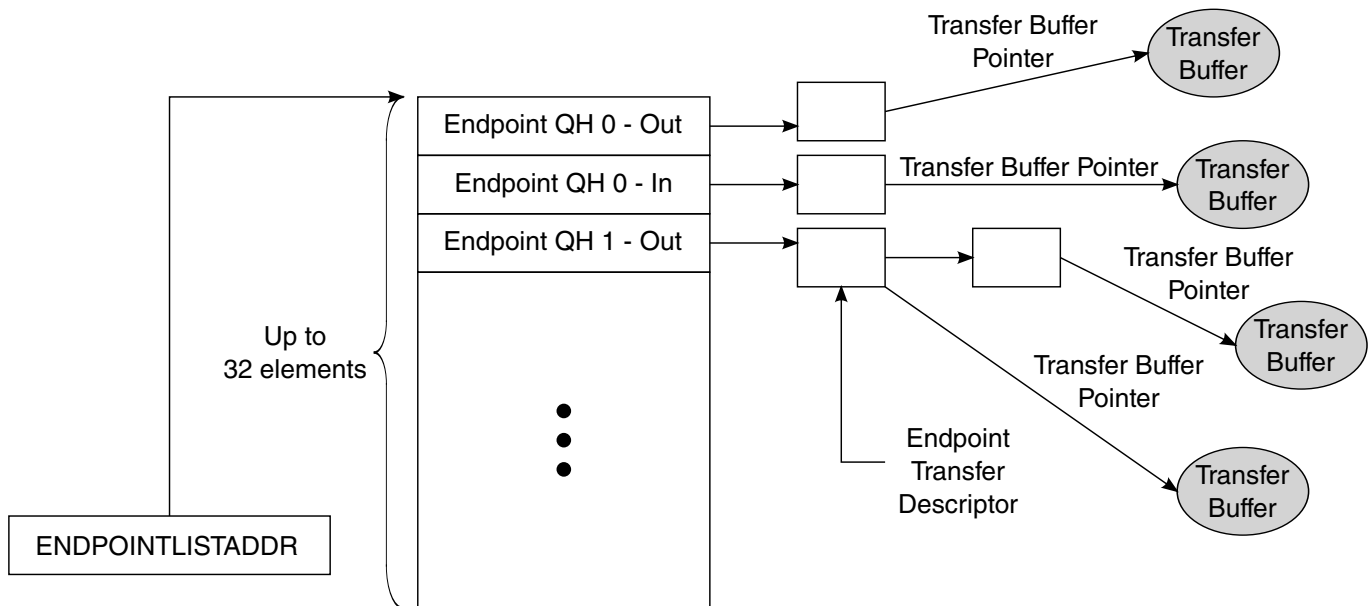
Figure 56-29. End Point Queue Head Diagram
