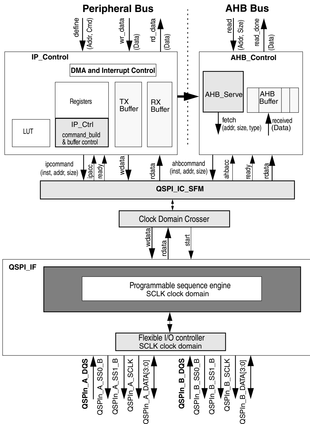
Figure 42-1. QuadSPI Block Diagram
