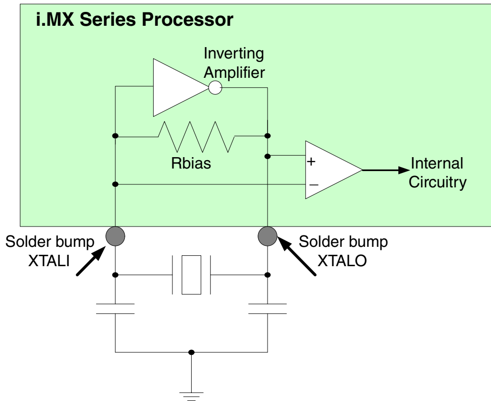
Figure 60-1. Oscillator Configuration (24 MHz)
