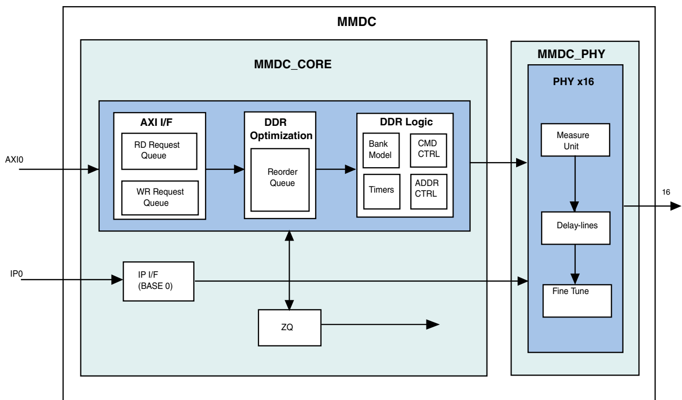
Figure 35-1. MMDC block diagram
