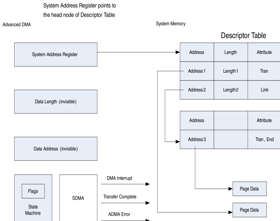
Figure 58-11. Concept and Access Method of ADMA2 Descriptor Table
