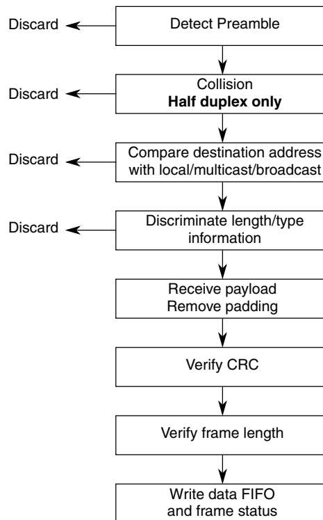
Figure 22-5. MAC receive flow
