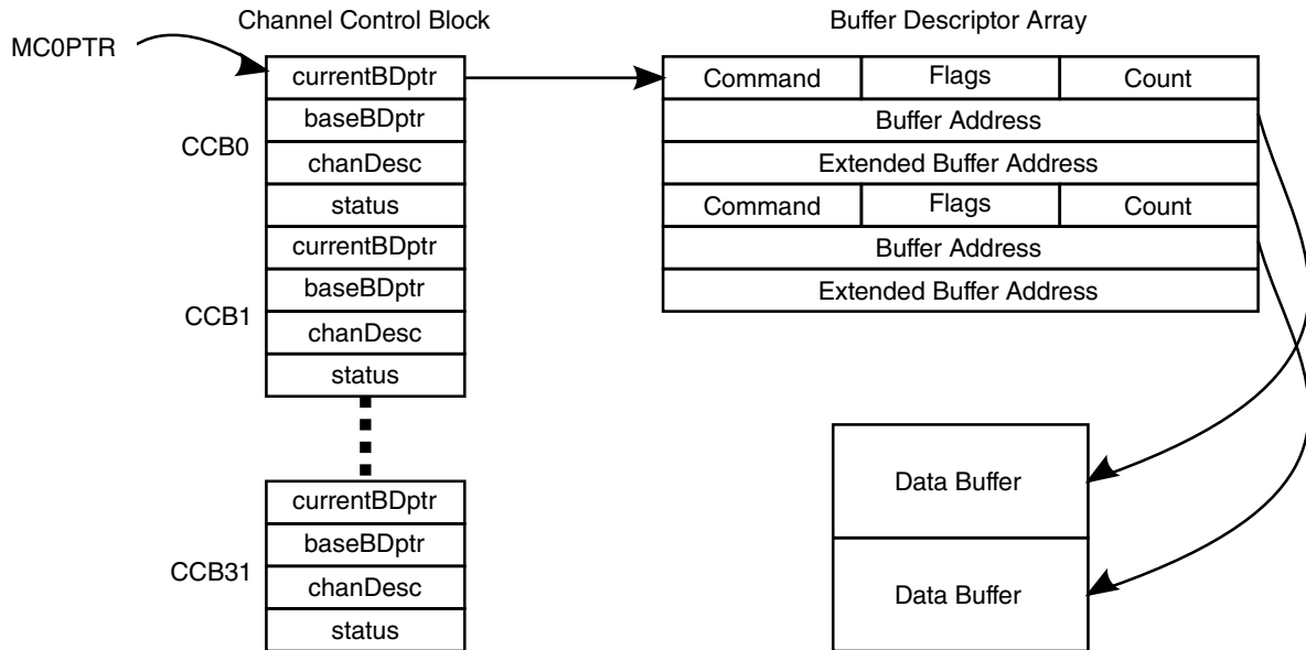
Figure 46-16. Data Structures Layout
