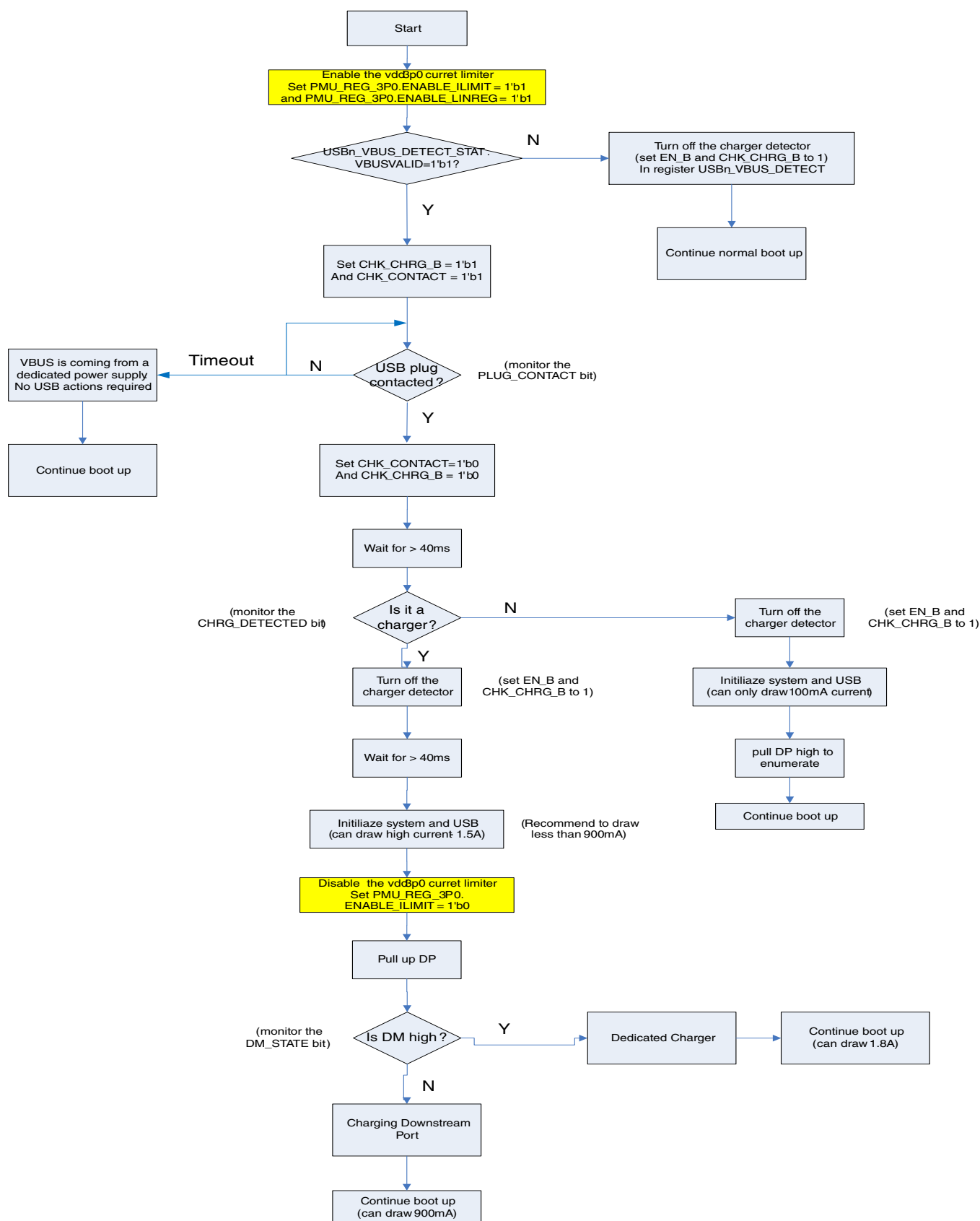
Figure 57-3. USBPHY Charger Detection Software Flow
