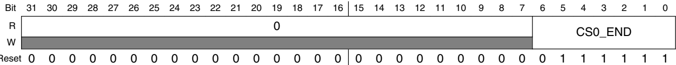
MMDC_MDASP field descriptions
