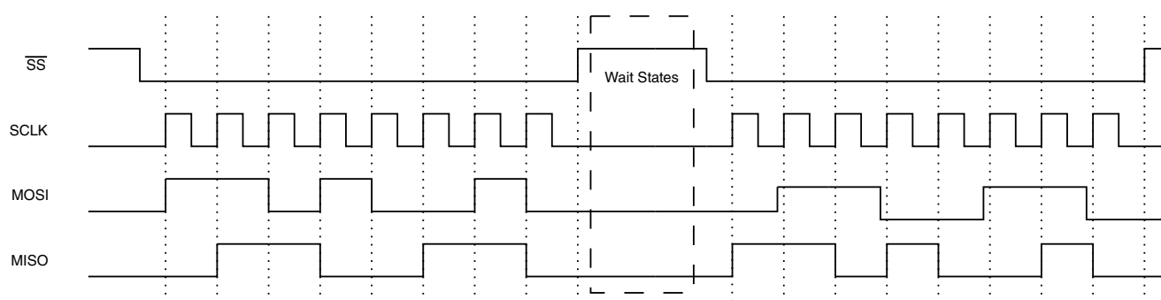
Figure 20-7. SPI Bursts with Wait States
