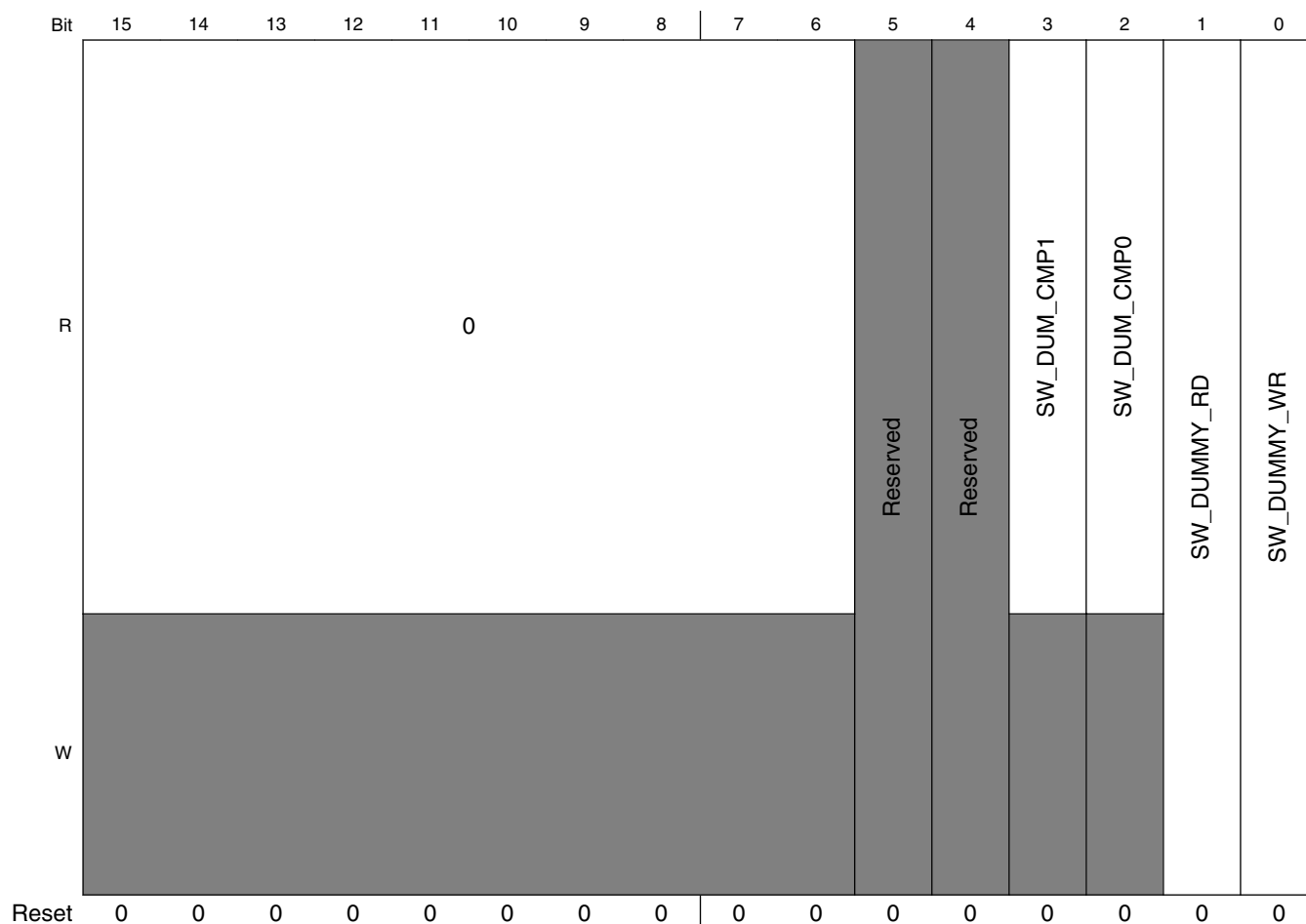
MMDC_MPSWDAR0 field descriptions
