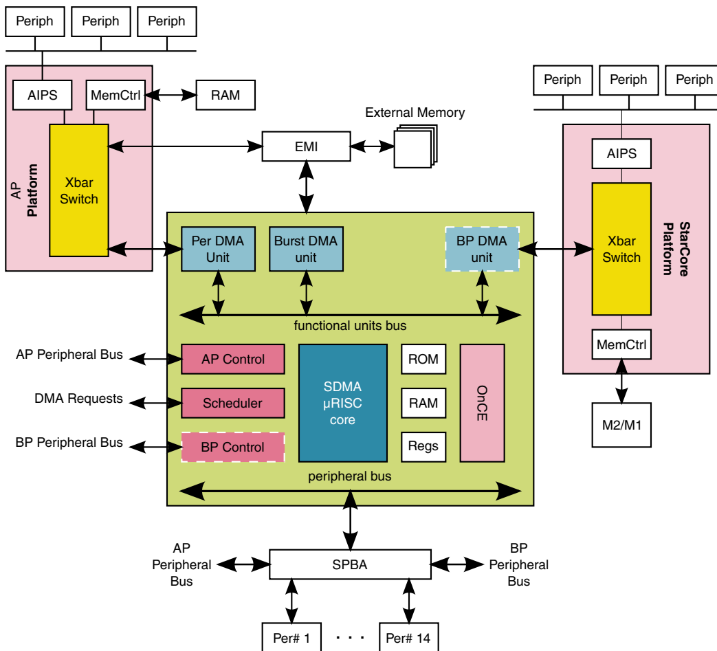
Figure 46-2. SDMA Connections
