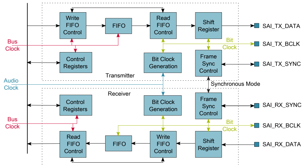
Figure 45-1. I²S/SAI block diagram
