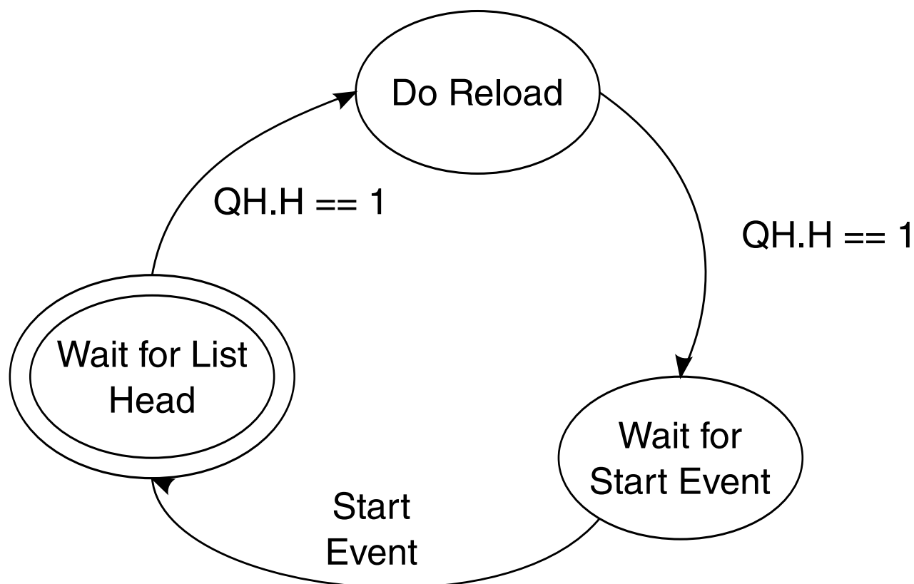
Figure 56-16. Example HC State Machine for Controlling Nak Counter Reloads
