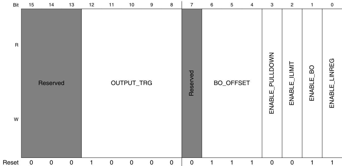
PMU_REG_2P5n field descriptions
