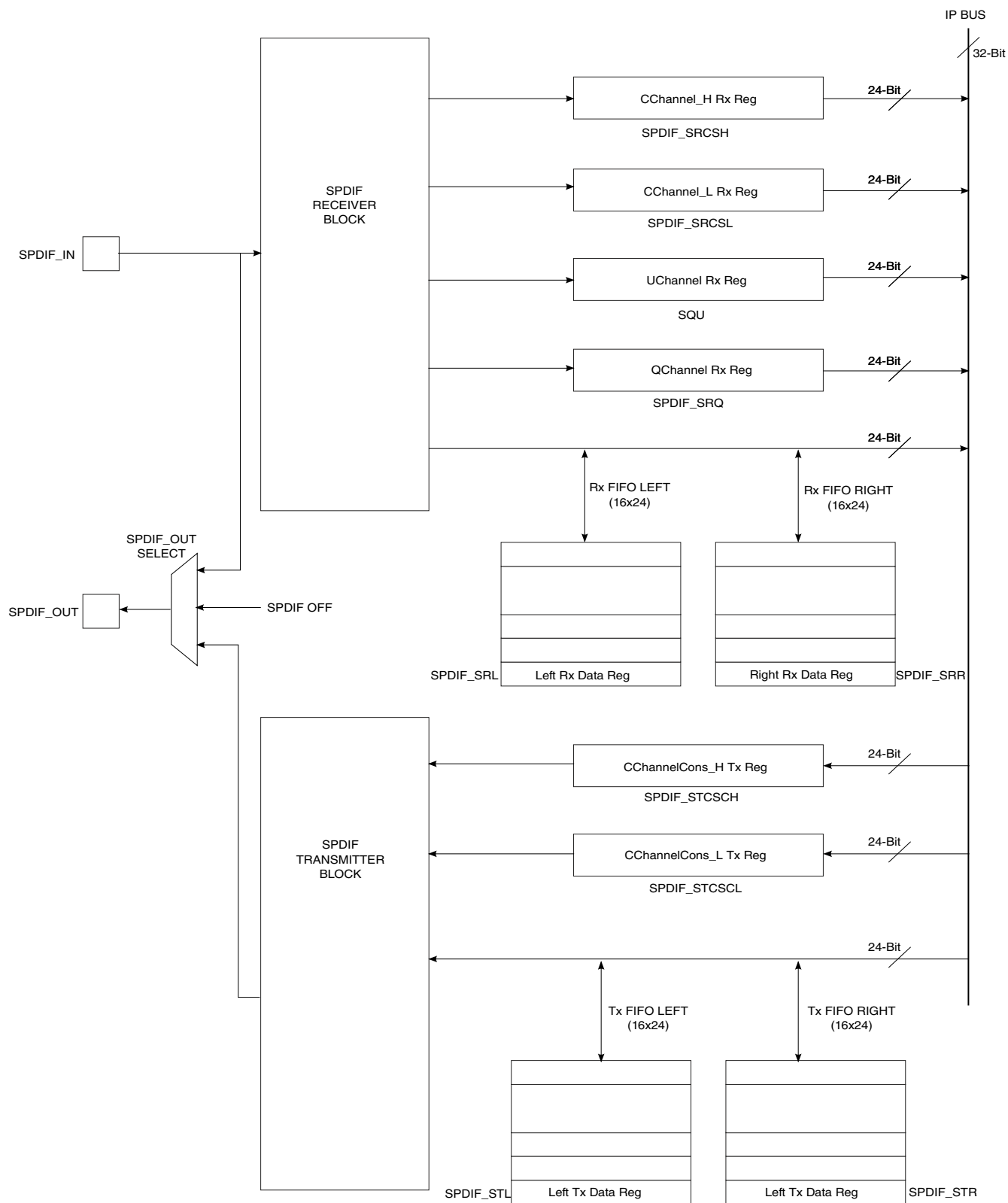
Figure 50-1. SPDIF Transceiver Data Interface Block Diagram
