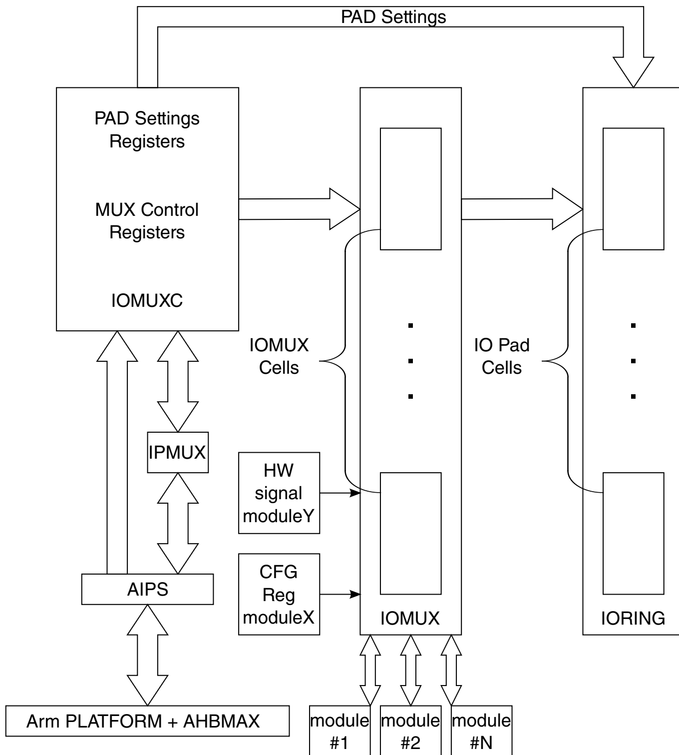
Figure 32-1. IOMUX SoC Level Block Diagram
