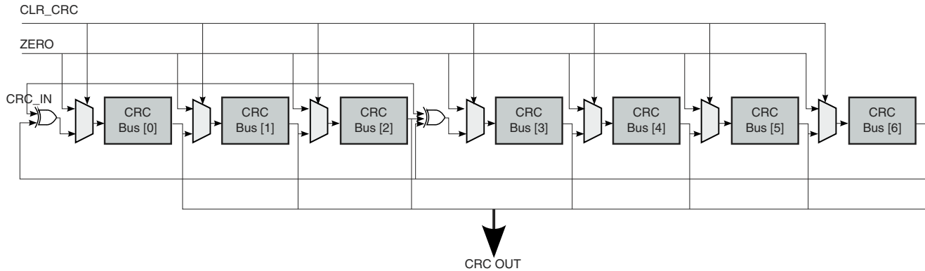
Figure 58-13. Command CRC Shift Register
