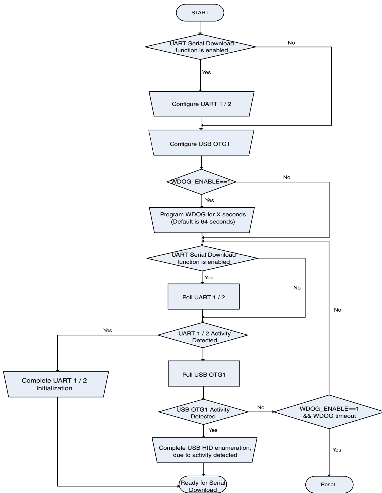
Figure 8-25. Serial Downloader boot flow
