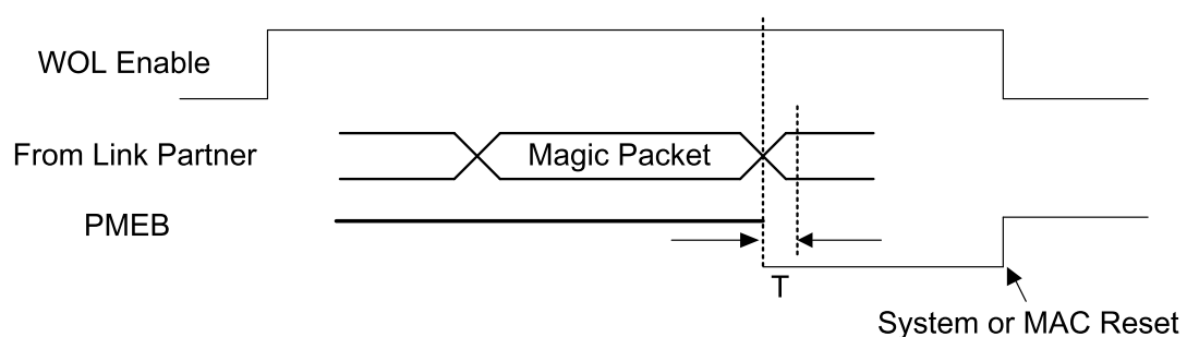
Figure 15. Active Low When Receiving a Magic Packet
