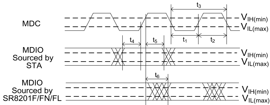
Figure 29. MDC/MDIO Timing
