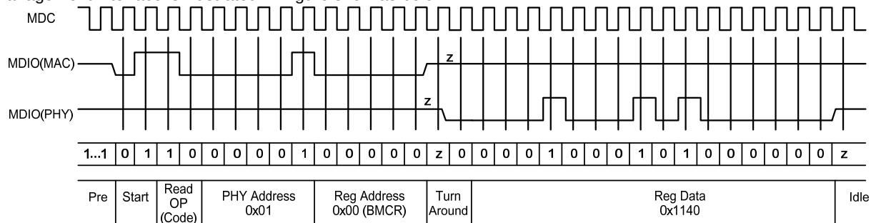
Figure 6. Read Cycle
