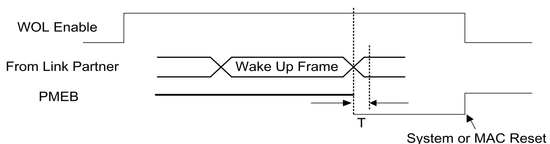
Figure 16. Active Low When Receiving a Wake-Up Frame
