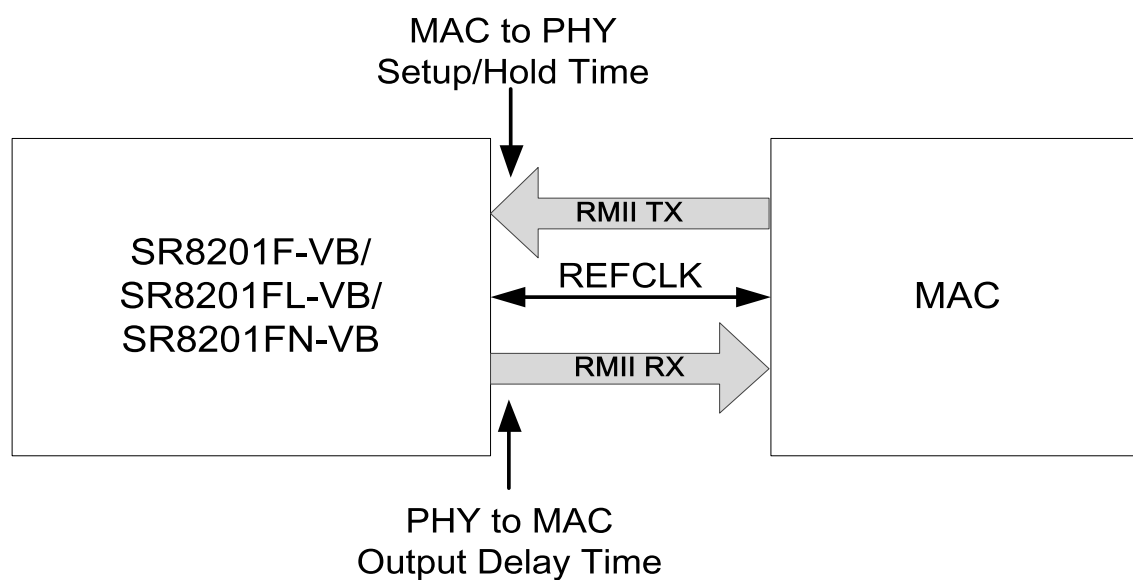
Figure 26. RMII Interface Setup, Hold Time, and Output Delay Time Definitions
